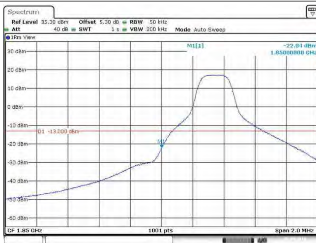
BAND25_5MHz_16QAM_26065_25RB#0
