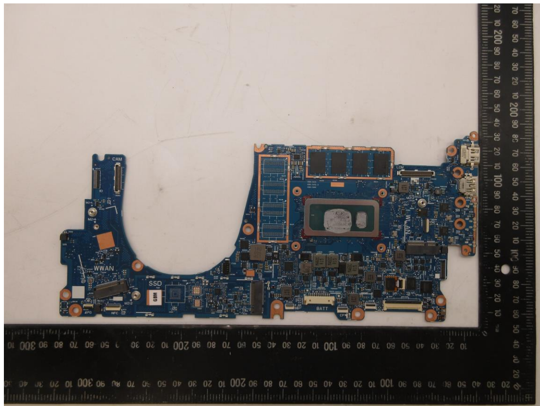
Main board
