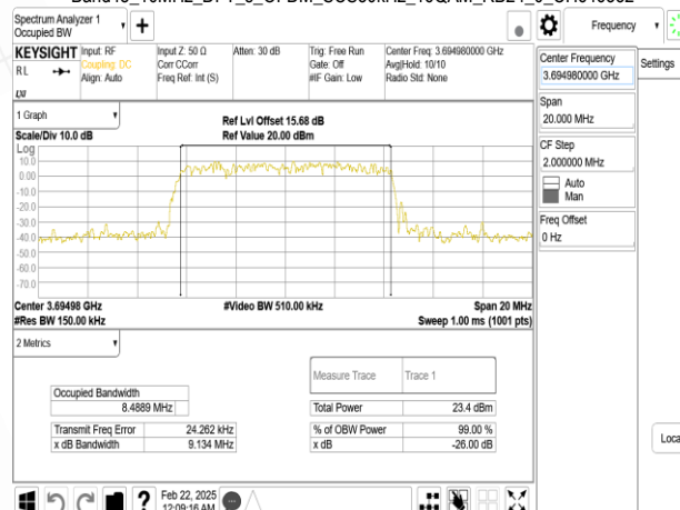
Band48_10MHz_DFT_s_OFDM_SCS30kHz_16QAM_RB24_0_CH646332
