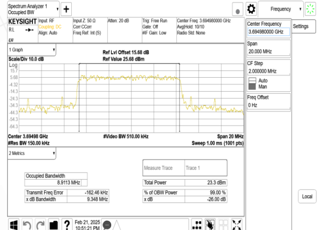
Band48_10MHz_DFT_s_OFDM_SCS15kHz_QPSK_RB50_0_CH646332
