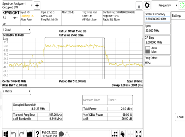
Band48_10MHz_DFT_s_OFDM_SCS15kHz_BPSK_RB50_0_CH646332
