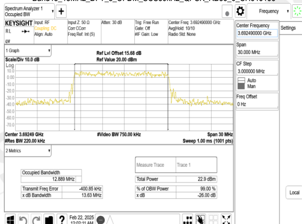
Band48_15MHz_DFT_s_OFDM_SCS30kHz_QPSK_RB36_0_CH646166
