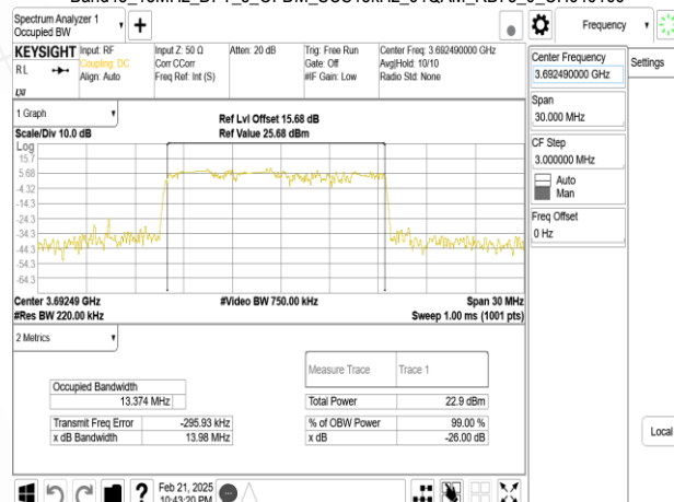
Band48_15MHz_DFT_s_OFDM_SCS15kHz_64QAM_RB75_0_CH646166
