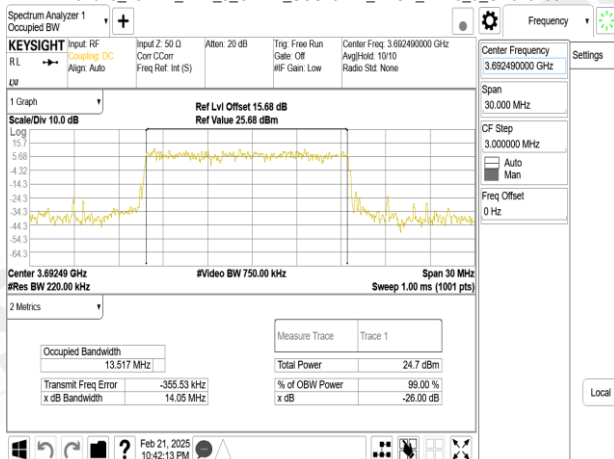
Band48_15MHz_DFT_s_OFDM_SCS15kHz_BPSK_RB75_0_CH646166
