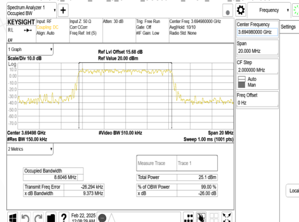
Band48_10MHz_DFT_s_OFDM_SCS30kHz_BPSK_RB24_0_CH646332
