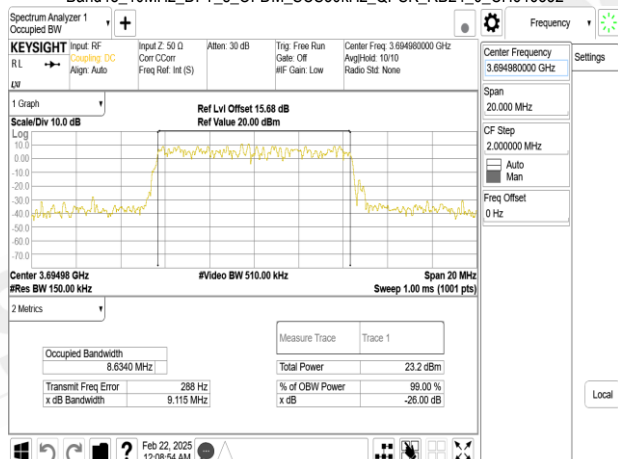
Band48_10MHz_DFT_s_OFDM_SCS30kHz_QPSK_RB24_0_CH646332
