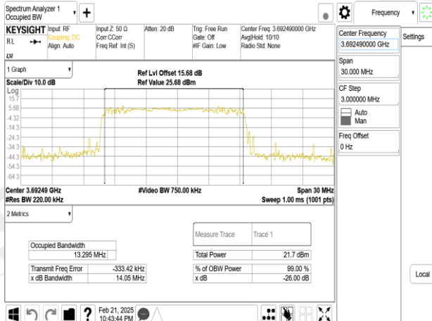
Band48_15MHz_DFT_s_OFDM_SCS15kHz_256QAM_RB75_0_CH646166
