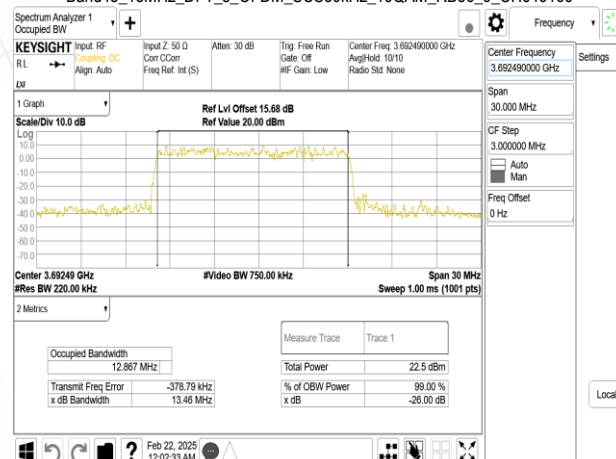
Band48_15MHz_DFT_s_OFDM_SCS30kHz_16QAM_RB36_0_CH646166
