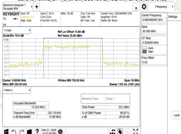
Band48_15MHz_DFT_s_OFDM_SCS15kHz_16QAM_RB75_0_CH646166
