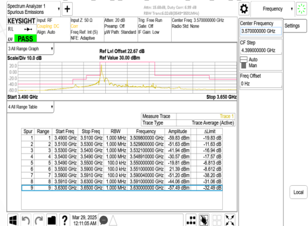
Band48_40MHz_DFT_s_OFDM_SCS30kHz_BPSK_RB1_105_CH638000
