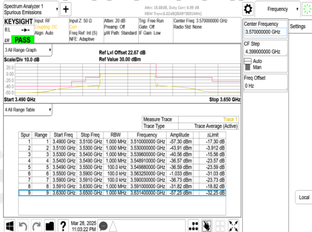
Band48_40MHz_CP_OFDM_SCS15kHz_QPSK_RB1_215_CH645332
