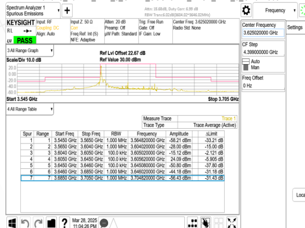
Band48_40MHz_DFT_s_OFDM_SCS15kHz_BPSK_RB1_0_CH641668
