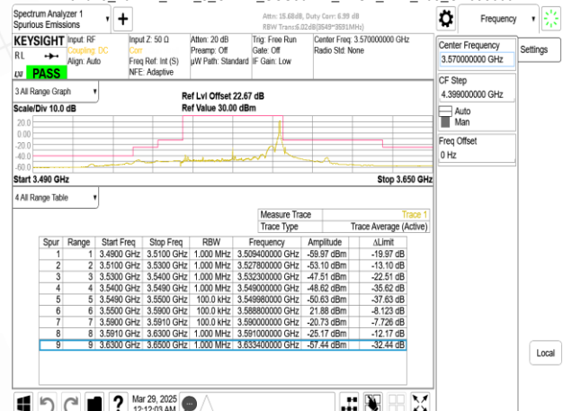
Band48_40MHz_DFT_s_OFDM_SCS30kHz_BPSK_RB1_105_CH638000
