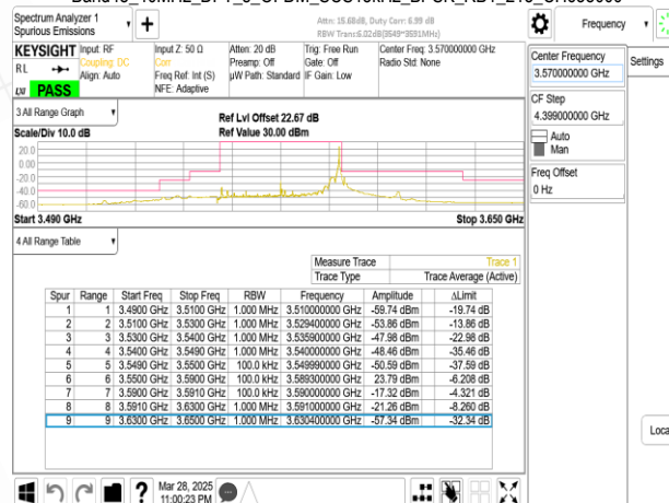
Band48_40MHz_DFT_s_OFDM_SCS15kHz_BPSK_RB216_0_CH638000
