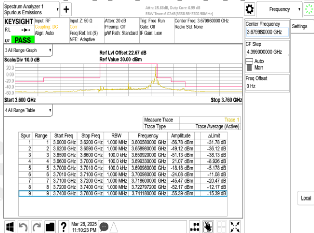
Band48_40MHz_CP_OFDM_SCS15kHz_QPSK_RB216_0_CH645332
