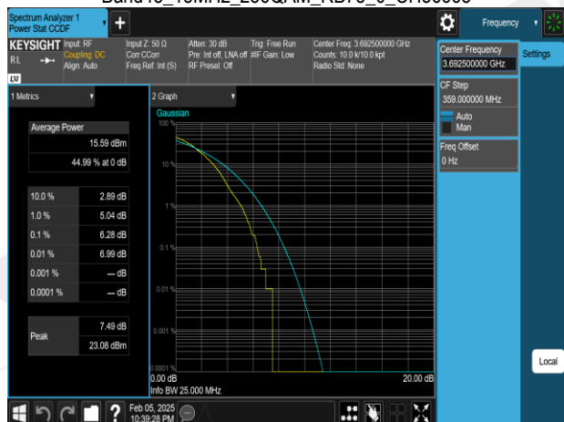
Band48_15MHz_256QAM_RB75_0_CH56665
