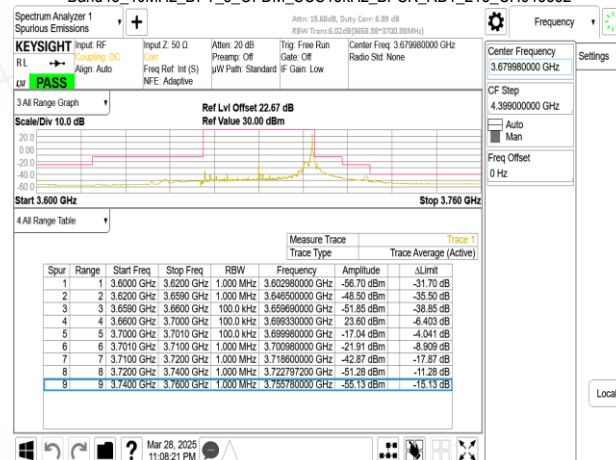
Band48_40MHz_DFT_s_OFDM_SCS15kHz_BPSK_RB216_0_CH645332
