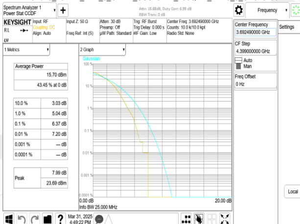
Band48_15MHz_DFT_s_OFDM_SCS15kHz_256QAM_RB75_0_CH646166
