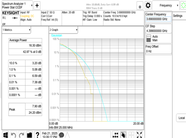
Band48_20MHz_DFT_s_OFDM_SCS15kHz_256QAM_RB100_0_CH646000
