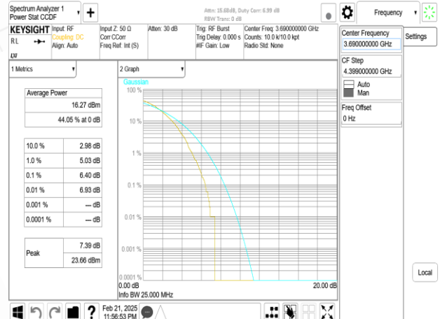
Band48_20MHz_DFT_s_OFDM_SCS30kHz_256QAM_RB50_0_CH646000
