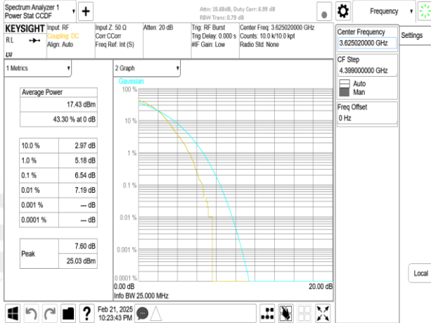
Band48_30MHz_DFT_s_OFDM_SCS15kHz_256QAM_RB160_0_CH645666
