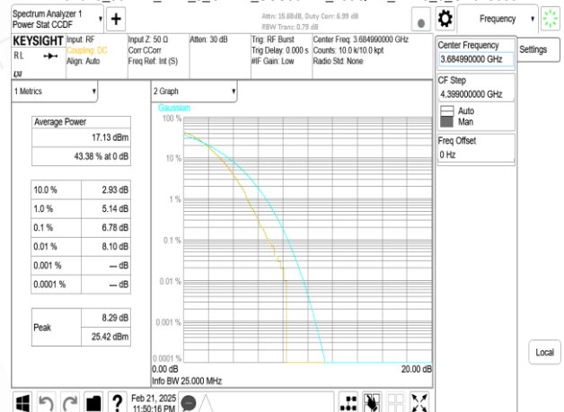
Band48_30MHz_DFT_s_OFDM_SCS30kHz_256QAM_RB75_0_CH645666
