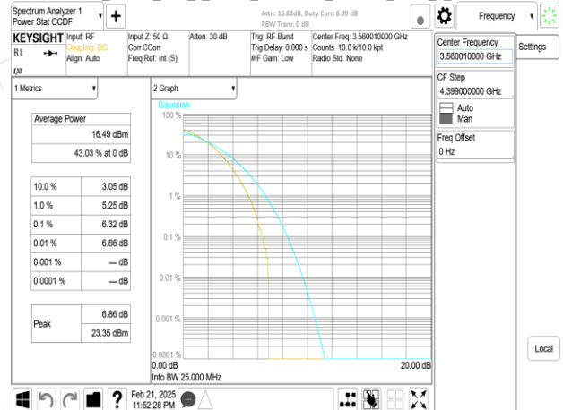
Band48_20MHz_DFT_s_OFDM_SCS30kHz_256QAM_RB50_0_CH641668
