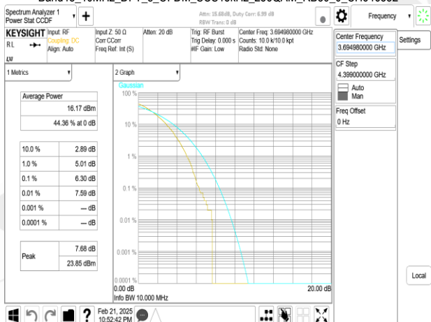
Band48_10MHz_DFT_s_OFDM_SCS15kHz_256QAM_RB50_0_CH646332
