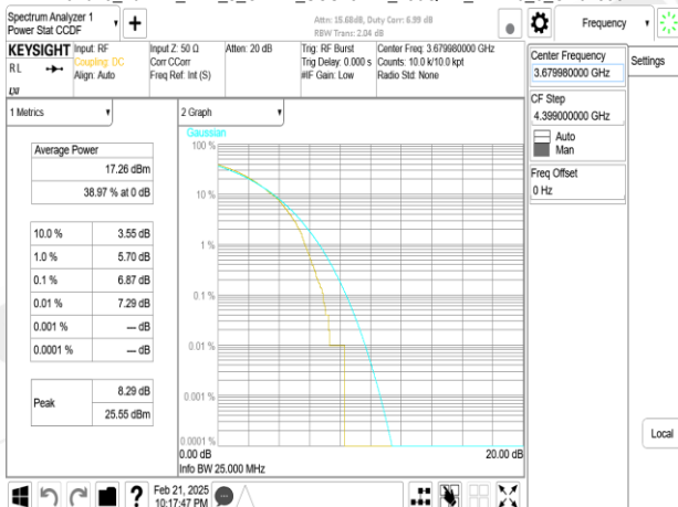
Band48_40MHz_DFT_s_OFDM_SCS15kHz_256QAM_RB216_0_CH645332
