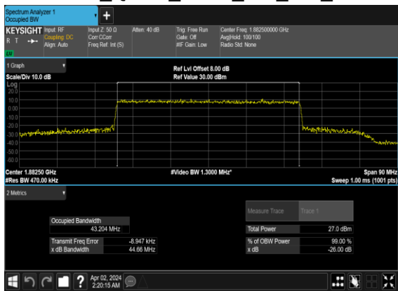
N25(45M)_CP- OFDM_QPSK_Outer_Full_Mid_CH
