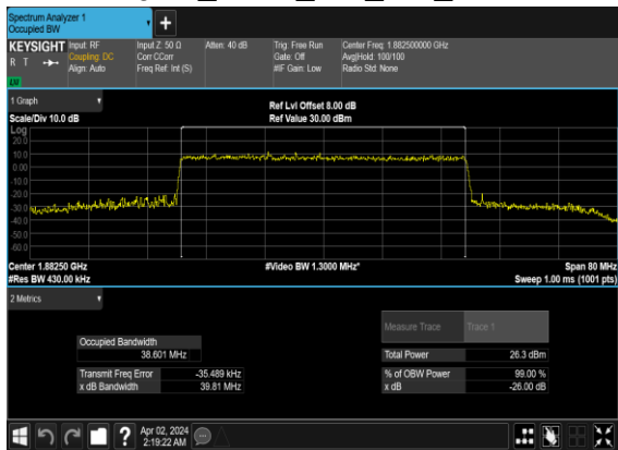
N25(40M)_CP-OFDM_64 QAM_Outer_Full_Mid_CH
