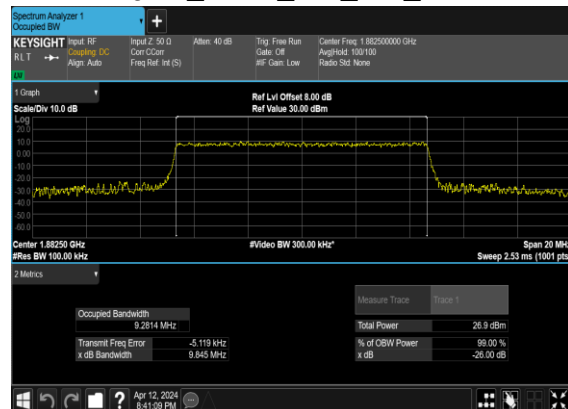
B66_N25(10M)_CP-OFDM_16 QAM_Outer_Full_Mid_CH
