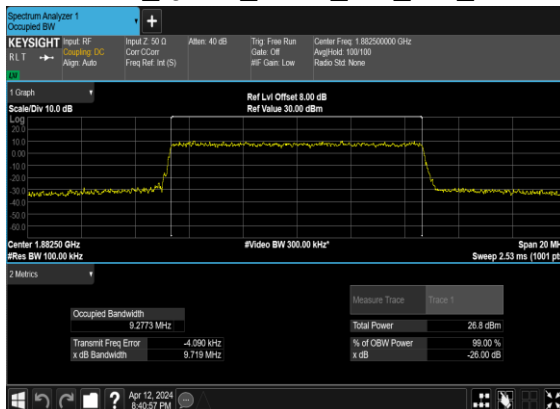
B66_N25(10M)_CP- OFDM_QPSK_Outer_Full_Mid_CH
