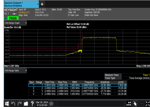
N41(50M)_DFT-s- OFDM_BPSK_Outer_Full_Low_CH
