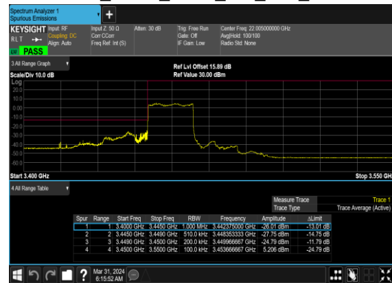
N77(20M)_DFT-s- OFDM_BPSK_Outer_Full_Low_CH
