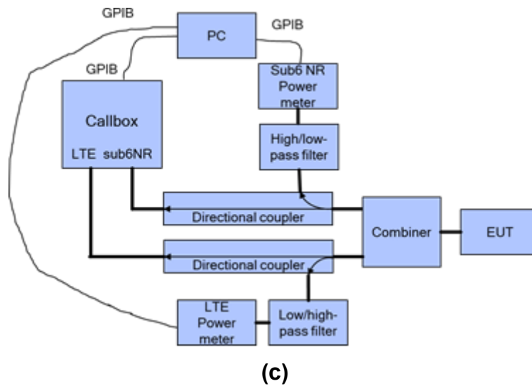
Figure 7-1 Conducted power measurement setup
