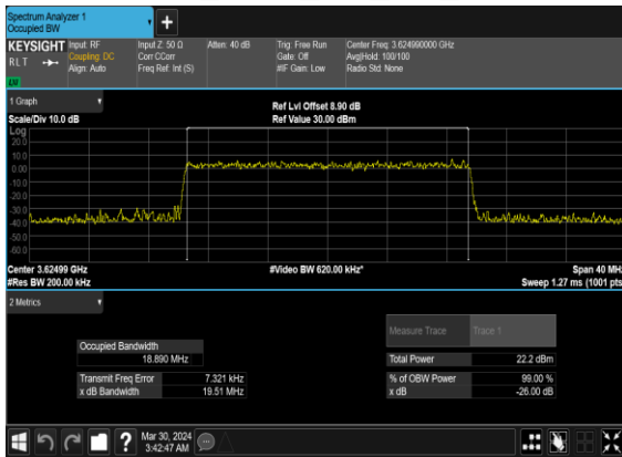
N48(20M)_CP-OFDM_16 QAM_Outer_Full_Mid_CH
