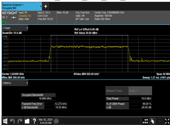
N48(20M)_CP-OFDM_256 QAM_Outer_Full_Mid_CH
