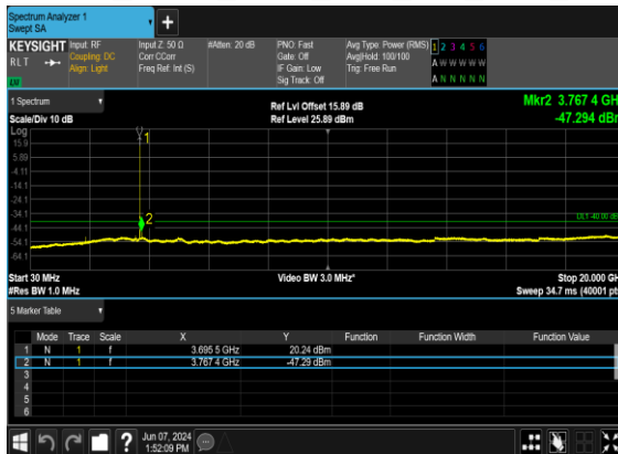
B2_N48(5M)_DFT-s-OFDM_BPSK_Edge_1RB_Left_High_CH
