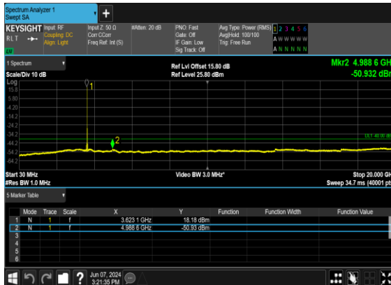
B2_N48(5M)_DFT-s-OFDM_QPSK_Edge_1RB_Left_Mid_CH
