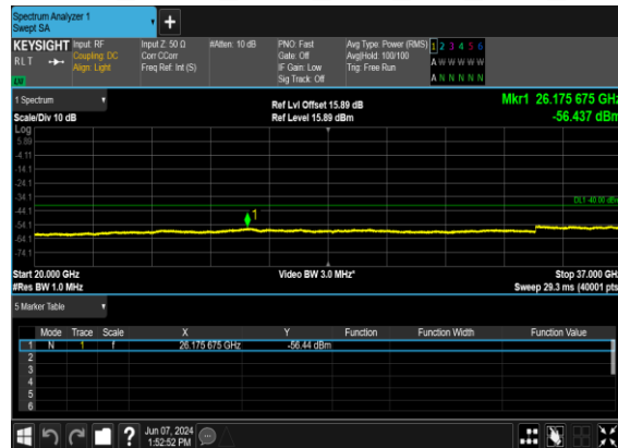
B2_N48(5M)_DFT-s-OFDM_BPSK_Edge_1RB_Left_High_CH
