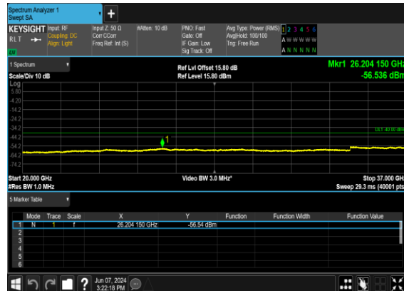
B2_N48(5M)_DFT-s-OFDM_QPSK_Edge_1RB_Left_Mid_CH
