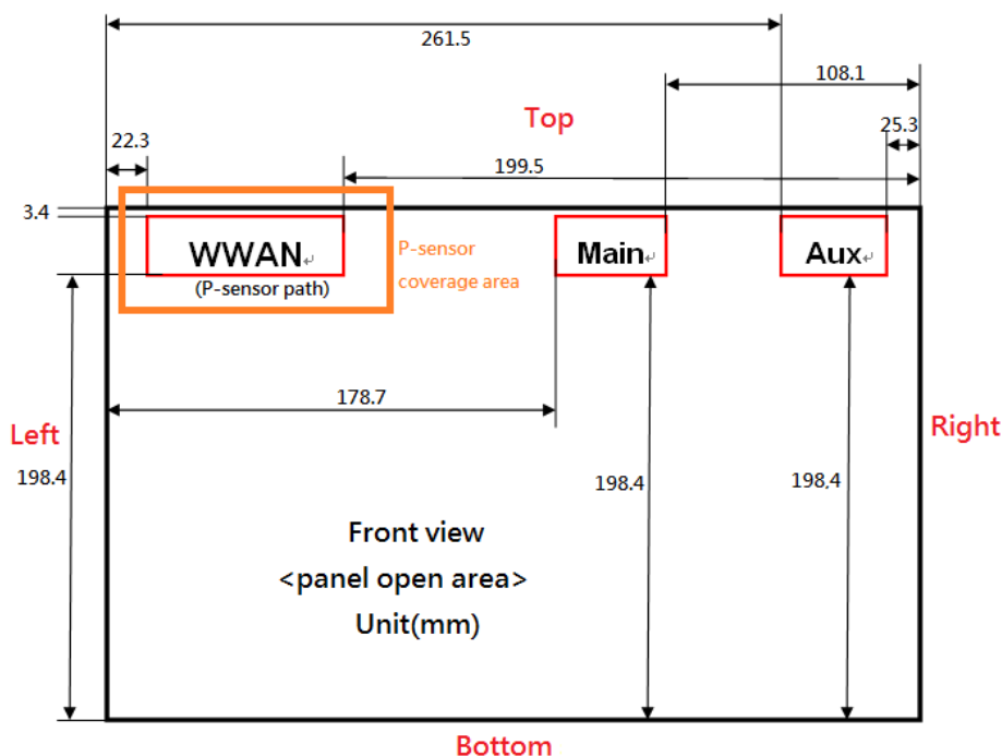
Fig.11 Antenna position of EUT (Front view)
