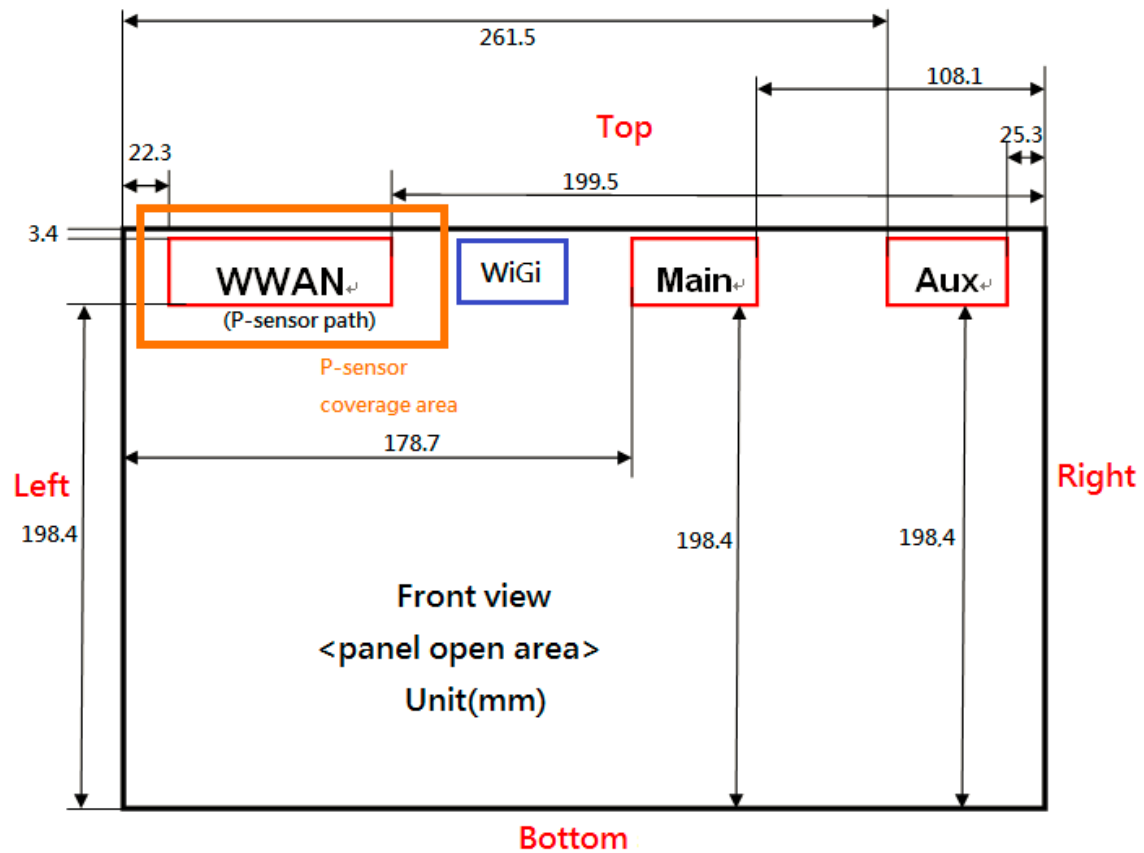
Fig.12 Antenna position of EUT (Front view)
