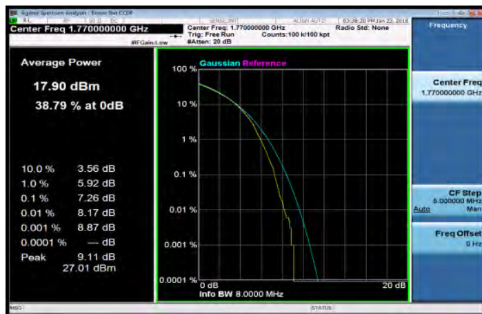
LTE_Band66_20MHz_16QAM_100_0_HighCH132572
