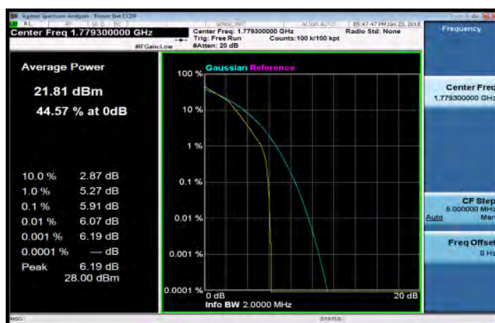
LTE_Band66_1_4MHz_16QAM_6_0_HighCH132665
