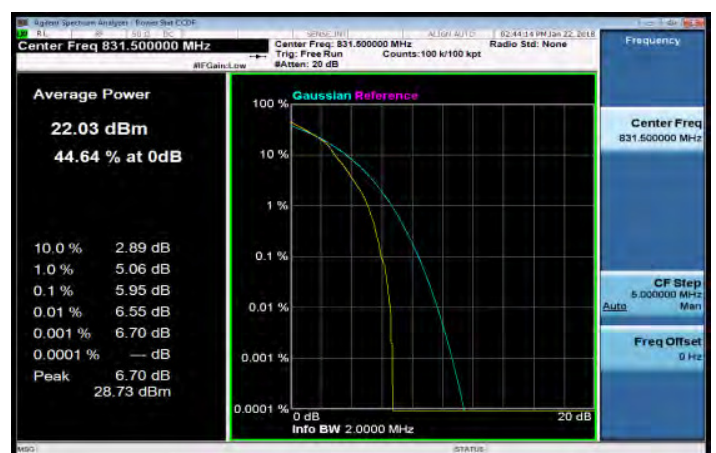
LTE_Band26_1_4MHz_16QAM_6_0_MidCH26865
