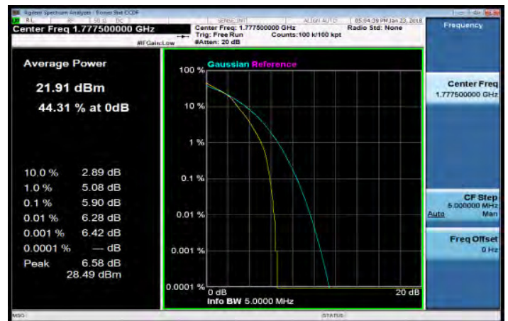
LTE_Band66_5MHz_16QAM_25_0_HighCH132647
