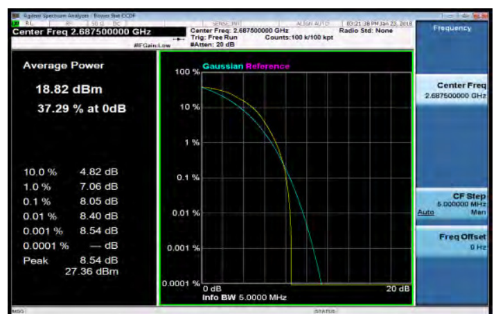
LTE_Band41_5MHz_16QAM_25_0_HighCH41565
