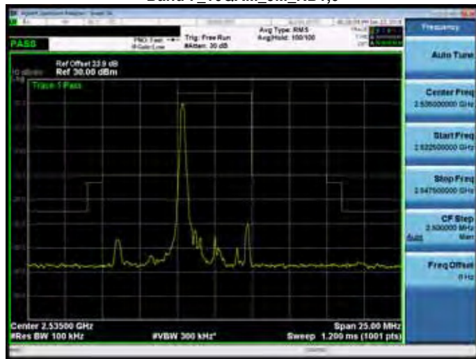
Band 7_16QAM_5M_RB1,24
