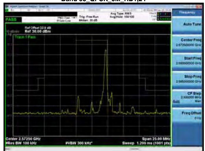
Band 38_QPSK_5M_RB1,24
