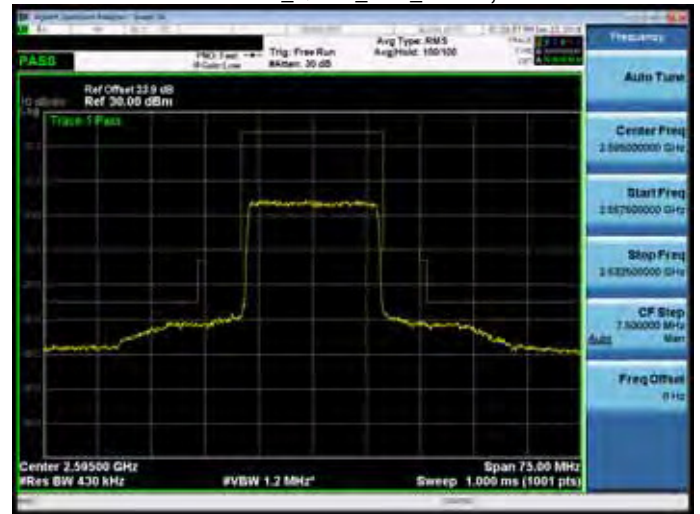
Band 38_QPSK_20M_RB1,0
