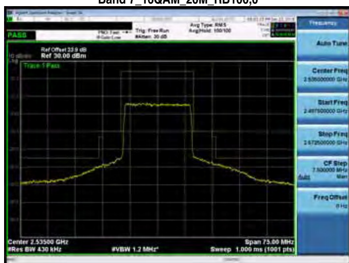
Band 7_16QAM_20M_RB100,0
