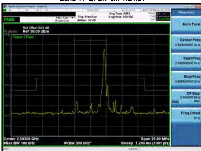
Band 41_QPSK_5M_RB1,24
