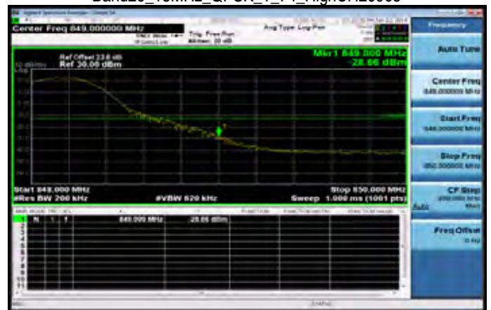
Band26_15MHz_QPSK_1_74_HighCH26965
