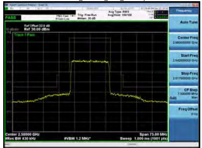
Band 38_16QAM_20M_RB1,0
