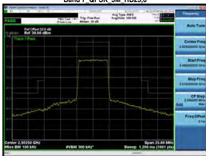
Band 7_QPSK_5M_RB25,0
