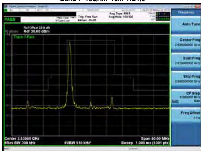
Band 7_16QAM_15M_RB1,74
