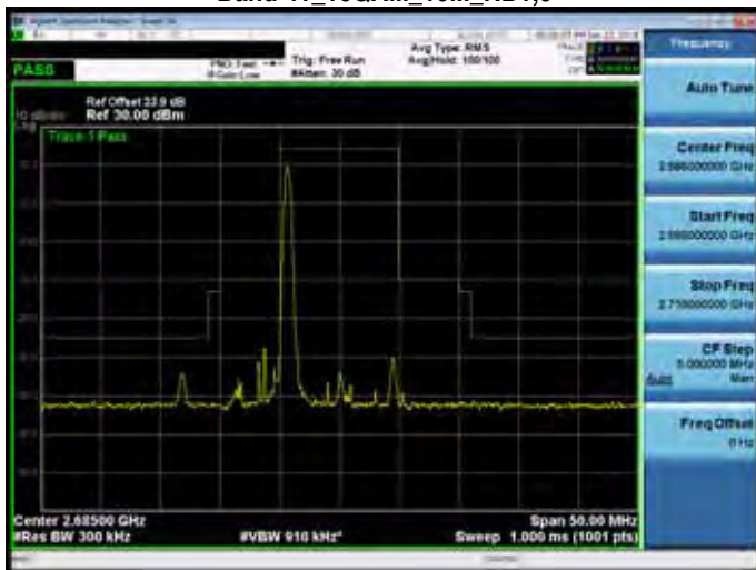
Band 41_16QAM_10M_RB1,49
