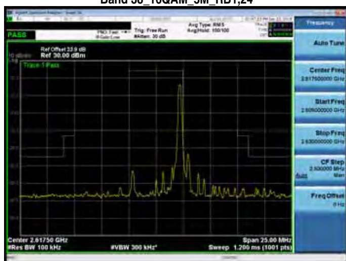
Band 38_16QAM_5M_RB1,24
