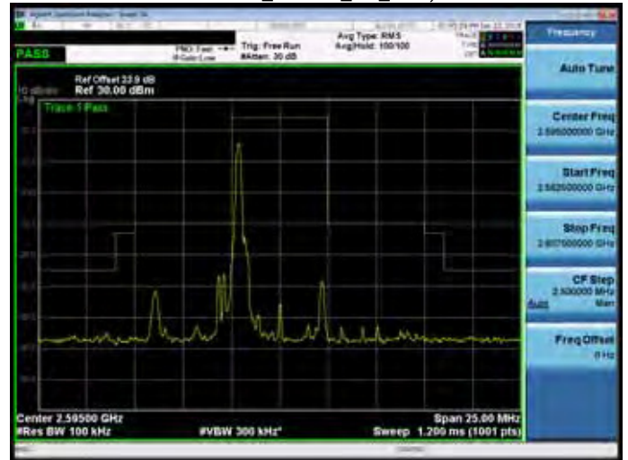
Band 38_16QAM_5M_RB1,24
