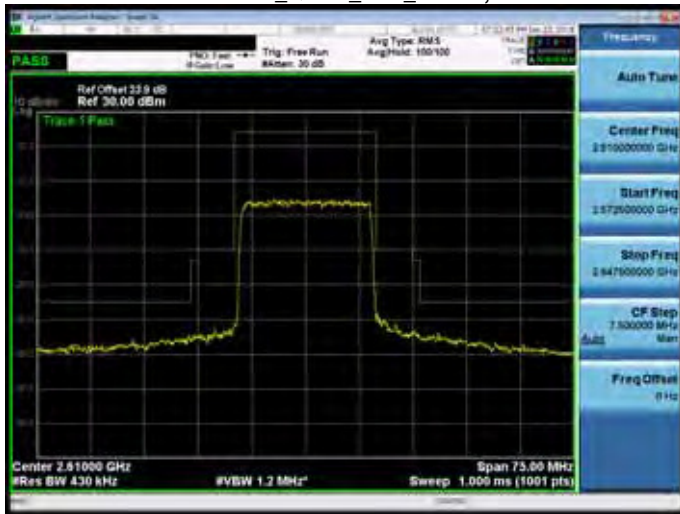
Band 38_16QAM_20M_RB1,0
