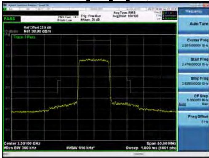
Band 41_QPSK_10M_RB1,0
