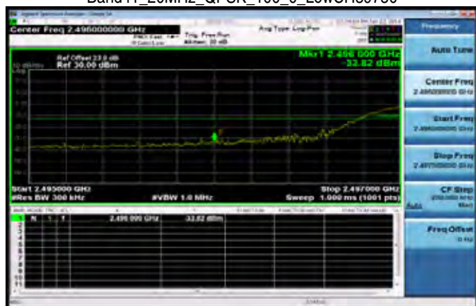
Band41_20MHz_QPSK_100_0_LowCH39750
