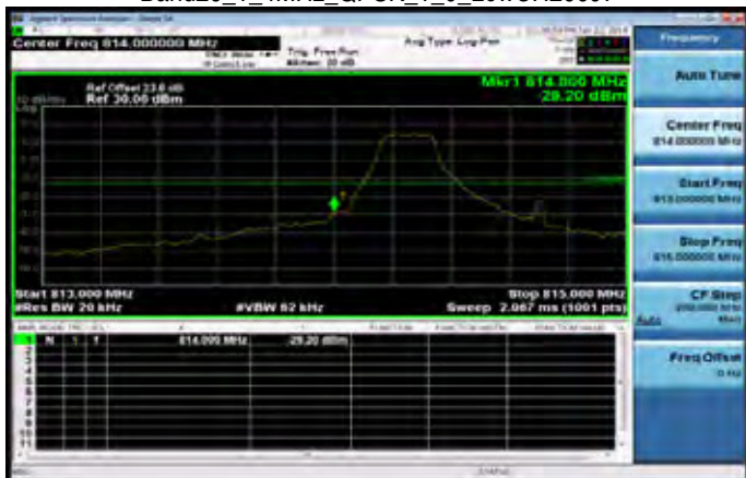
Band26_1_4MHz_QPSK_1_0_LowCH26697
