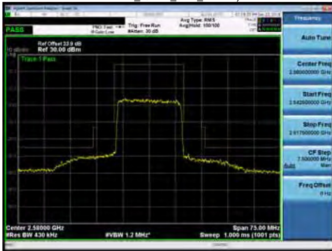
Band 38_QPSK_20M_RB1,0
