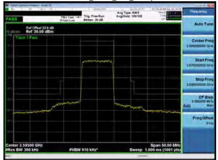
Band 38_QPSK_10M_RB1,0
