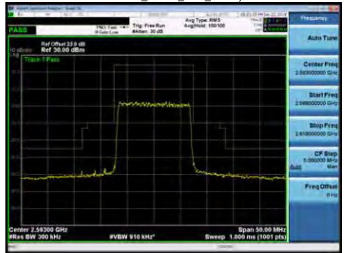
Band 41_QPSK_15M_RB1,0
