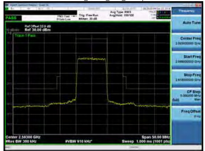
Band 41_QPSK_10M_RB1,0
