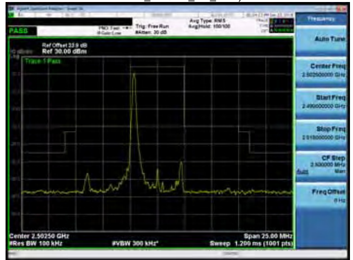
Band 7_16QAM_5M_RB1,24
