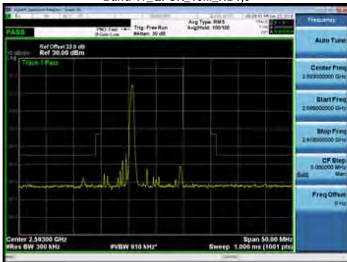
Band 41_QPSK_10M_RB1,49
