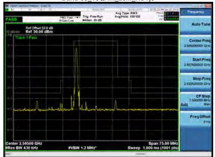
Band 38_16QAM_20M_RB1,99
