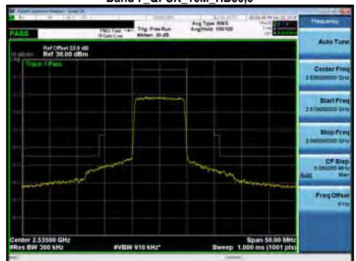
Band 7_QPSK_10M_RB50,0
