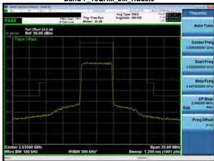
Band 7_16QAM_5M_RB25,0
