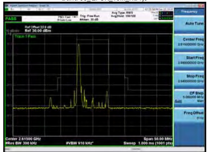
Band 38_QPSK_10M_RB1,49
