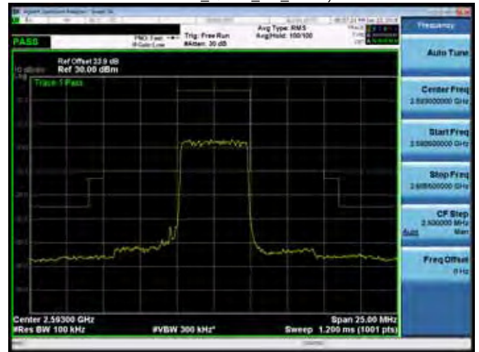
Band 41_QPSK_5M_RB1,0
