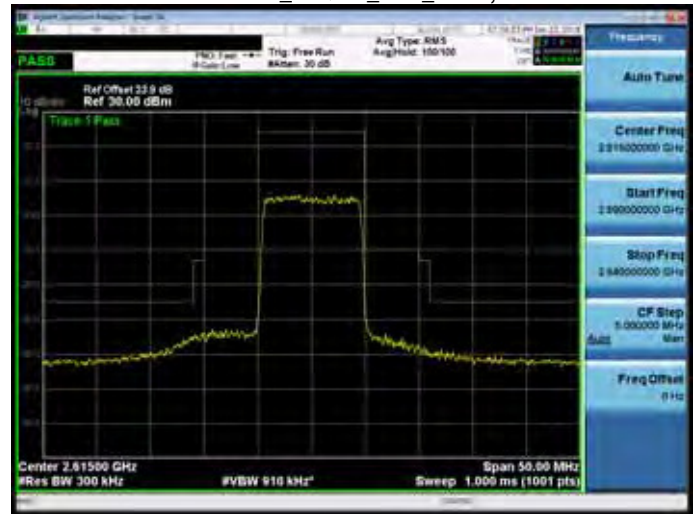
Band 38_QPSK_15M_RB1,0
