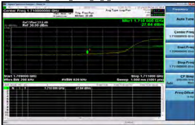
Band4_15MHz_QPSK_75_0_LowCH20025-1717.5
