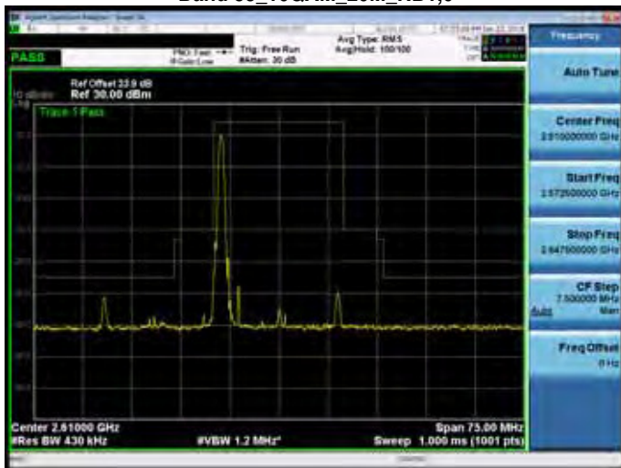
Band 38_16QAM_20M_RB1,99
