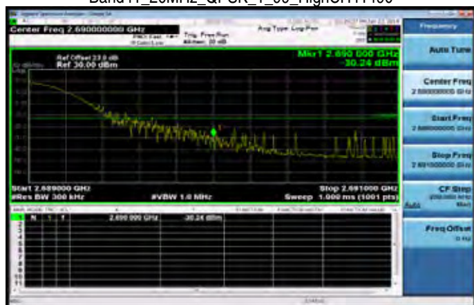
Band41_20MHz_QPSK_1_99_HighCH41490
