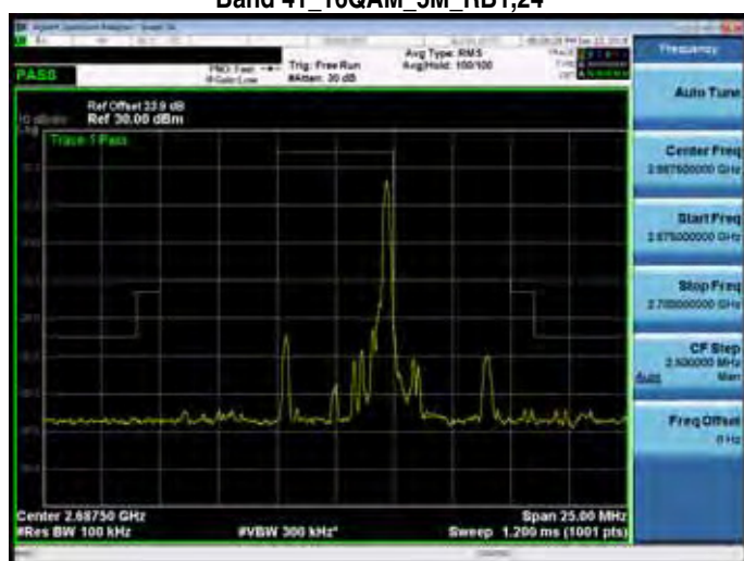
Band 41_16QAM_5M_RB1,24
