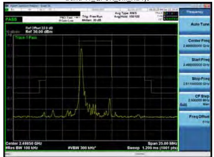
Band 41_QPSK_5M_RB1,24
