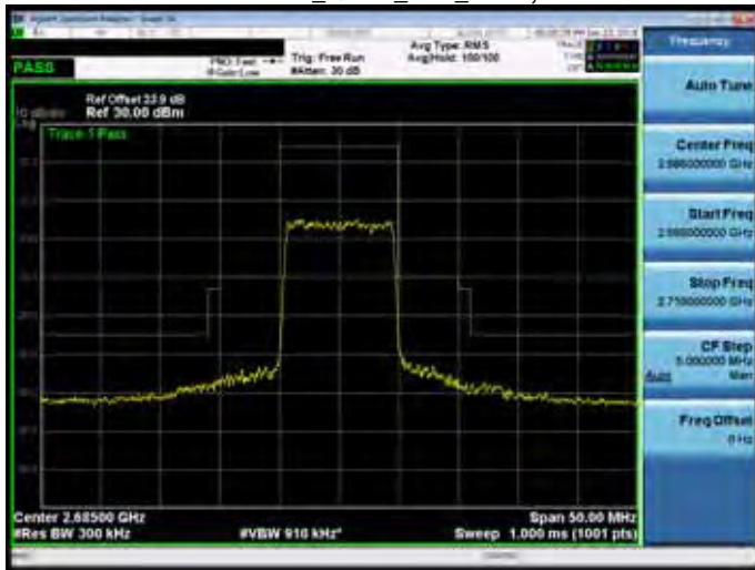
Band 41_16QAM_10M_RB1,0
