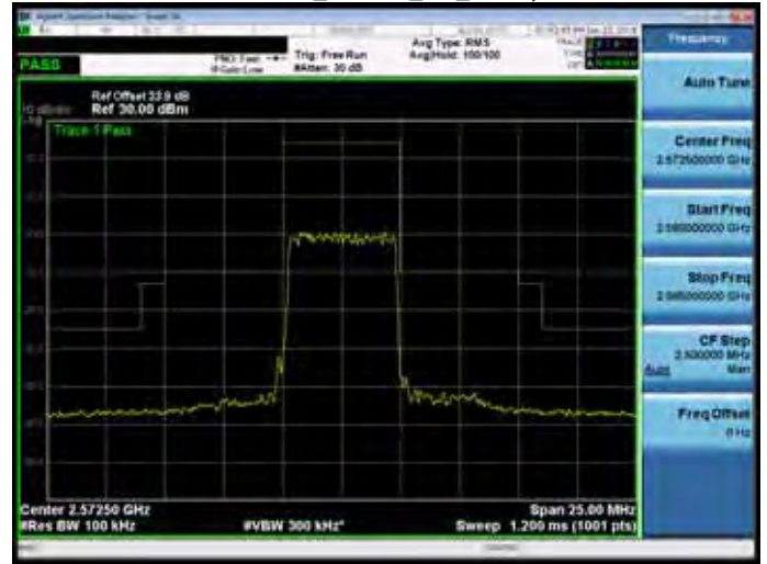
Band 38_16QAM_5M_RB1,0
