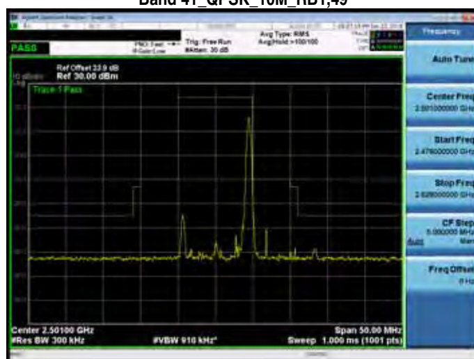
Band 41_QPSK_10M_RB1,49
