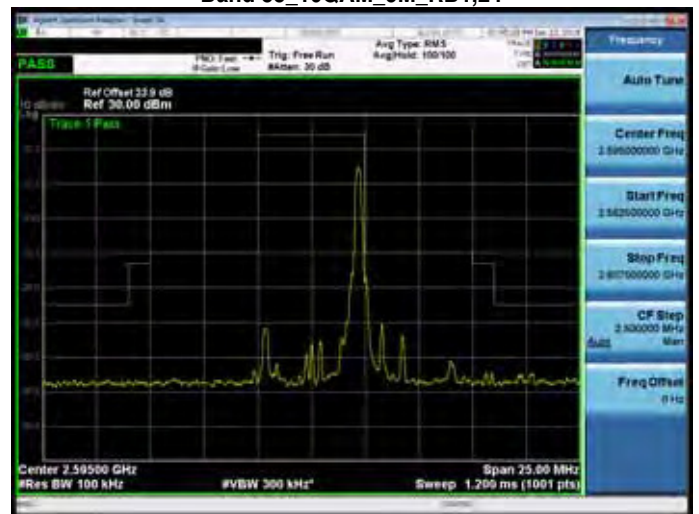
Band 38_16QAM_5M_RB1,24
