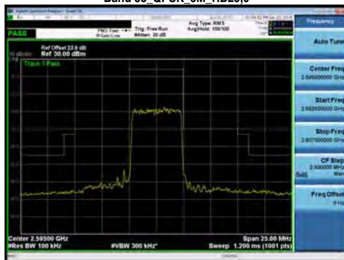
Band 38_QPSK_5M_RB1,0
