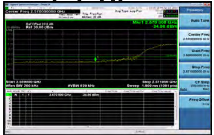
Band38_15MHz_QPSK_75_0_LowCH37825-2577.5
