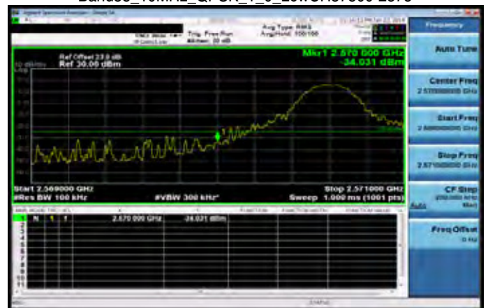
Band38_10MHz_QPSK_1_0_LowCH37800-2575
