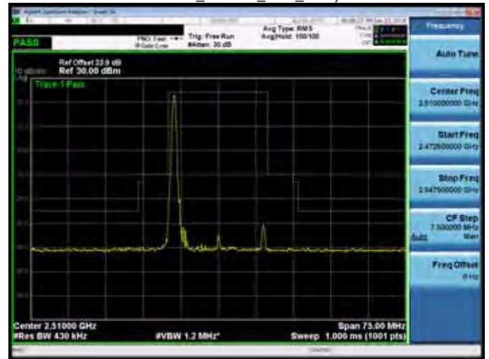
Band 7_16QAM_20M_RB1,99
