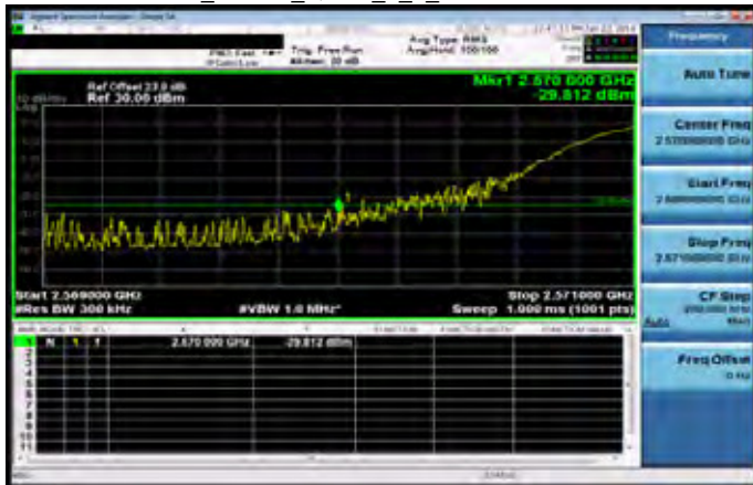
Band38_20MHz_QPSK_1_0_LowCH37850-2580
