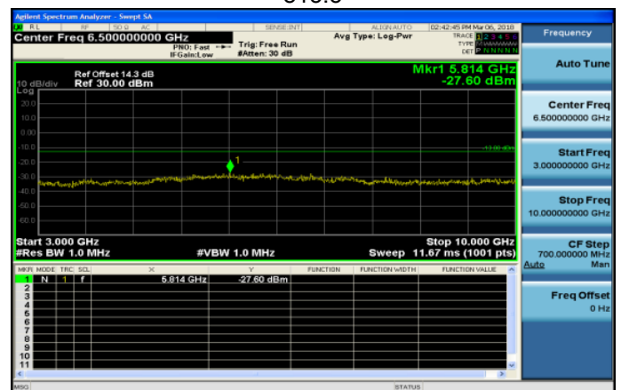
3GHz~10GHz_Band26_3MHz_QPSK_1_0_LowCH26705- 815.5
