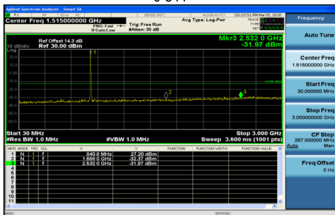
30MHz~3GHz_Band26_10MHz_QPSK_1_0_HighCH2699 0-844
