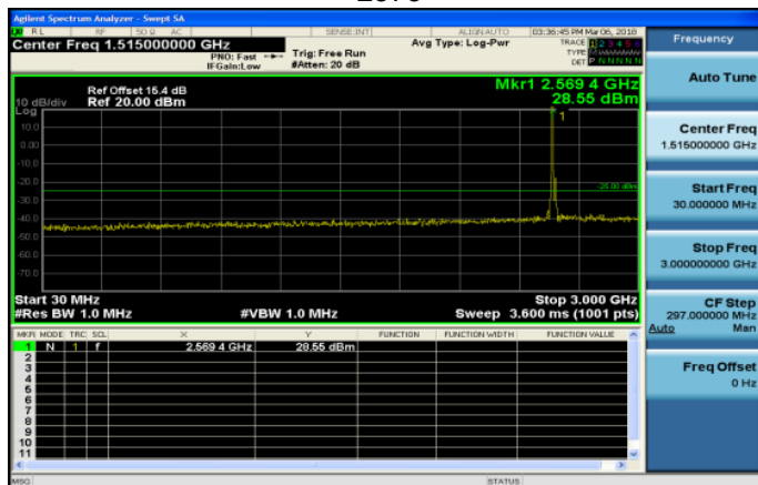
30MHz~3GHz_Band38_10MHz_QPSK_1_0_LowCH37800-2575
