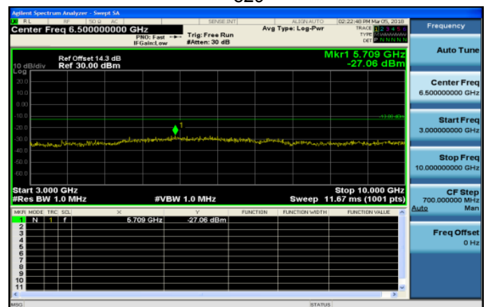
3GHz~10GHz_Band26_10MHz_QPSK_1_0_LowCH26840-829
