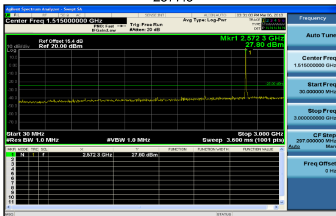
30MHz~3GHz_Band38_15MHz_QPSK_1_0_LowCH37825 -2577.5
