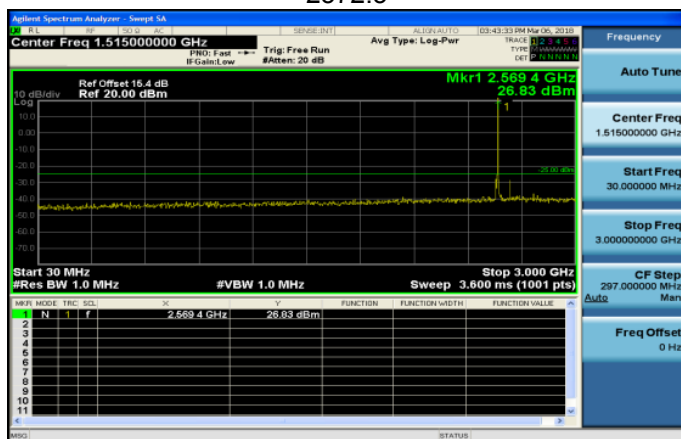
30MHz~3GHz_Band38_5MHz_QPSK_1_0_LowCH37775-2572.5
