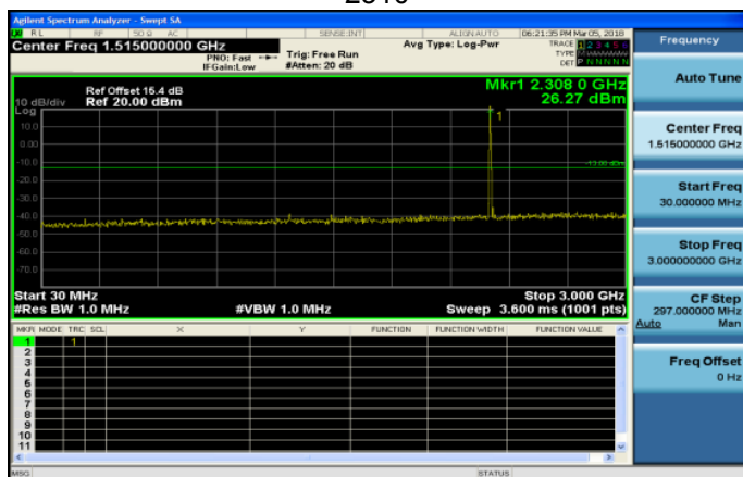
30MHz~3GHz_Band30_5MHz_QPSK_1_0_MidCH27710-2310
