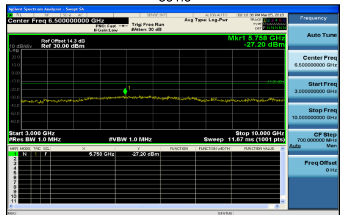
3GHz~10GHz_Band26_15MHz_QPSK_1_0_LowCH26865 -831.5
