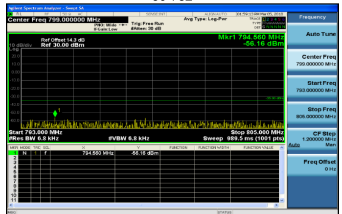
793MHz~805MHz_Band13_5MHz_QPSK_1_0_MidCH23230-782
