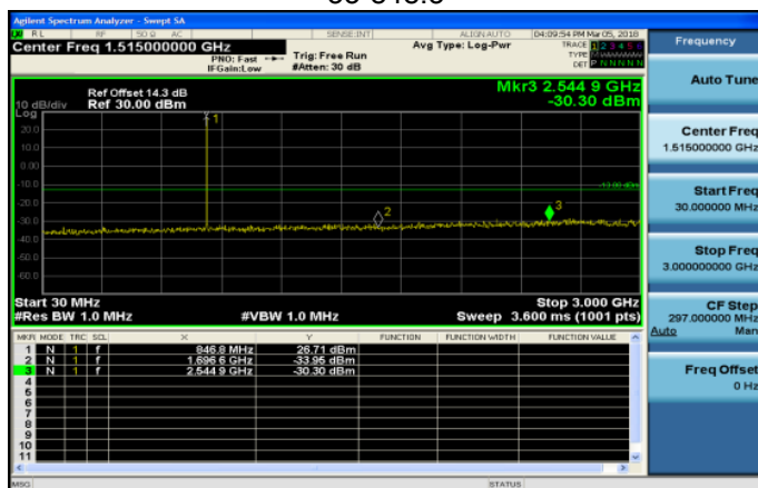
30MHz~3GHz_Band26_1_4MHz_QPSK_1_0_HighCH270 33-848.3
