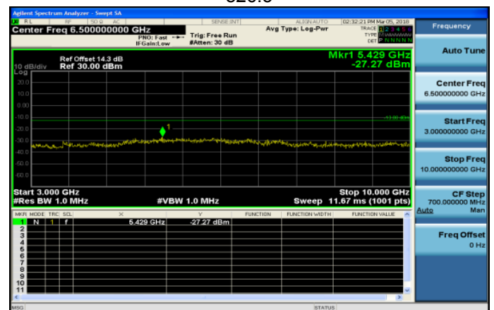
3GHz~10GHz_Band26_5MHz_QPSK_1_0_LowCH26815-826.5
