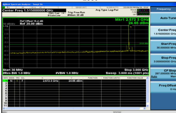
30MHz~3GHz_Band38_20MHz_QPSK_1_0_LowCH37850 -2580
