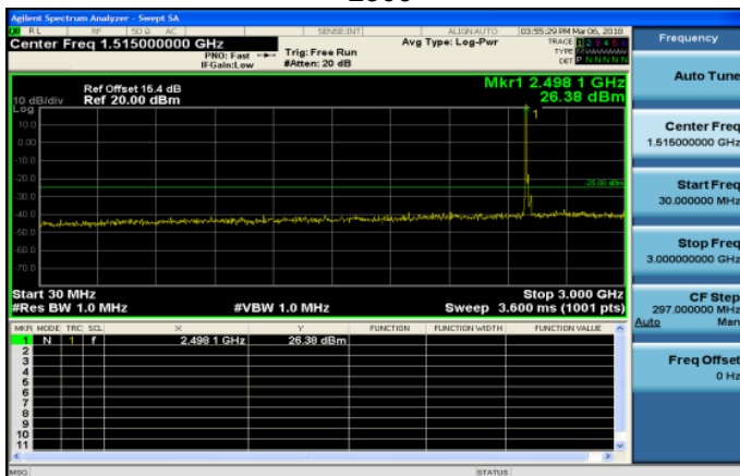
30MHz~3GHz_Band41_20MHz_QPSK_1_0_LowCH39750 -2506
