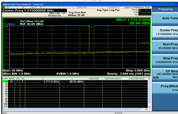
30MHz~3GHz_Band66_5MHz_QPSK_1_0_LowCH131997 -1712.5
