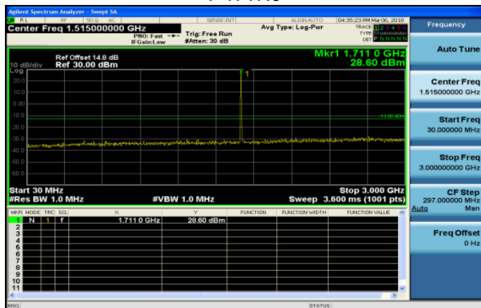
30MHz~3GHz_Band66_15MHz_QPSK_1_0_LowCH13204 7-1717.5
