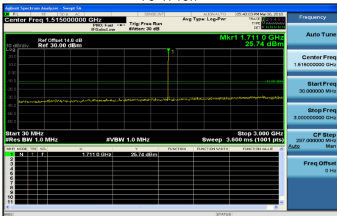
30MHz~3GHz_Band66_1_4MHz_QPSK_1_0_LowCH1319 79-1710.7
