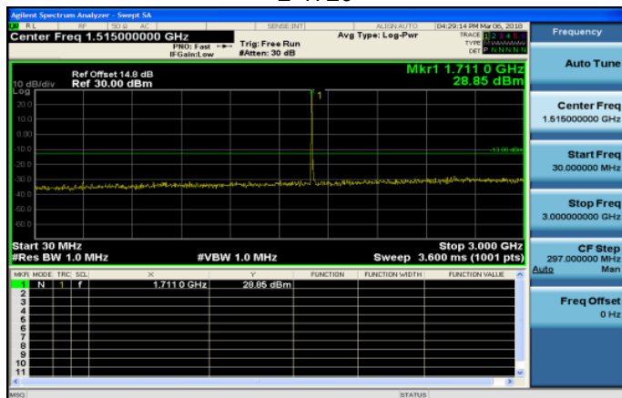
30MHz~3GHz_Band66_20MHz_QPSK_1_0_LowCH13207 2-1720
