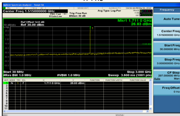
30MHz~3GHz_Band66_3MHz_QPSK_1_0_LowCH131987 -1711.5
