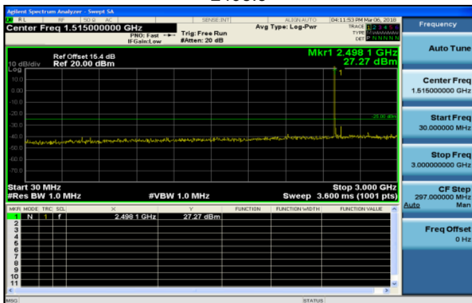
30MHz~3GHz_Band41_5MHz_QPSK_1_0_LowCH39675- 2498.5
