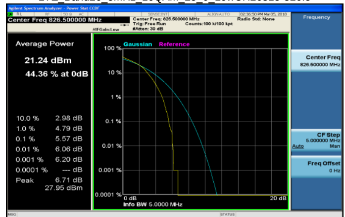
LTE Band26 5MHz 16QAM 25 0 LowCH26815-826.5
