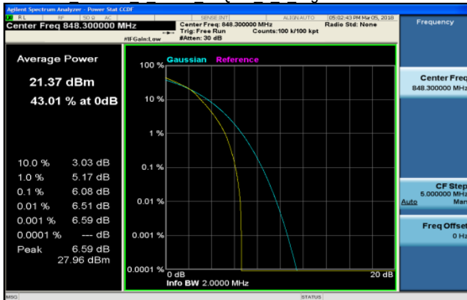
LTE Band26 1 4MHz 16QAM 6 0 HighCH27033-848.3
