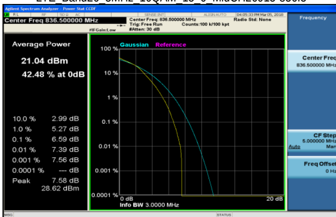
LTE Band26 3MHz 16QAM 15 0 MidCH26915-836.5
