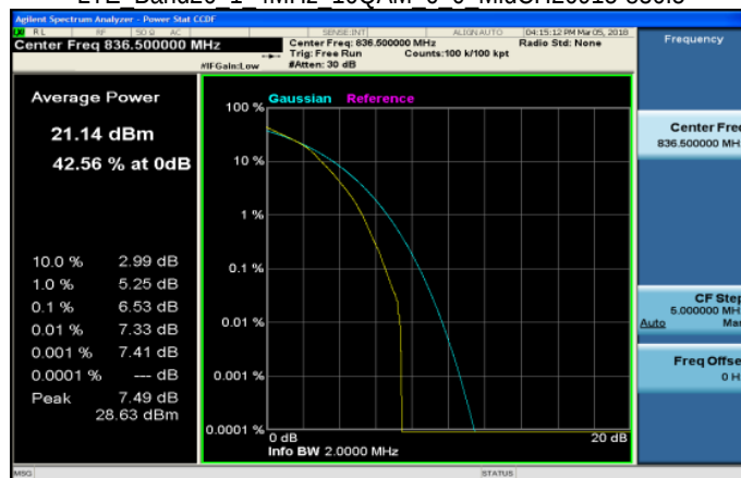
LTE Band26 1 4MHz 16QAM 6 0 MidCH26915-836.5
