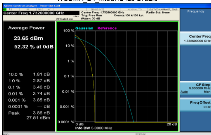
WCDMA_B4_MidCH1413-1732.6
