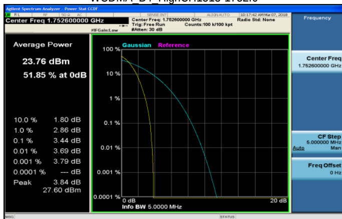
WCDMA_B4_HighCH1513-1752.6
