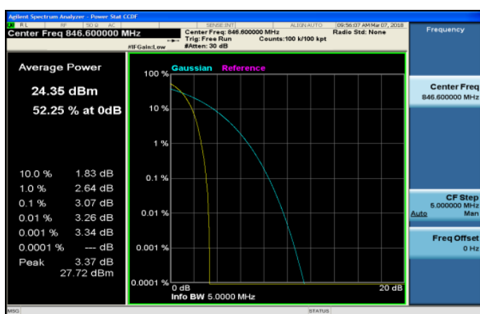
HSUPA_B5_HighCH4233-846.6
