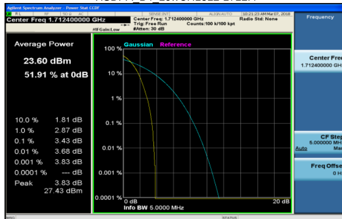
HSDPA_B4_LowCH1312-1712.4
