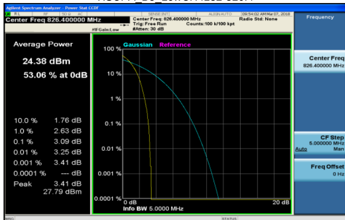
HSUPA_B5_LowCH4132-826.4
