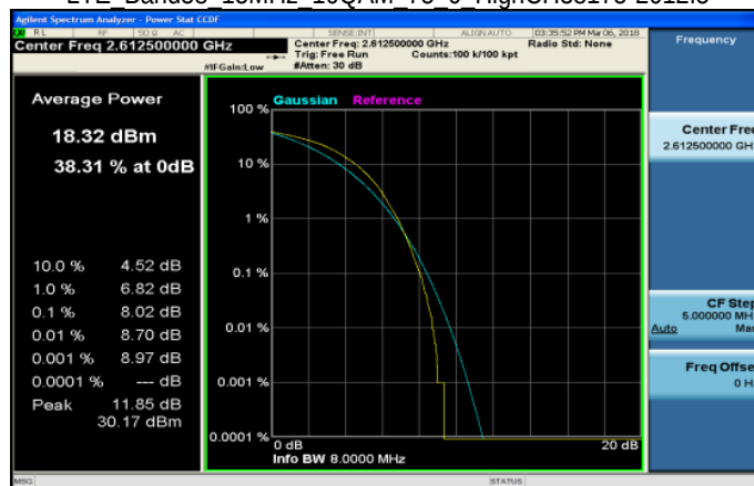
LTE Band38 15MHz 16QAM 75 0 HighCH38175-2612.5
