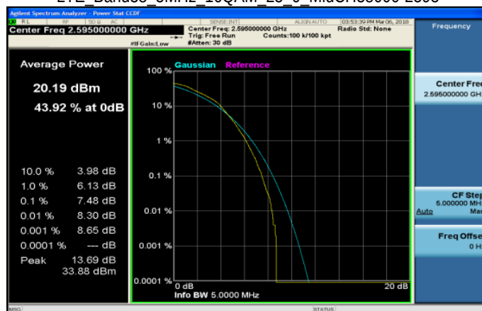
LTE Band38 5MHz 16QAM 25 0 MidCH38000-2595
