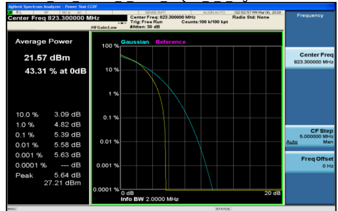
Part 90 LTE Band26 1 4MHz 16QAM 6 0 HighCH26783-823.3
