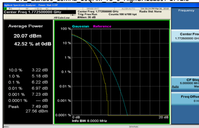
LTE Band66 15MHz 16QAM 75 0 HighCH132597-1772.5
