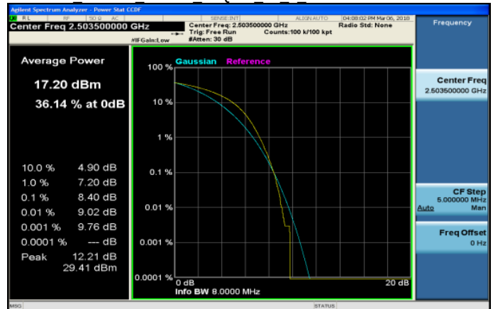
LTE Band41 15MHz 16QAM 75 0 LowCH39725-2503.5
