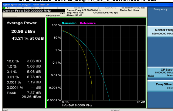
LTE Band26 10MHz 16QAM 50 0 LowCH26840-829
