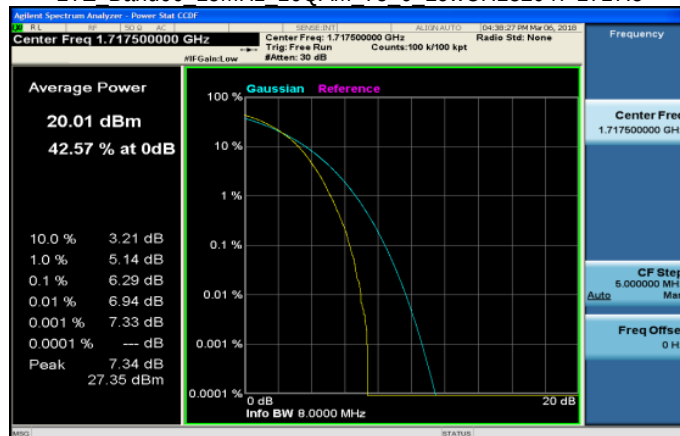
LTE Band66 15MHz 16QAM 75 0 LowCH132047-1717.5
