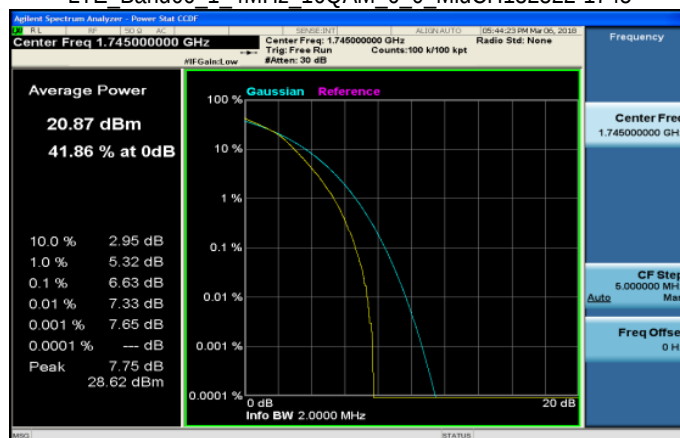
LTE_Band66 1 4MHz 16QAM 6 0 MidCH132322-1745
