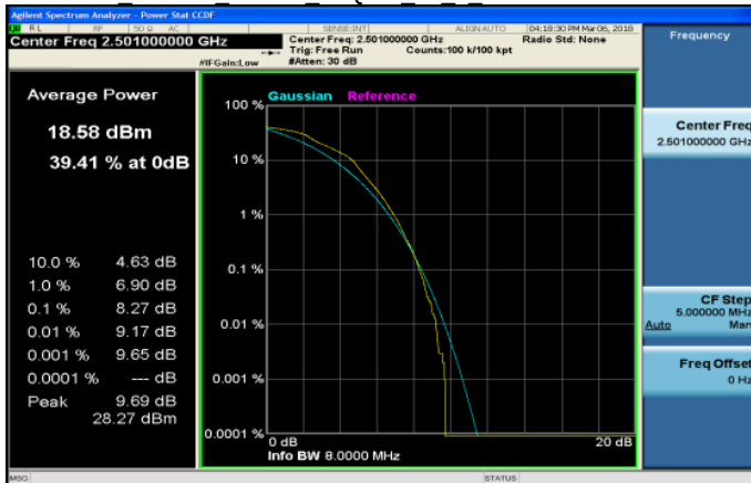
LTE Band41 10MHz 16QAM 50 0 LowCH39700-2501
