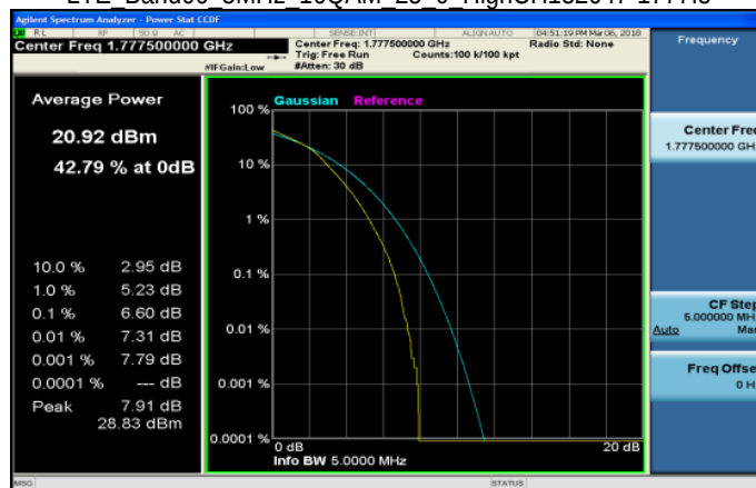
LTE Band66 5MHz 16QAM 25 0 HighCH132647-1777.5
