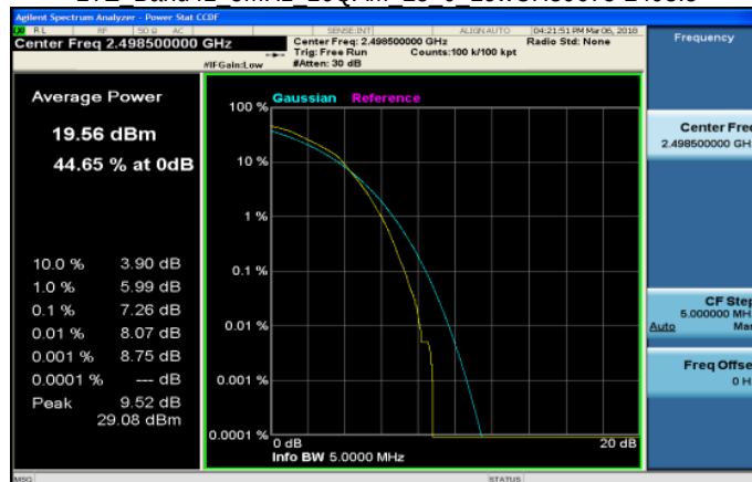
LTE Band41 5MHz 16QAM 25 0 LowCH39675-2498.5
