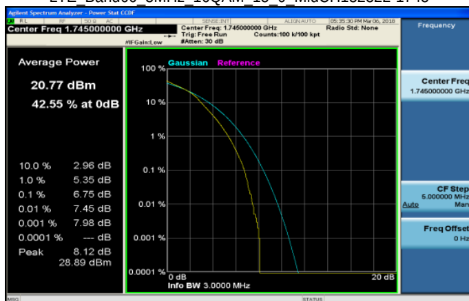
LTE Band66 3MHz 16QAM 15 0 MidCH132322-1745
