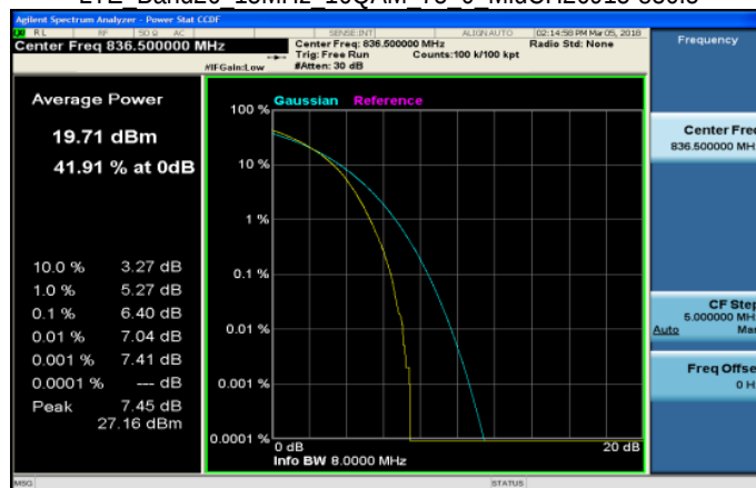
LTE Band26 15MHz 16QAM 75 0 MidCH26915-836.5
