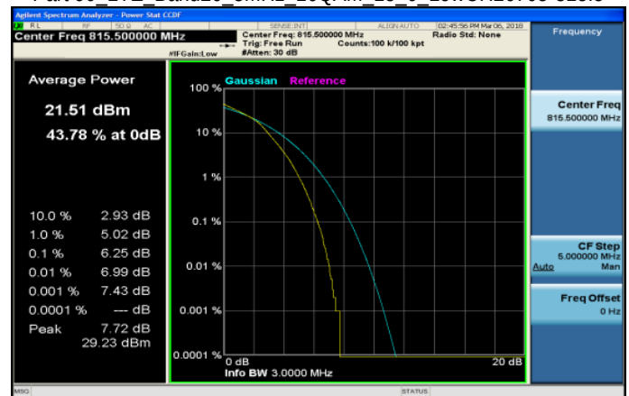
Part 90 LTE Band26 3MHz 16QAM 15 0 LowCH26705-815.5
