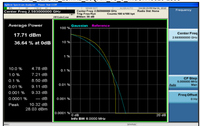
LTE Band41 15MHz 16QAM 75 0 MidCH40620-2593
