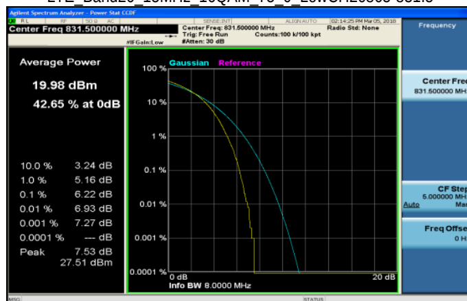
LTE Band26 15MHz 16QAM 75 0 LowCH26865-831.5
