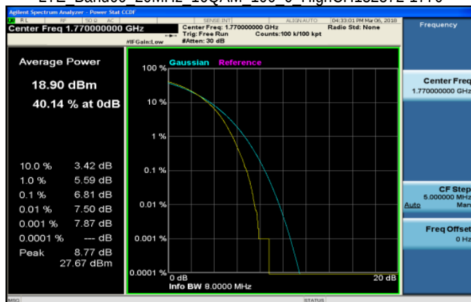
LTE Band66 20MHz 16QAM 100 0 HighCH132572-1770
