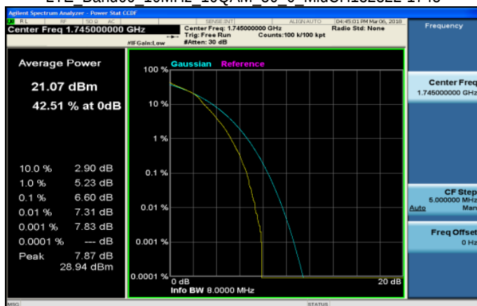
LTE Band66 10MHz 16QAM 50 0 MidCH132322-1745
