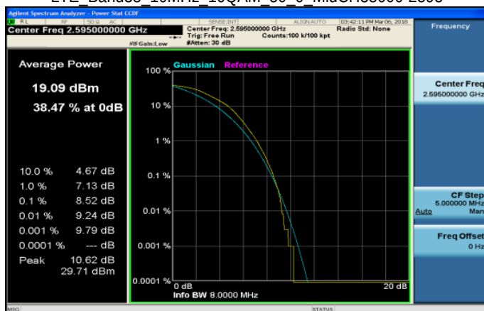
LTE Band38 10MHz 16QAM 50 0 MidCH38000-2595
