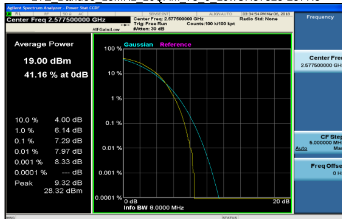
LTE Band38 15MHz 16QAM 75 0 LowCH37825-2577.5
