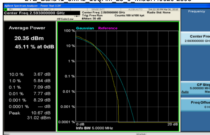
LTE Band41 5MHz 16QAM 25 0 MidCH40620-2593
