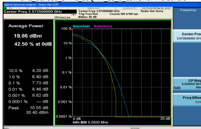
LTE Band38 5MHz 16QAM 25 0 LowCH37775-2572.5
