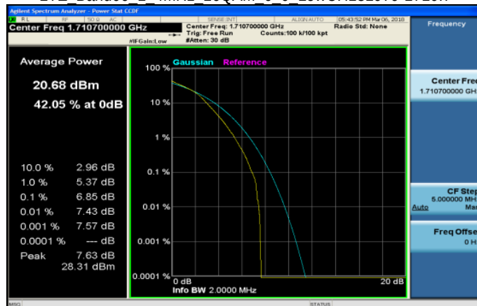
LTE_Band66 1 4MHz 16QAM 6 0 LowCH131979-1710.7
