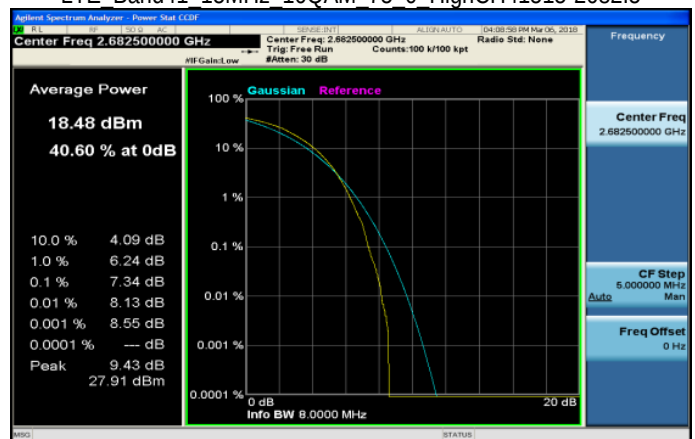
LTE Band41 15MHz 16QAM 75 0 HighCH41515-2682.5
