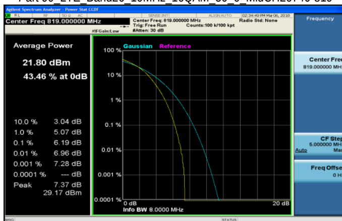
Part 90 LTE Band26 10MHz 16QAM 50 0 MidCH26740-819
