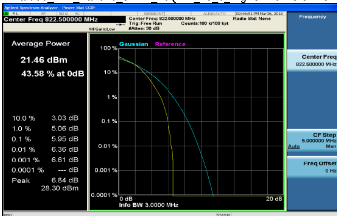
Part 90 LTE Band26 3MHz 16QAM 15 0 HighCH26775-822.5
