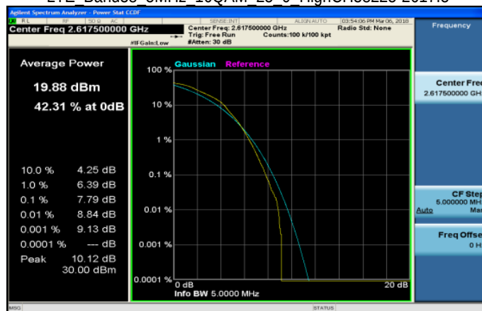
LTE Band38 5MHz 16QAM 25 0 HighCH38225-2617.5
