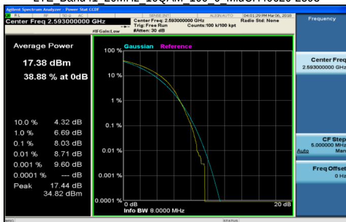
LTE_Band41 20MHz 16QAM 100 0 MidCH40620-2593
