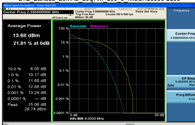
LTE Band38 20MHz 16QAM 100 0 MidCH38000-2595
