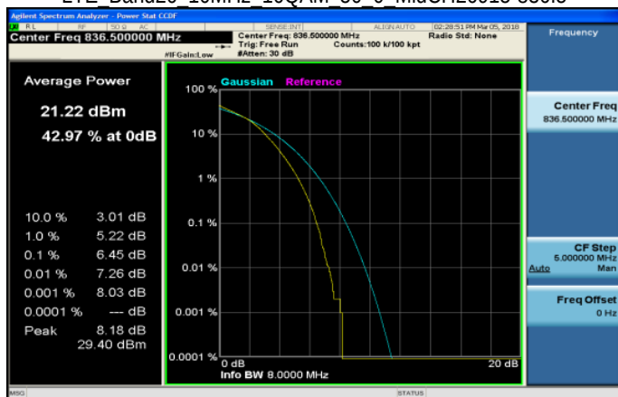
LTE Band26 10MHz 16QAM 50 0 MidCH26915-836.5
