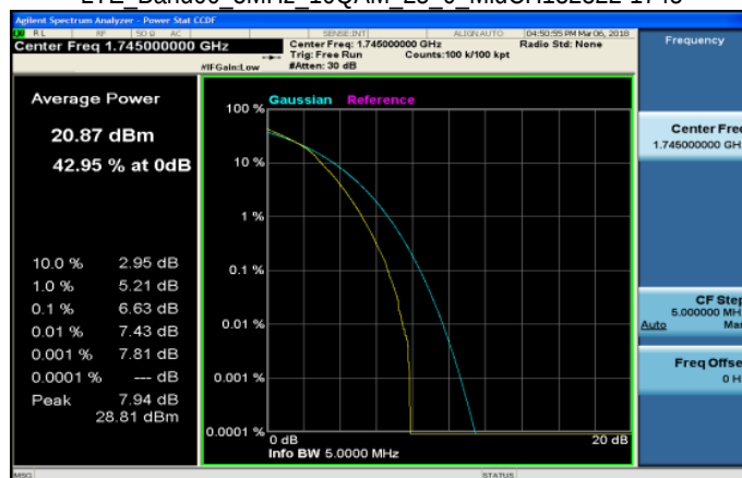
LTE Band66 5MHz 16QAM 25 0 MidCH132322-1745
