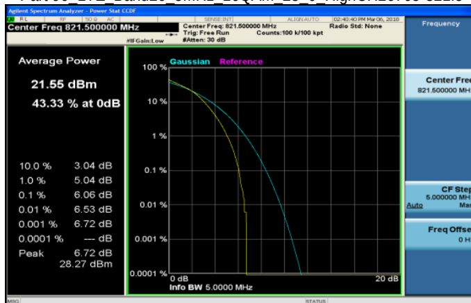
Part 90 LTE Band26 5MHz 16QAM 25 0 HighCH26765-821.5
