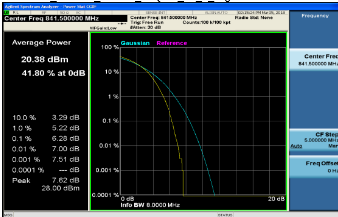
LTE Band26 15MHz 16QAM 75 0 HighCH26965-841.5
