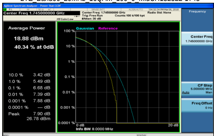
LTE Band66 20MHz 16QAM 100 0 MidCH132322-1745
