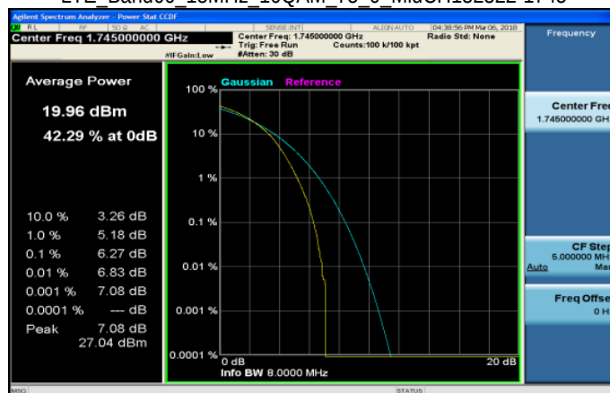
LTE Band66 15MHz 16QAM 75 0 MidCH132322-1745
