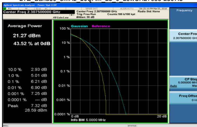
LTE Band30 5MHz 16QAM 25 0 LowCH27685-2307.5
