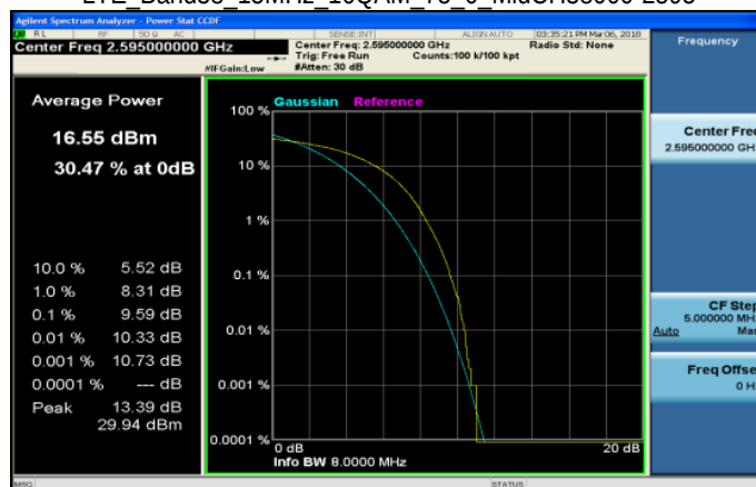
LTE Band38 15MHz 16QAM 75 0 MidCH38000-2595
