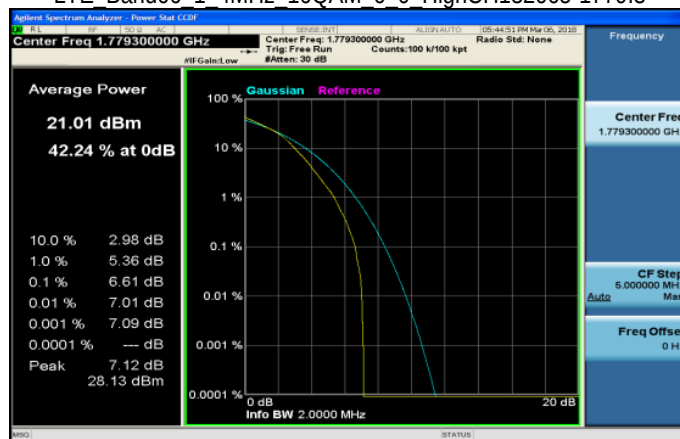
LTE_Band66 1 4MHz 16QAM 6 0 HighCH132665-1779.3
