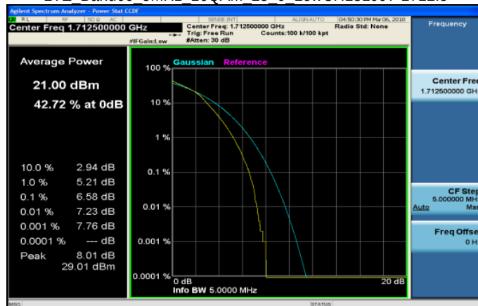
LTE Band66 5MHz 16QAM 25 0 LowCH131997-1712.5
