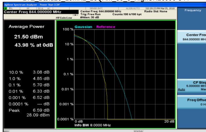
LTE Band26 10MHz 16QAM 50 0 HighCH26990-844
