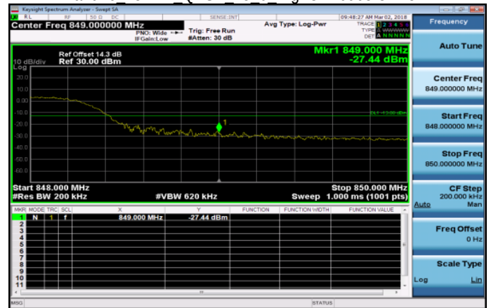
Band26 15MHz QPSK 75 0 HighCH26965-841.5
