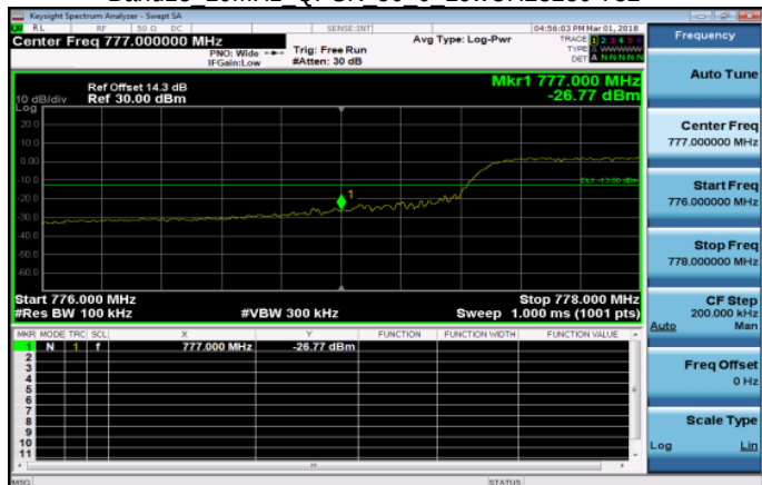
Band13 10MHz QPSK 50 0 LowCH23230-782
