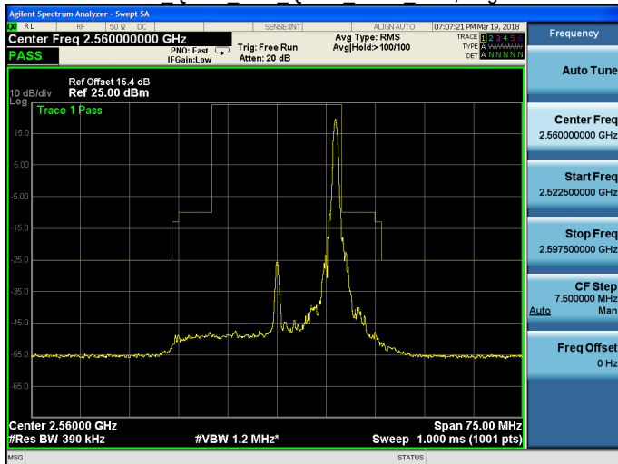
Band 7 QPSK 20M QPSK HIGH RB100,0.gif
