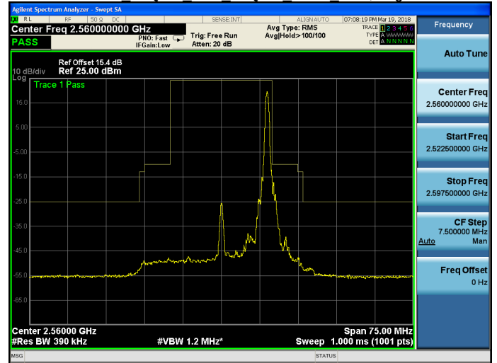
Band 7 16QAM 20M 16QAM HIGH RB100,0.gif
