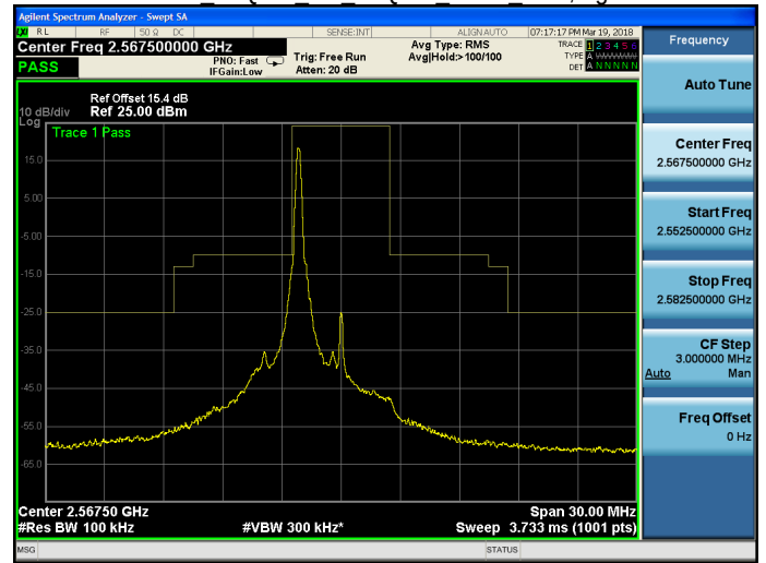
Band 7 16QAM 5M 16QAM HIGH RB1,24.gif
