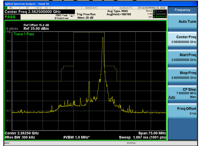
Band 7 16QAM 15M 16QAM HIGH RB75,0.gif
