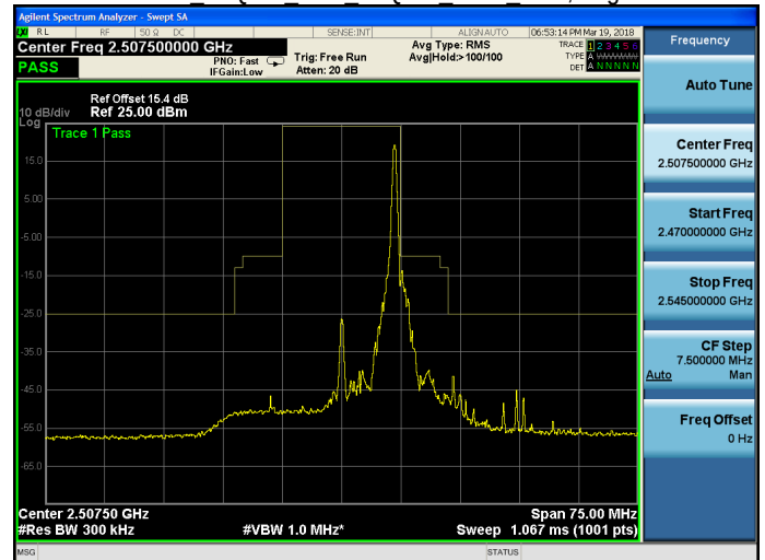
Band 7 16QAM 15M 16QAM LOW RB75,0.gif
