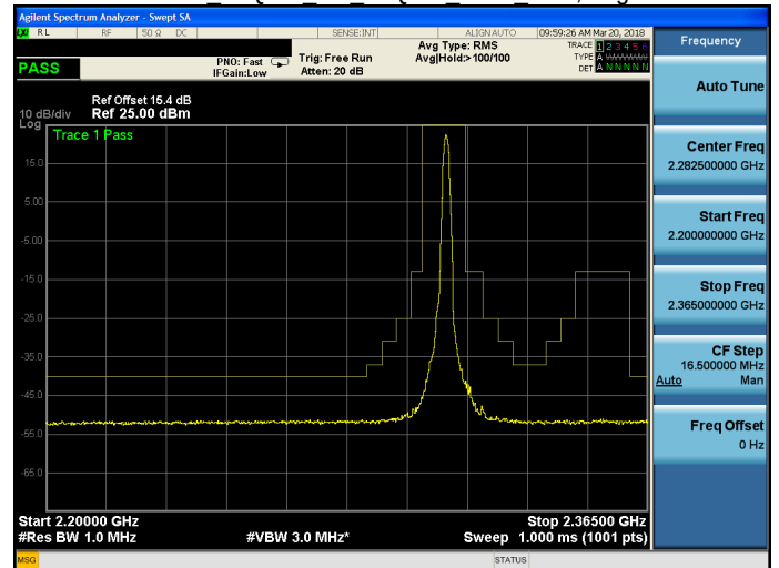
Band 30 16QAM 5M 16QAM LOW RB25,0.gif
