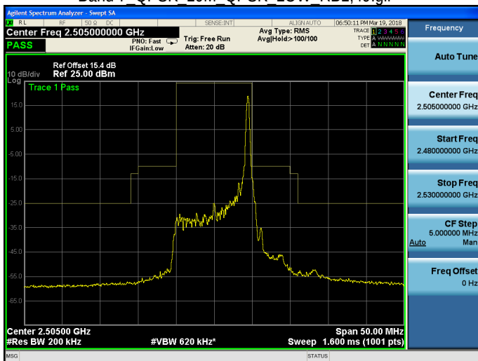
Band 7 QPSK 10M QPSK LOW RB50,0.gif
