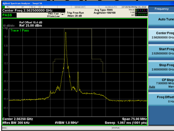
Band 7 QPSK 15M QPSK HIGH RB1,74.gif
