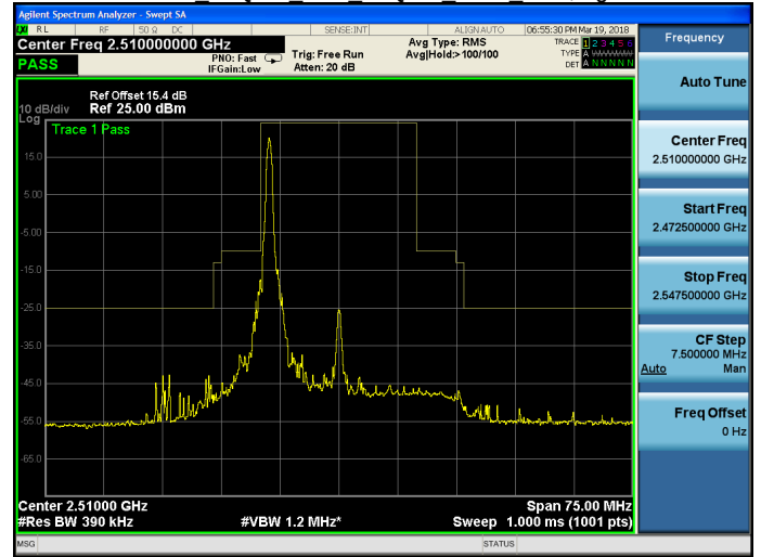
Band 7 16QAM 20M 16QAM LOW RB1,99.gif
