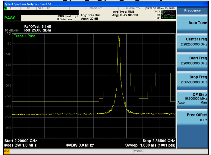
Band 30 QPSK 5M QPSK MID RB1,24.gif
