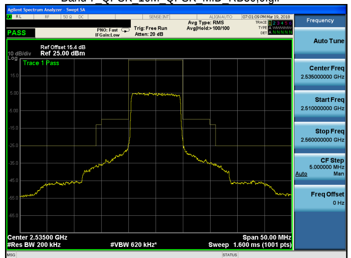
Band 7 QPSK 10M QPSK MID RB50,0.gif
