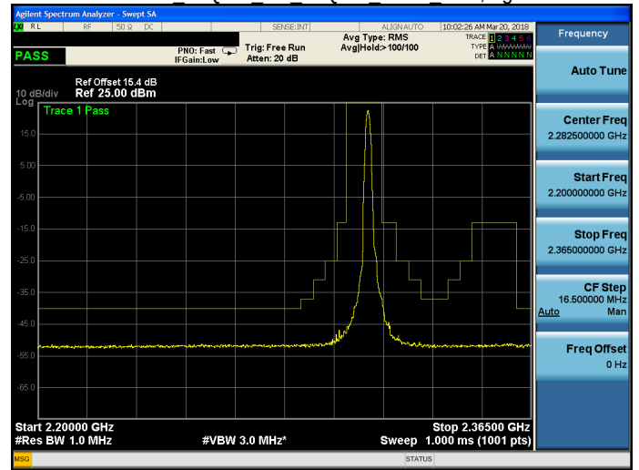
Band 30 16QAM 5M 16QAM HIGH RB1,24.gif
