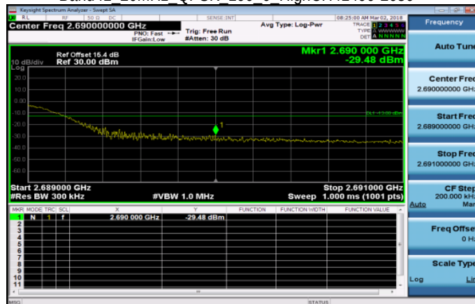
Band41 20MHz QPSK 100 0 HighCH41490-2680
