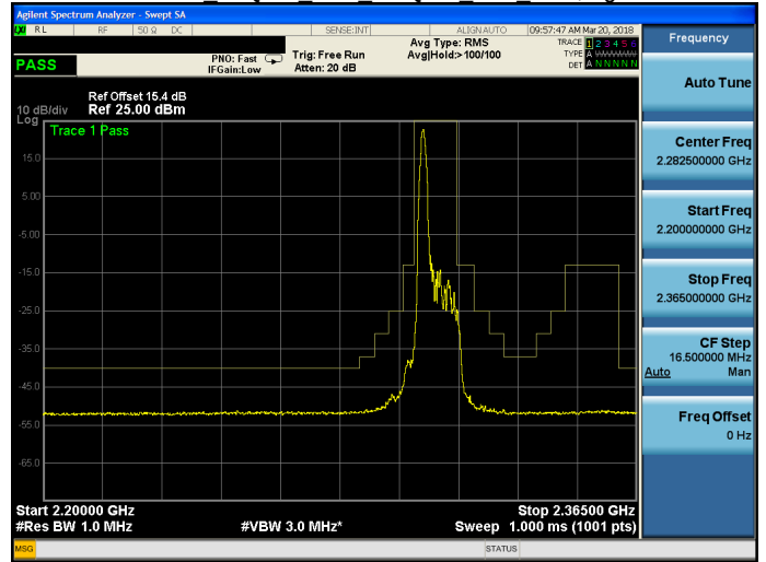
Band 30 16QAM 10M 16QAM MID RB1,49.gif
