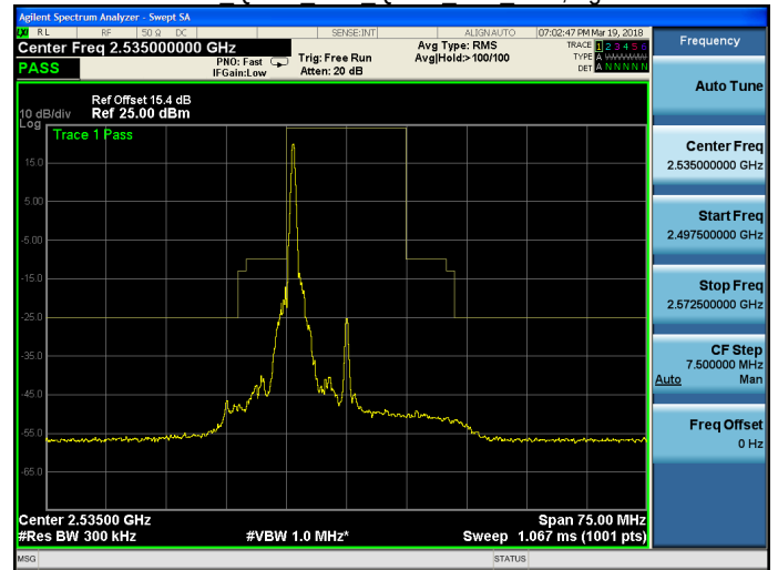
Band 7 QPSK 15M QPSK MID RB1,74.gif
