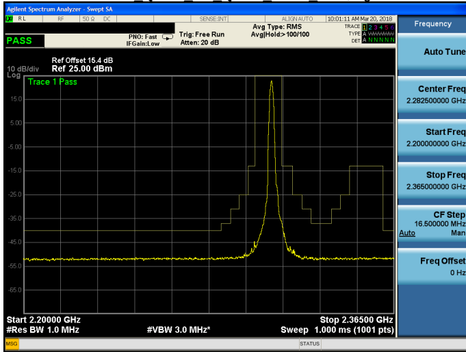
Band 30 QPSK 5M QPSK HIGH RB1,24.gif
