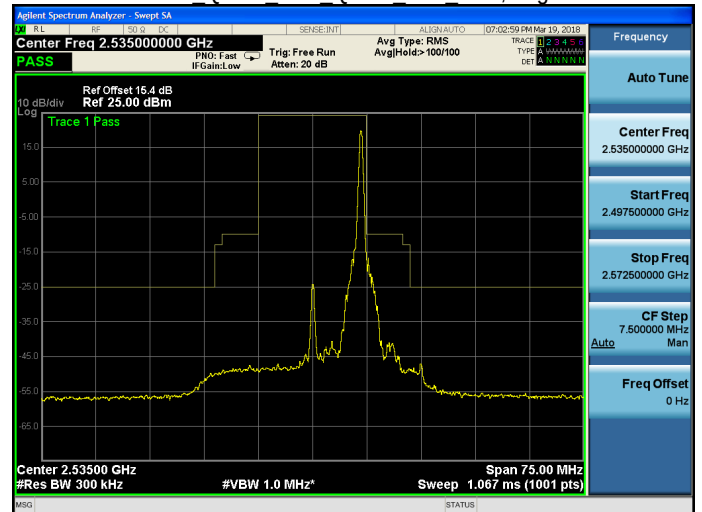
Band 7 QPSK 15M QPSK MID RB75,0.gif
