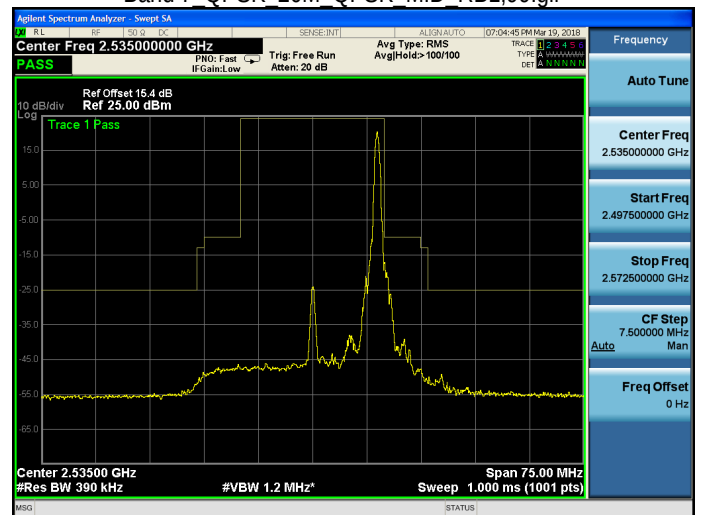
Band 7 QPSK 20M QPSK MID RB100,0.gif
