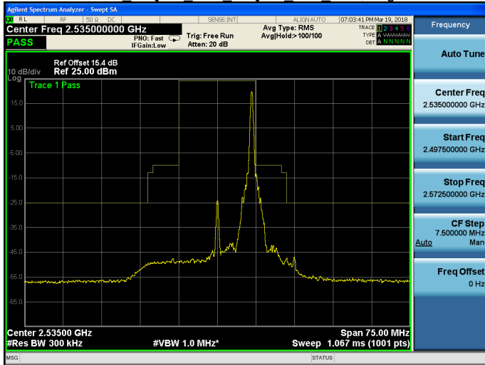
Band 7 16QAM 15M 16QAM MID RB75,0.gif
