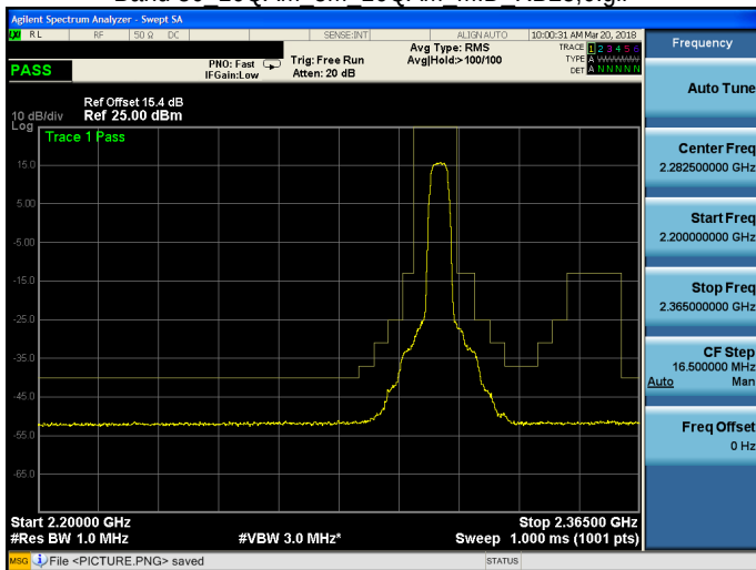
Band 30 16QAM 5M 16QAM MID RB25,0.gif
