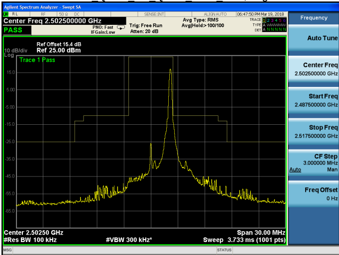
Band 7 QPSK 5M QPSK LOW RB25,0.gif
