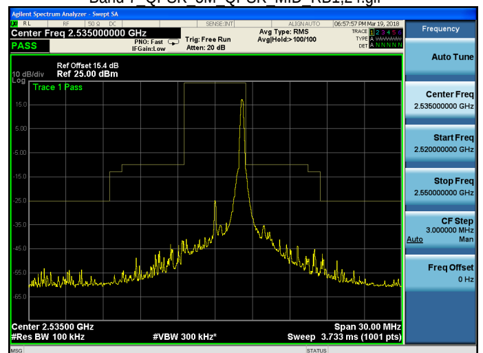
Band 7 QPSK 5M QPSK MID RB25,0.gif
