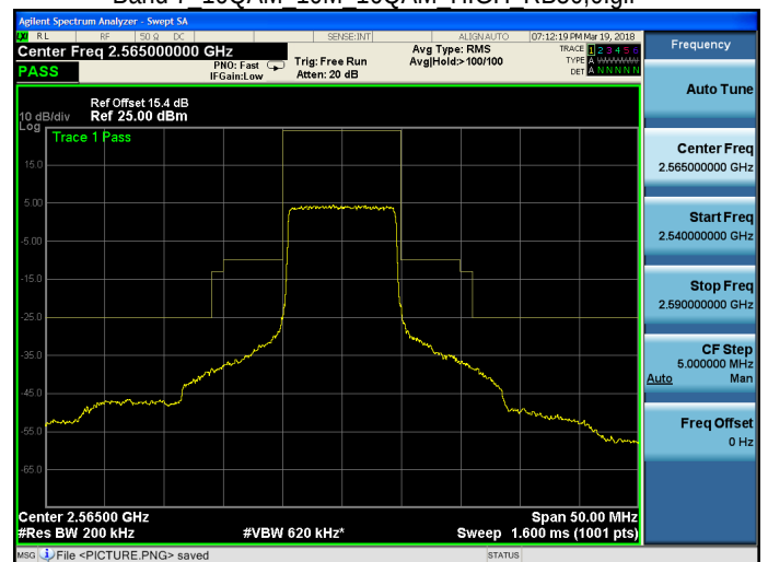
Band 7 16QAM 10M 16QAM HIGH RB50,0.gif
