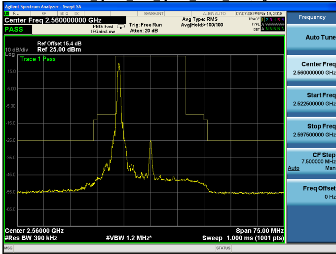
Band 7 QPSK 20M QPSK HIGH RB1,99.gif
