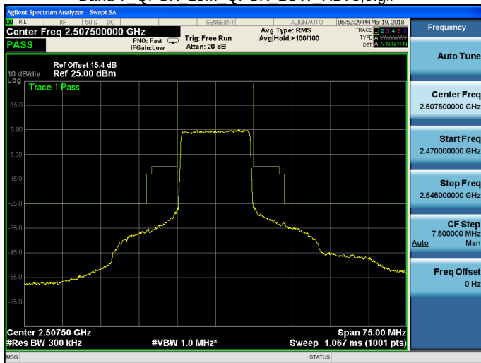
Band 7 QPSK 15M QPSK LOW RB75,0.gif
