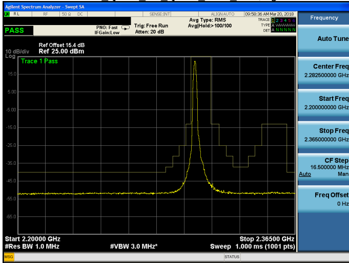
Band 30 QPSK 5M QPSK LOW RB1,24.gif
