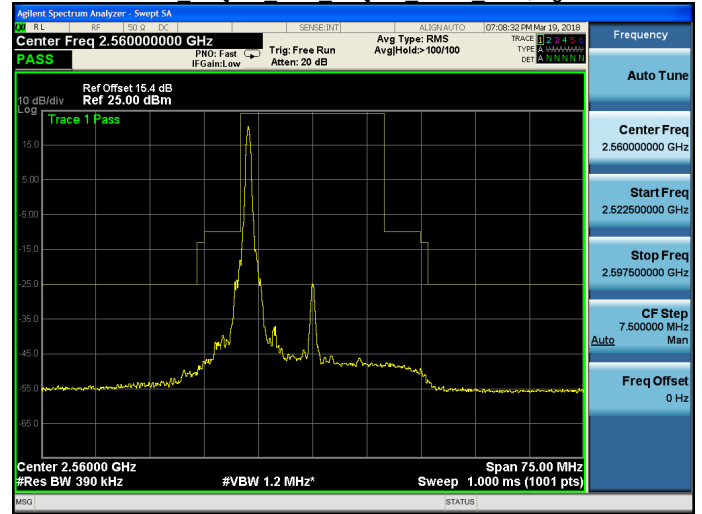
Band 7 16QAM 20M 16QAM HIGH RB1,99.gif
