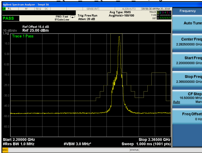
Band 30 QPSK 10M QPSK MID RB50,0.gif
