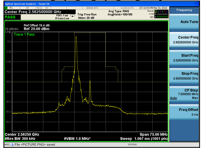
Band 7 16QAM 15M 16QAM HIGH RB1,74.gif
