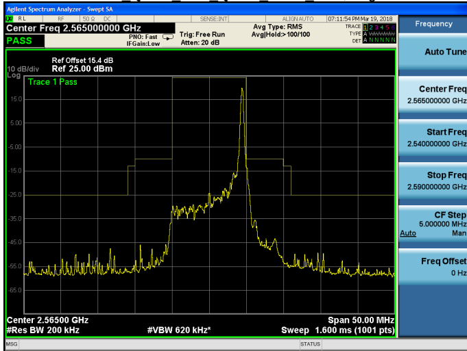
Band 7 QPSK 10M QPSK HIGH RB50,0.gif
