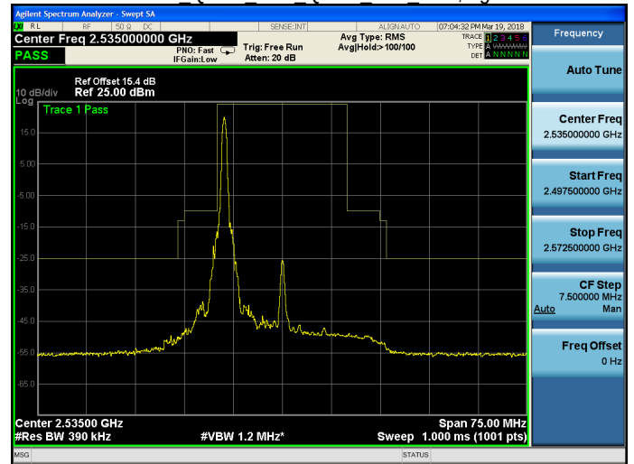
Band 7 QPSK 20M QPSK MID RB1,99.gif
