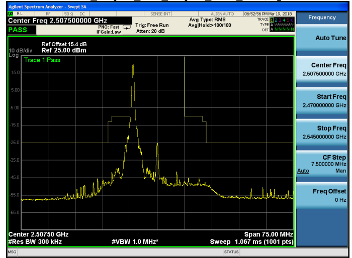
Band 7 16QAM 15M 16QAM LOW RB1,74.gif
