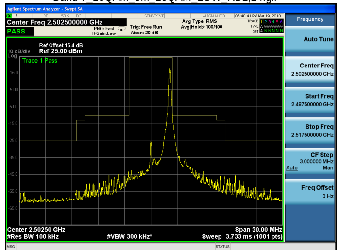
Band 7 16QAM 5M 16QAM LOW RB25,0.gif
