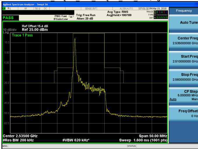
Band 7 16QAM 10M 16QAM MID RB1,49.gif
