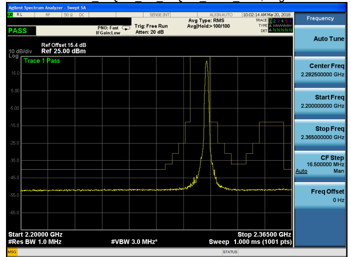
Band 30 16QAM 5M 16QAM HIGH RB25,0.gif
