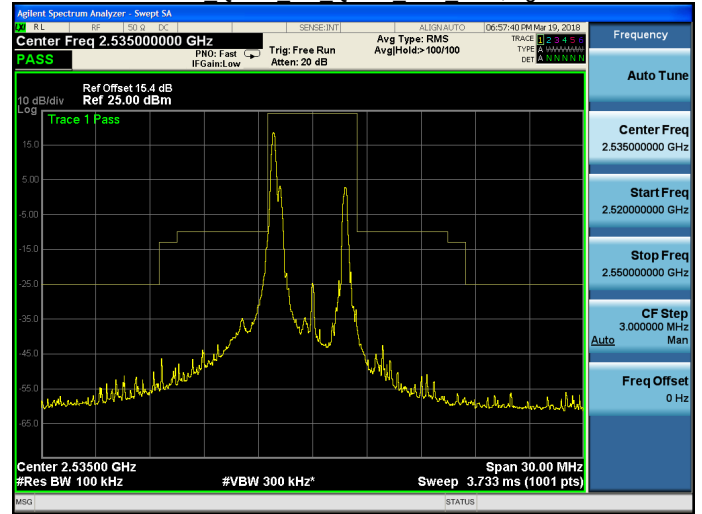
Band 7 QPSK 5M QPSK MID RB1,24.gif
