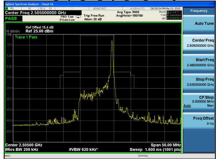
Band 7 16QAM 10M 16QAM LOW RB50,0.gif
