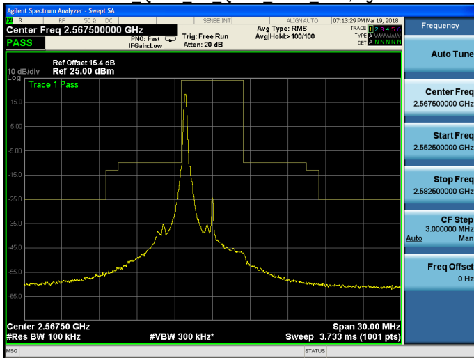
Band 7 QPSK 5M QPSK HIGH RB1,24.gif
