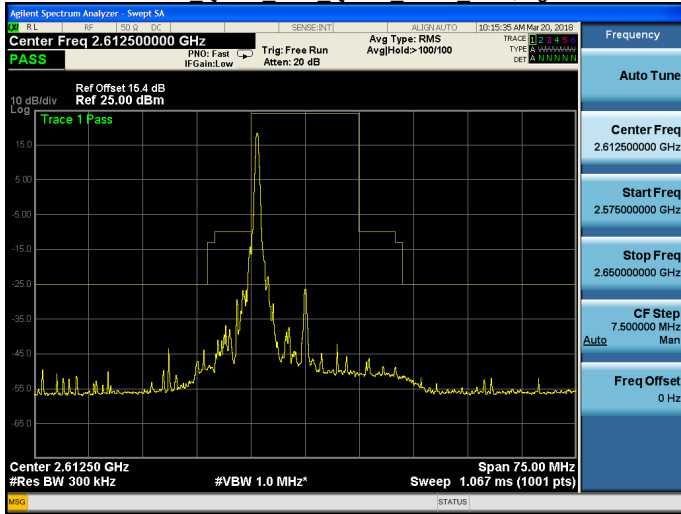
Band 38 QPSK 15M QPSK HIGH RB1,74.gif
