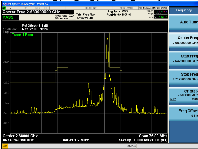
Band 41 QPSK 20M QPSK HIGH RB100,0.gif
