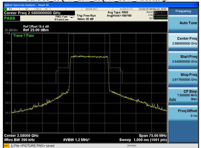
Band 38 16QAM 20M 16QAM LOW RB100,0.gif
