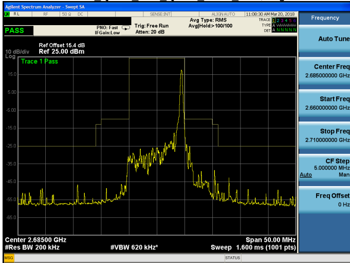
Band 41 QPSK 10M QPSK HIGH RB50,0.gif
