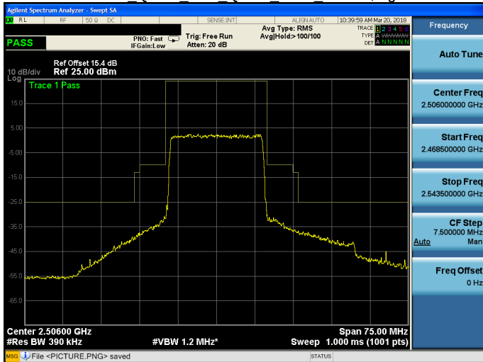
Band 41 QPSK 20M QPSK LOW RB100,0.gif
