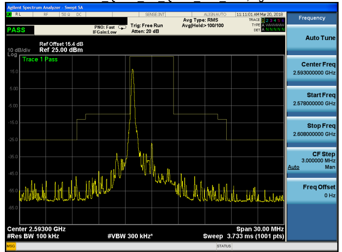
Band 41 QPSK 5M QPSK MID RB1,24.gif
