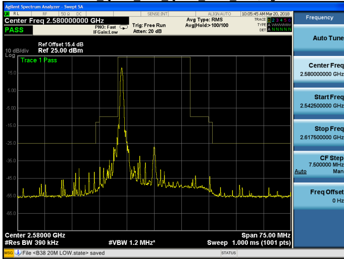
Band 38 QPSK 20M QPSK LOW RB1,99.gif
