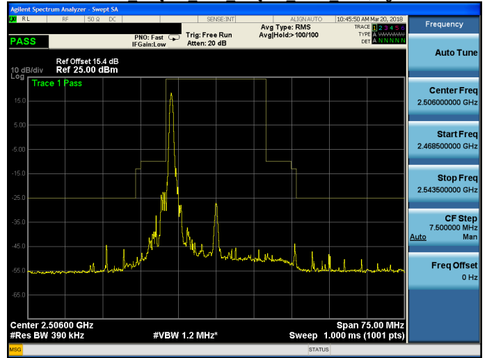
Band 41 16QAM 20M 16QAM LOW RB1,99.gif
