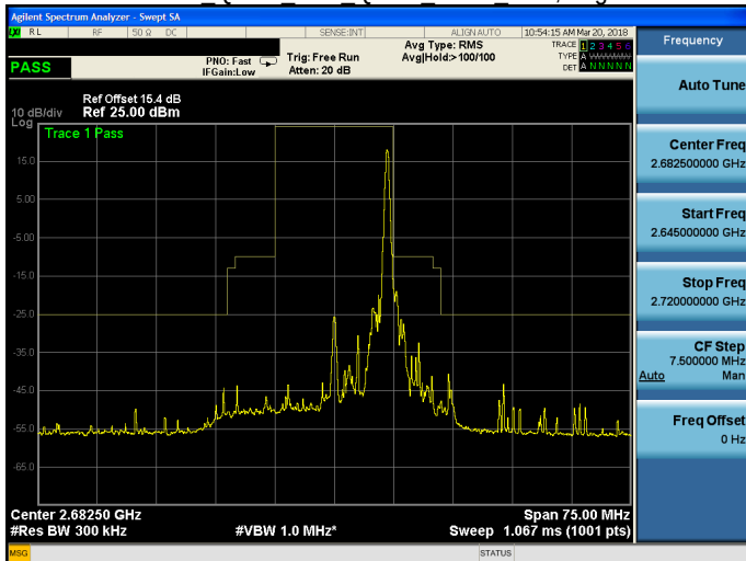
Band 41 QPSK 15M QPSK HIGH RB75,0.gif
