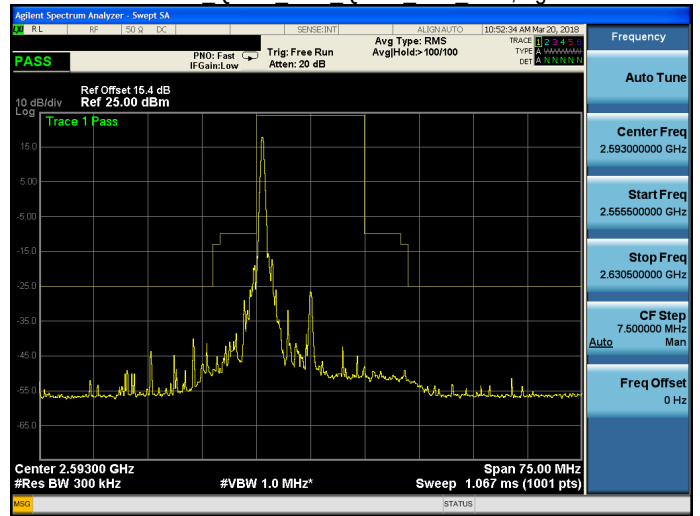
Band 41 QPSK 15M QPSK MID RB1,74.gif
