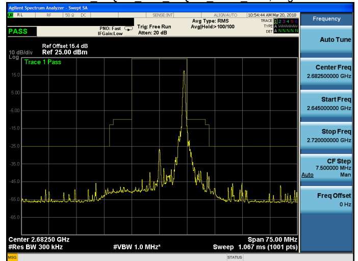
Band 41 16QAM 15M 16QAM HIGH RB75,0.gif
