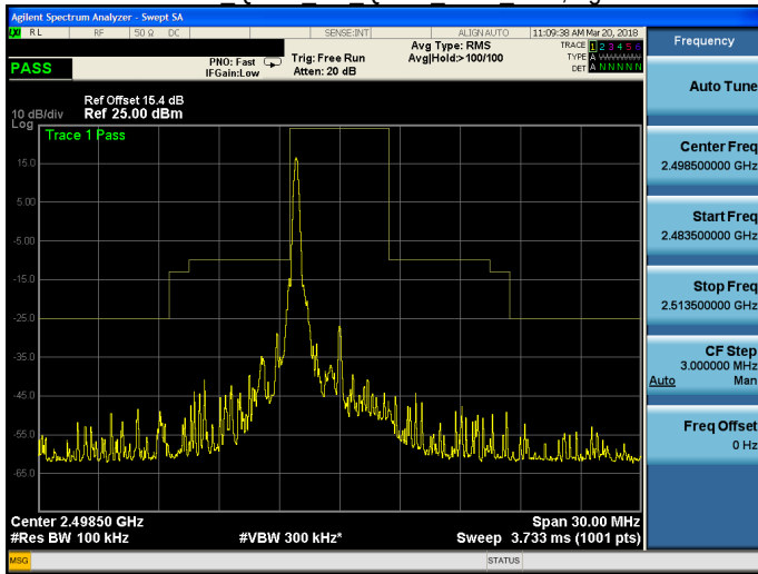
Band 41 QPSK 5M QPSK LOW RB1,24.gif
