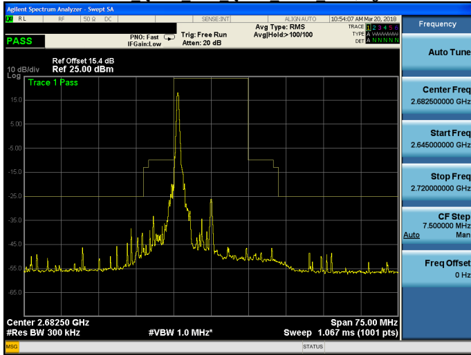
Band 41 QPSK 15M QPSK HIGH RB1,74.gif
