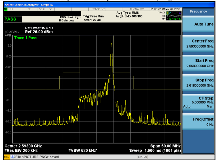
Band 41 QPSK 10M QPSK MID RB50,0.gif
