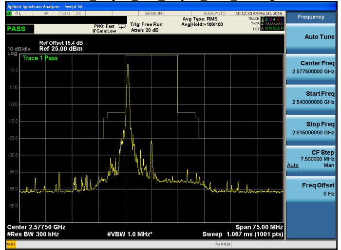
Band 38 16QAM 15M 16QAM LOW RB1,74.gif
