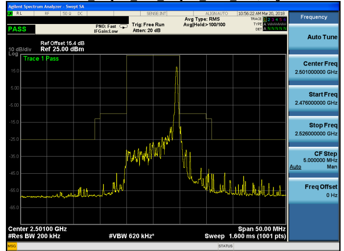
Band 41 16QAM 10M 16QAM LOW RB50,0.gif
