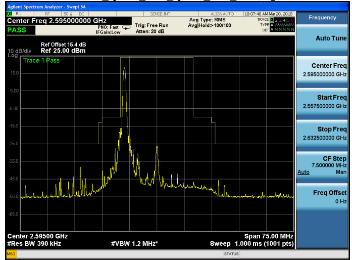
Band 38 QPSK 20M QPSK MID RB1,99.gif
