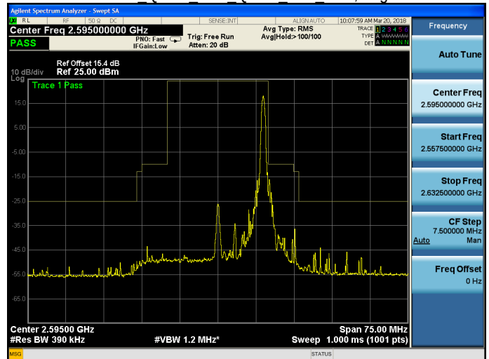
Band 38 QPSK 20M QPSK MID RB100,0.gif
