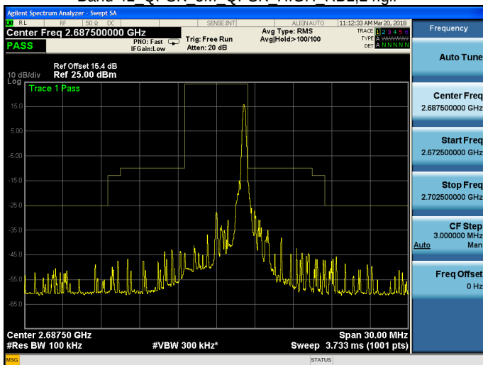
Band 41 QPSK 5M QPSK HIGH RB25,0.gif
