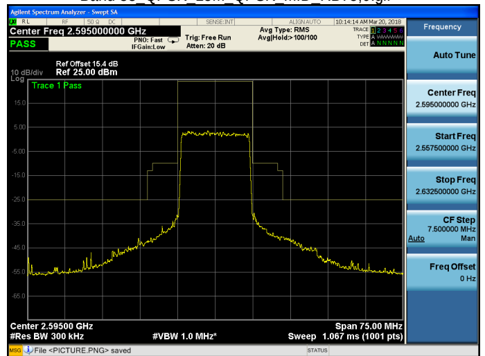
Band 38 QPSK 15M QPSK MID RB75,0.gif
