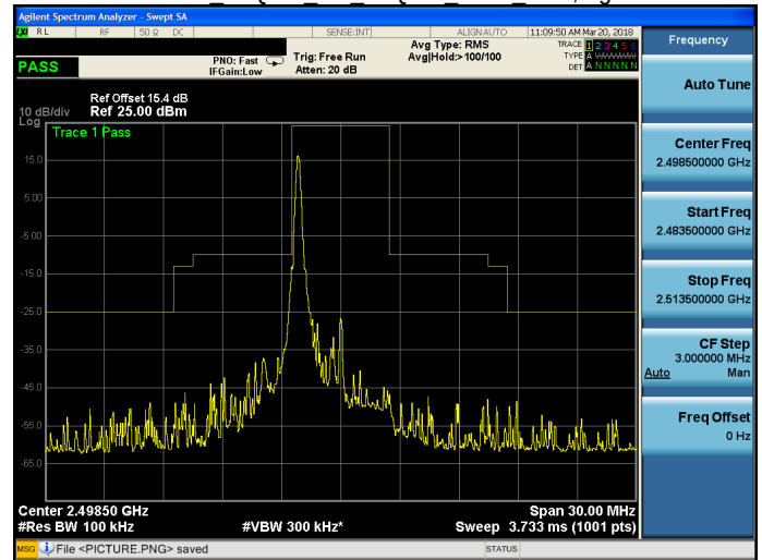
Band 41 16QAM 5M 16QAM LOW RB1,24.gif
