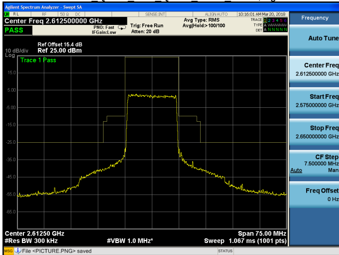
Band 38 QPSK 15M QPSK HIGH RB75,0.gif
