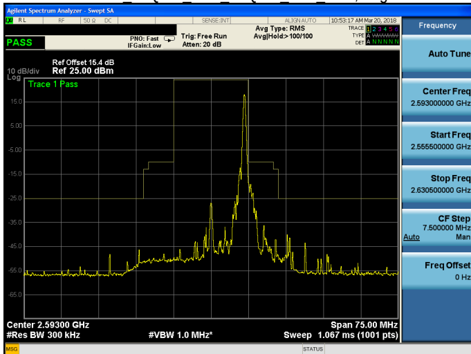
Band 41 16QAM 15M 16QAM MID RB75,0.gif
