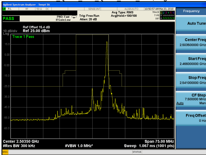
Band 41 QPSK 15M QPSK LOW RB75,0.gif
