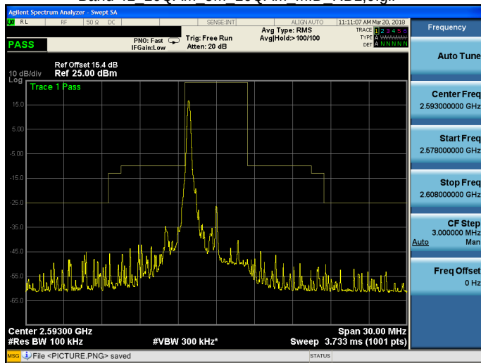
Band 41_16QAM_5M_16QAM_MID_RB1,24.gif
