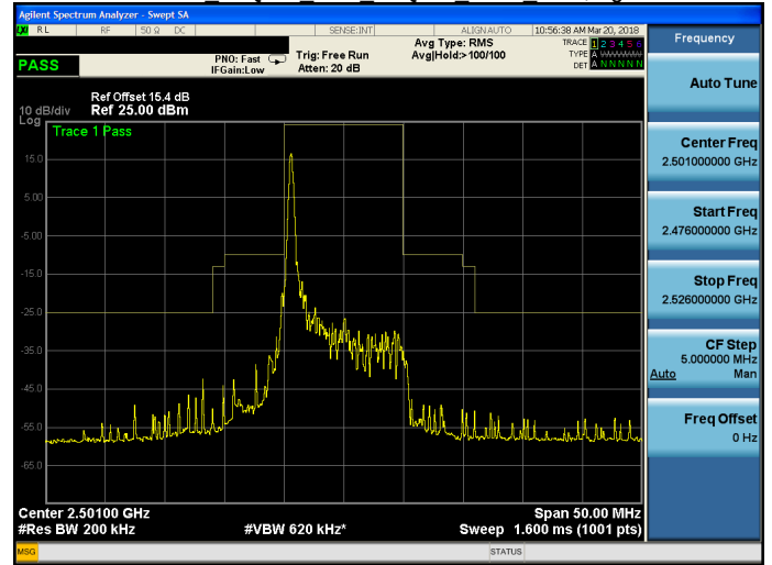
Band 41 16QAM 10M 16QAM LOW RB1,49.gif
