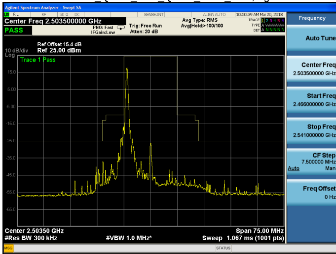
Band 41 QPSK 15M QPSK LOW RB1,74.gif
