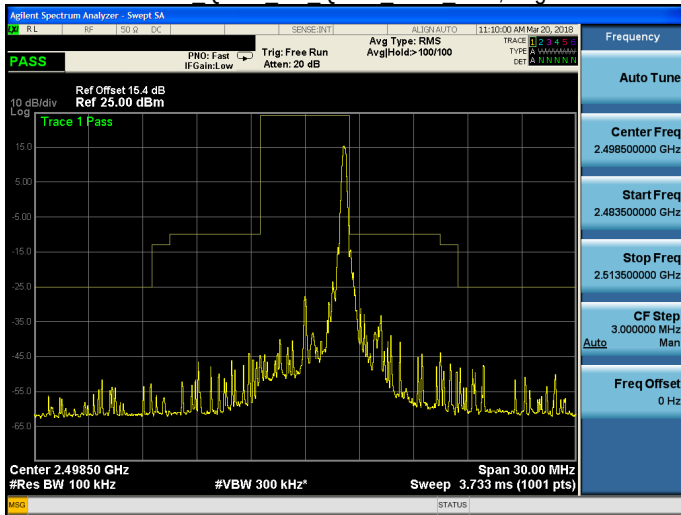
Band 41 QPSK 5M QPSK LOW RB25,0.gif
