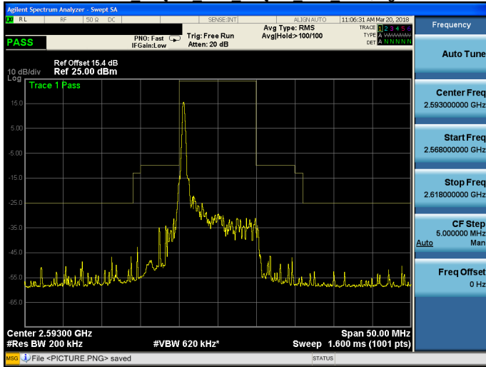
Band 41 16QAM 10M 16QAM MID RB1,49.gif
