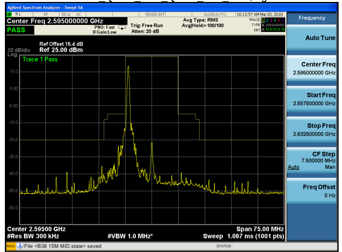
Band 38 QPSK 15M QPSK MID RB1,74.gif
