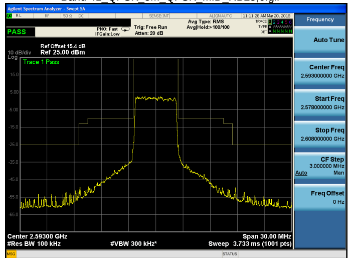
Band 41 QPSK 5M QPSK MID RB25,0.gif
