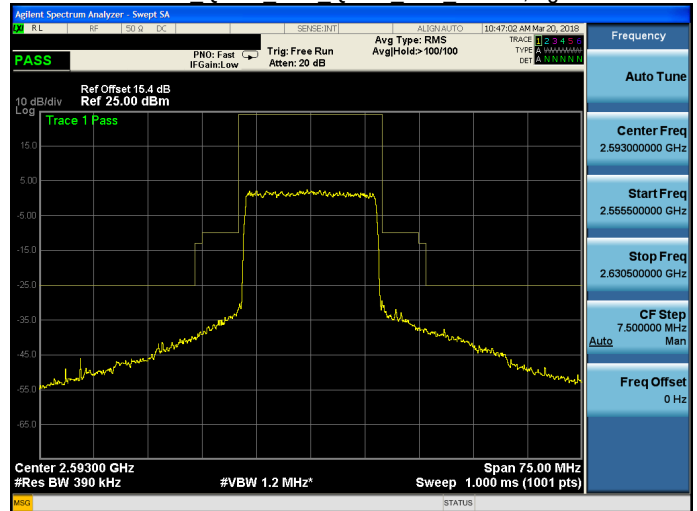
Band 41 QPSK 20M QPSK MID RB100,0.gif
