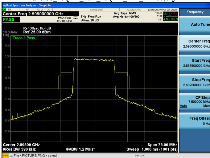
Band 38 16QAM 20M 16QAM MID RB100,0.gif
