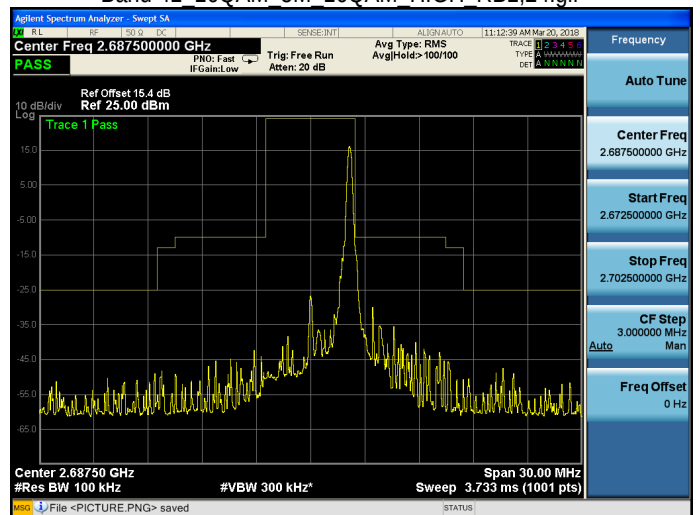
Band 41_16QAM_5M_16QAM_HIGH_RB25,0.gif
