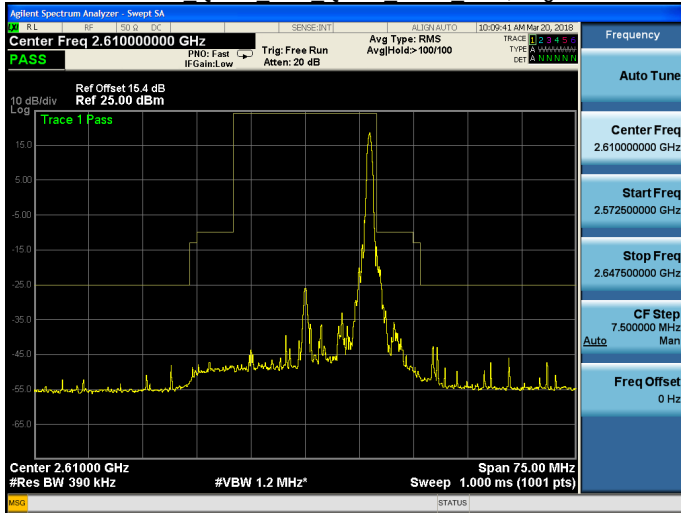
Band 38 QPSK 20M QPSK HIGH RB100,0.gif
