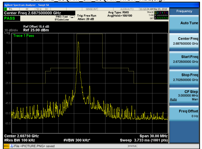
Band 41_16QAM_5M_16QAM_HIGH_RB1,24.gif
