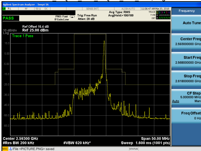
Band 41 16QAM 10M 16QAM MID RB50,0.gif
