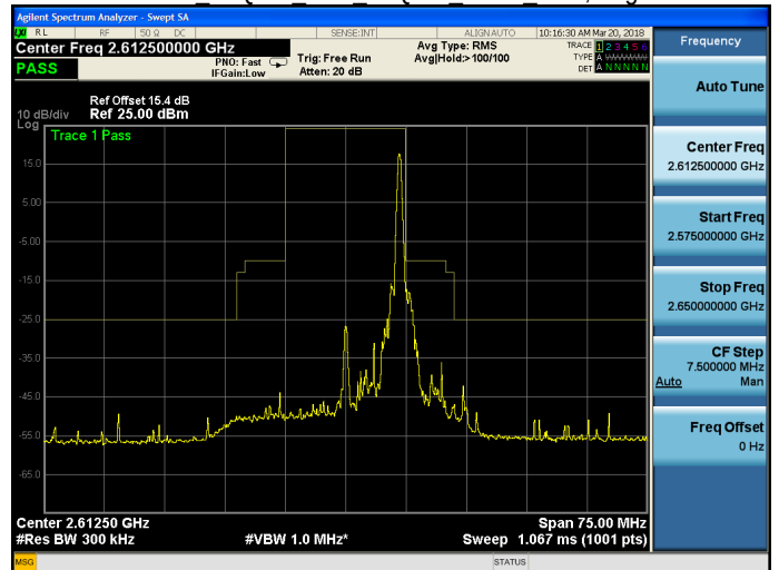
Band 38 16QAM 15M 16QAM HIGH RB75,0.gif
