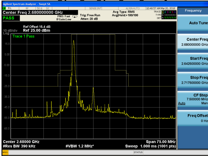
Band 41 QPSK 20M QPSK HIGH RB1,99.gif
