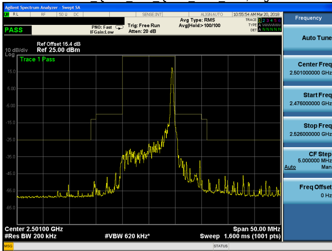
Band 41 QPSK 10M QPSK LOW RB50,0.gif
