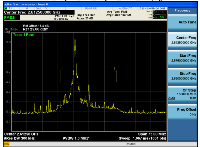
Band 38 16QAM 15M 16QAM HIGH RB1,74.gif
