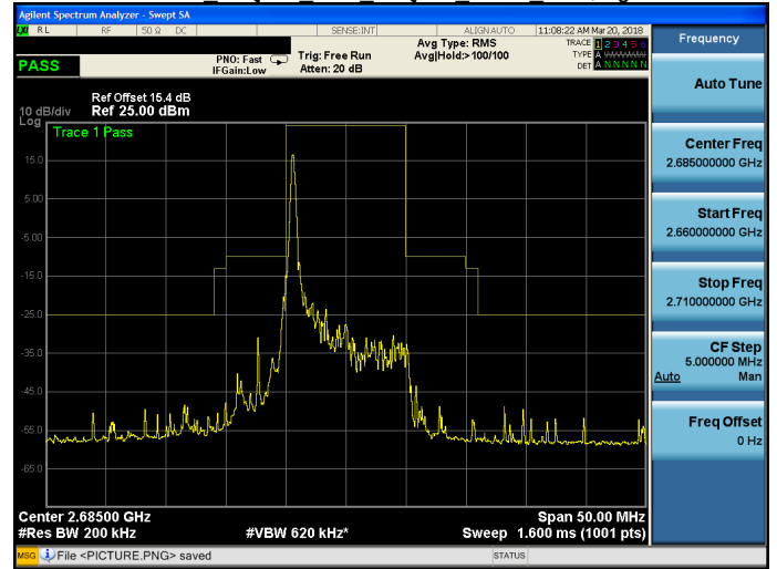
Band 41 16QAM 10M 16QAM HIGH RB1,49.gif
