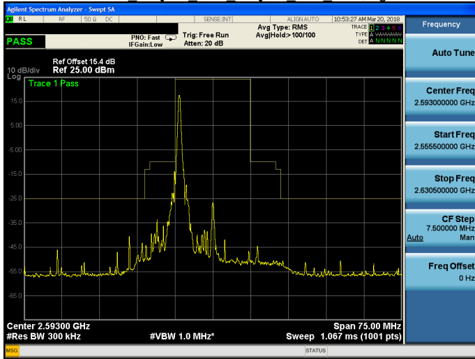
Band 41 16QAM 15M 16QAM MID RB1,74.gif
