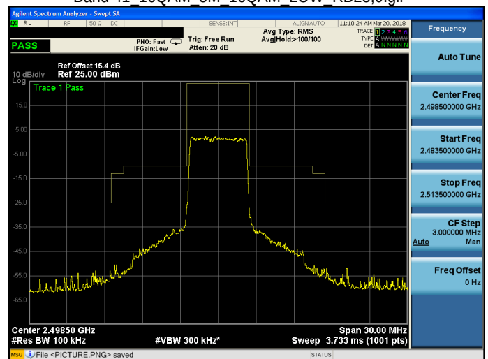
Band 41 16QAM 5M 16QAM LOW RB25,0.gif
