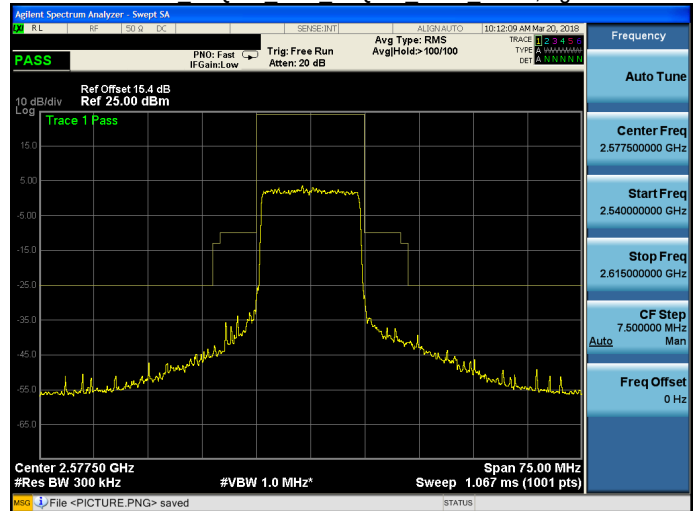
Band 38 16QAM 15M 16QAM LOW RB75,0.gif
