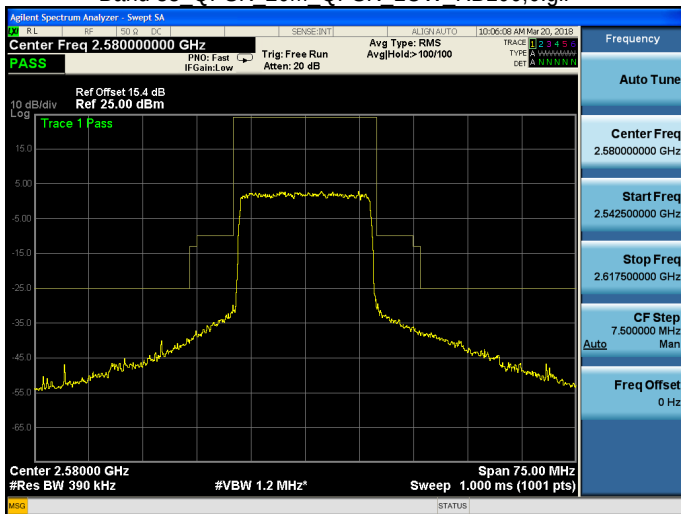
Band 38 QPSK 20M QPSK LOW RB100,0.gif
