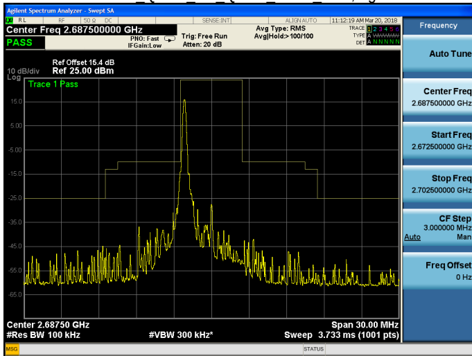
Band 41 QPSK 5M QPSK HIGH RB1,24.gif
