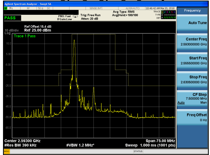
Band 41 QPSK 20M QPSK MID RB1,99.gif
