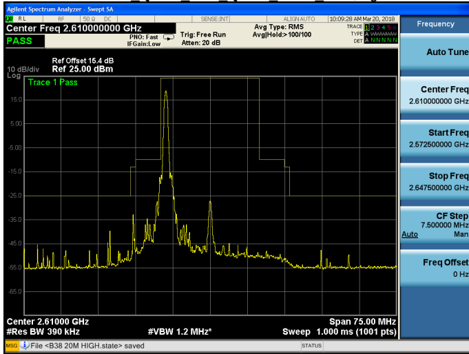
Band 38 QPSK 20M QPSK HIGH RB1,99.gif
