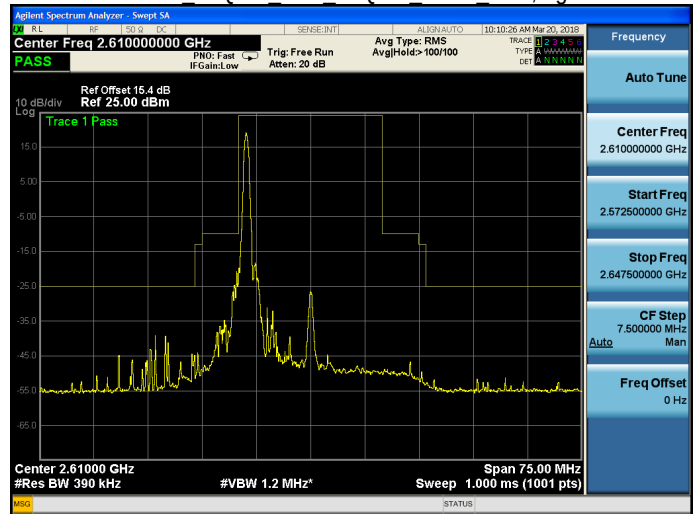
Band 38 16QAM 20M 16QAM HIGH RB1,99.gif
