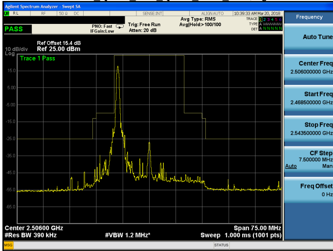
Band 41 QPSK 20M QPSK LOW RB1,99.gif
