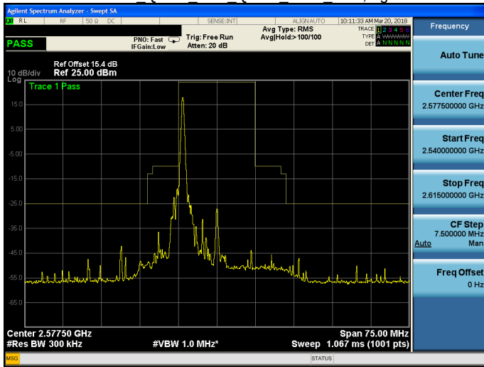
Band 38 QPSK 15M QPSK LOW RB1,74.gif
