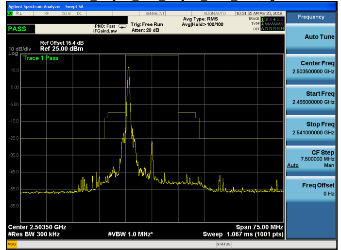
Band 41 16QAM 15M 16QAM LOW RB1,74.gif
