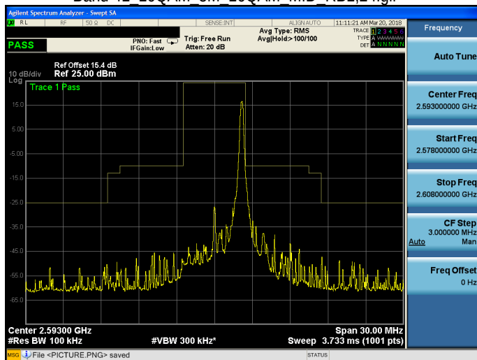
Band 41_16QAM_5M_16QAM_MID_RB25,0.gif
