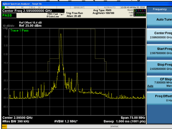
Band 38 16QAM 20M 16QAM MID RB1,99.gif
