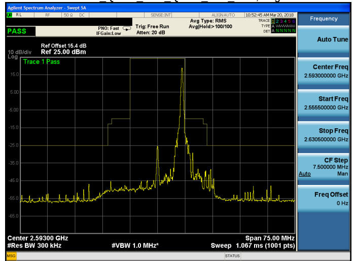
Band 41 QPSK 15M QPSK MID RB75,0.gif
