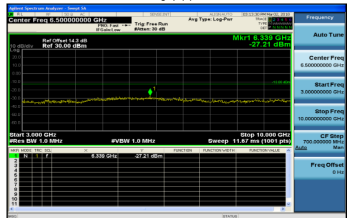
3GHz~10GHz_Band12_10MHz_QPSK_1_0_HighCH2313 0-711
