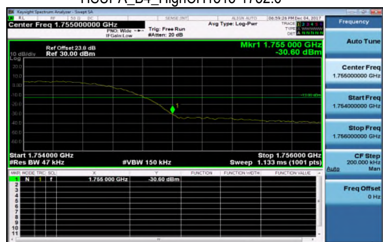
HSUPA_B4_HighCH1513-1752.6
