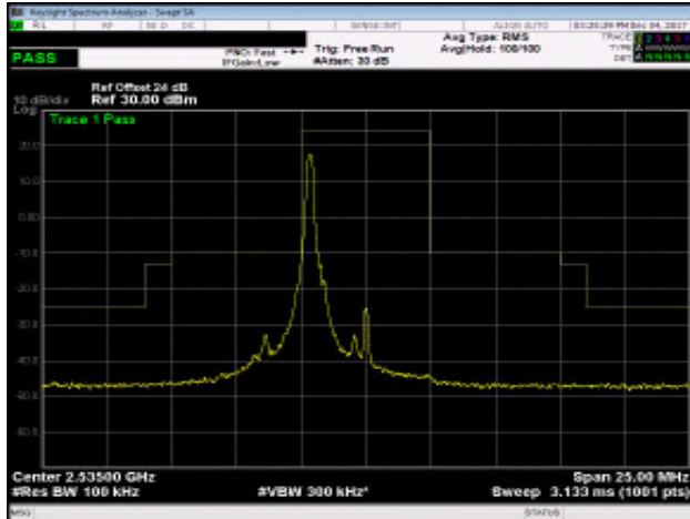
Band 7_5M_16QAM_MID_RB1,24
