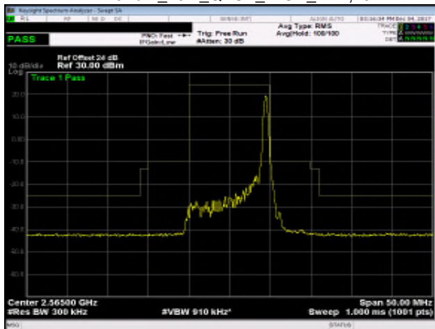
Band 7_10M_QPSK_HIGH_RB50,0
