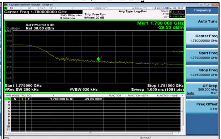
Band66_15MHz_QPSK_75_0_HighCH132597
