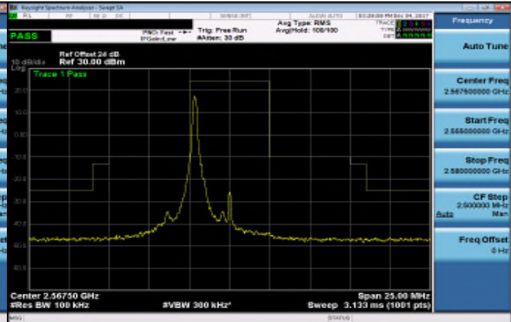
Band 7_5M_16QAM_HIGH_RB1,24
