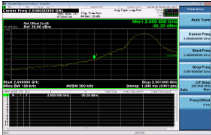
Band7_10MHz_QPSK_1_0_LowCH20800-2505
