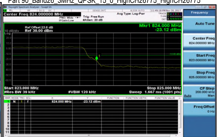
Part 90_Band26_3MHz_QPSK_15_0_HighCH26775_HighCH26775
