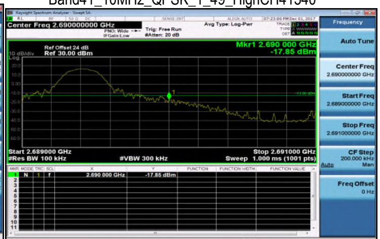
Band41_10MHz_QPSK_1_49_HighCH41540
