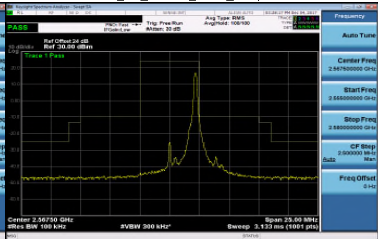
Band 7_5M_16QAM_HIGH_RB25,0
