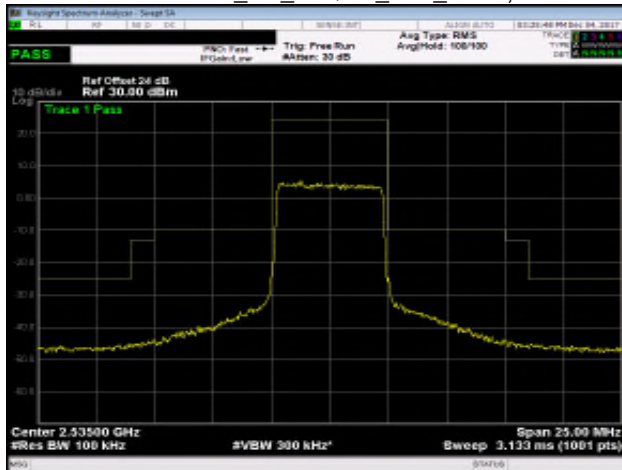
Band 7_5M_16QAM_MID_RB25,0
