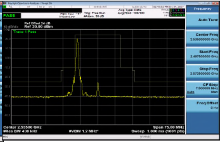
Band 7_20M_QPSK_MID_RB1,99
