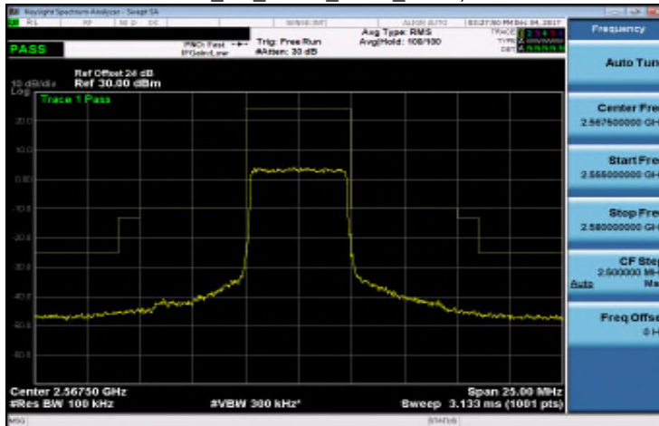
Band 7_5M_QPSK_HIGH_RB25,0
