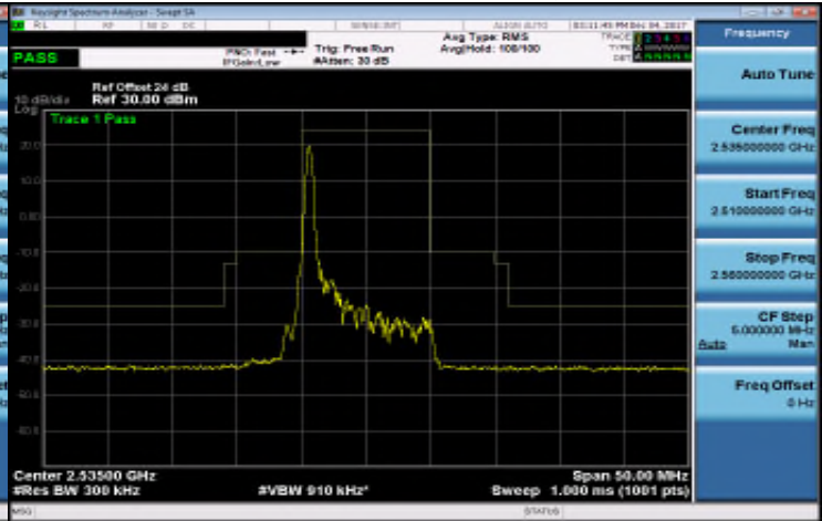
Band 7_10M_QPSK_MID_RB1,49
