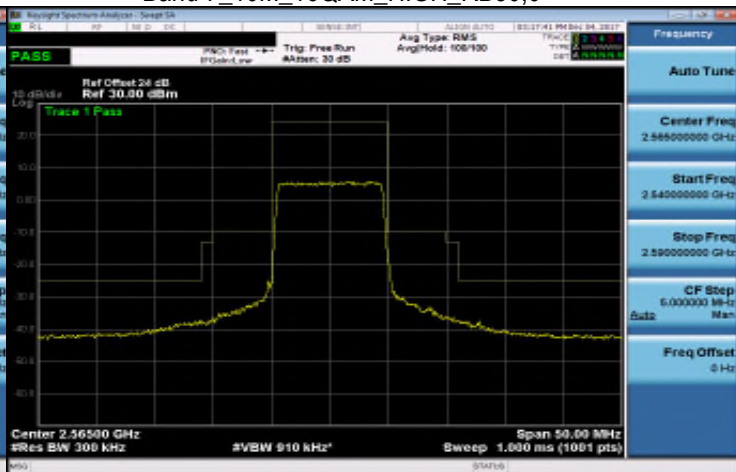
Band 7_10M_16QAM_HIGH_RB50,0
