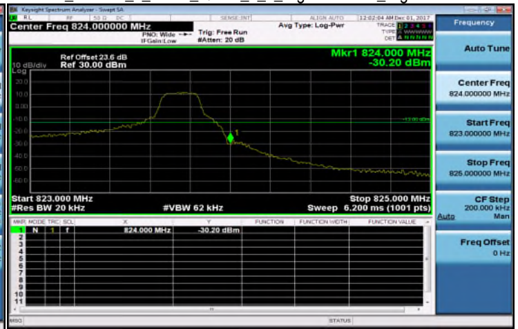
Part 90_Band26_1_4MHz_QPSK_1_5_HighCH26783_HighCH26783
