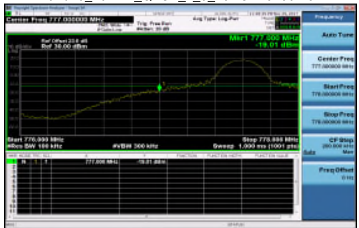
Band13_10MHz_QPSK_1_49_HighCH23230-782
