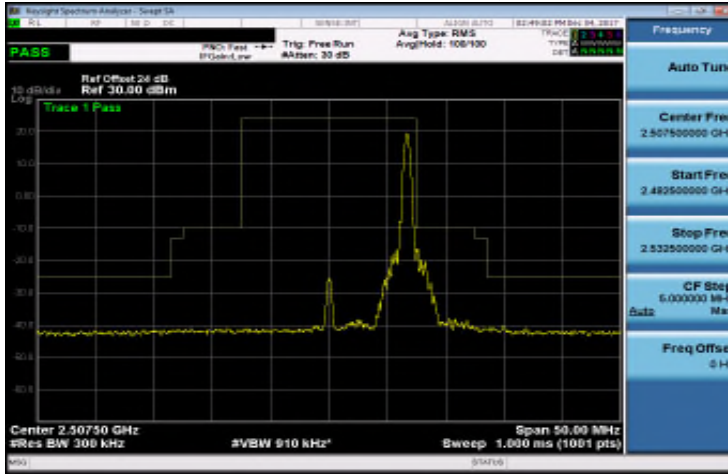
Band 7_15M_QPSK_LOW_RB75,0
