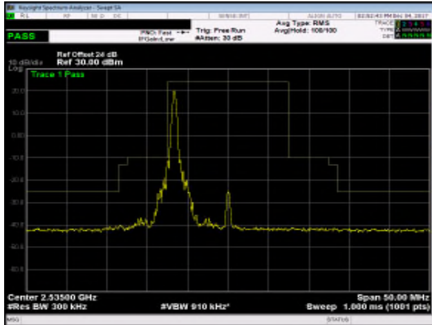
Band 7_15M_16QAM_MID_RB1,74
