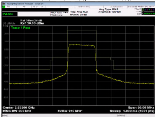
Band 7_10M_16QAM_MID_RB50,0
