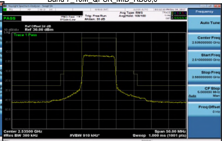
Band 7_10M_QPSK_MID_RB50,0
