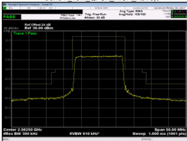
Band 7_15M_QPSK_HIGH_RB75,0
