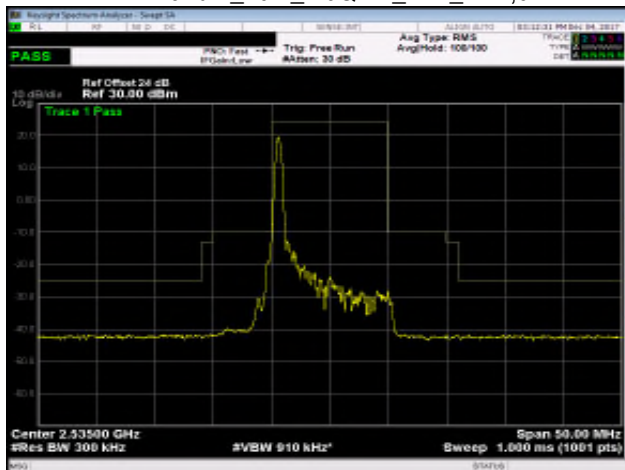
Band 7_10M_16QAM_MID_RB1,49
