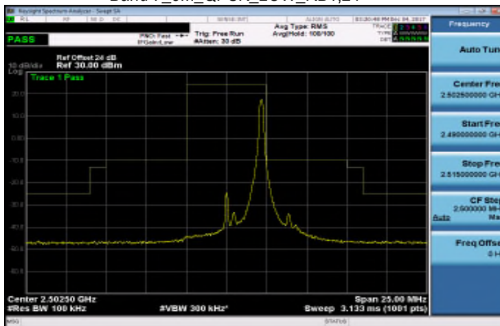
Band 7_5M_QPSK_LOW_RB25,0
