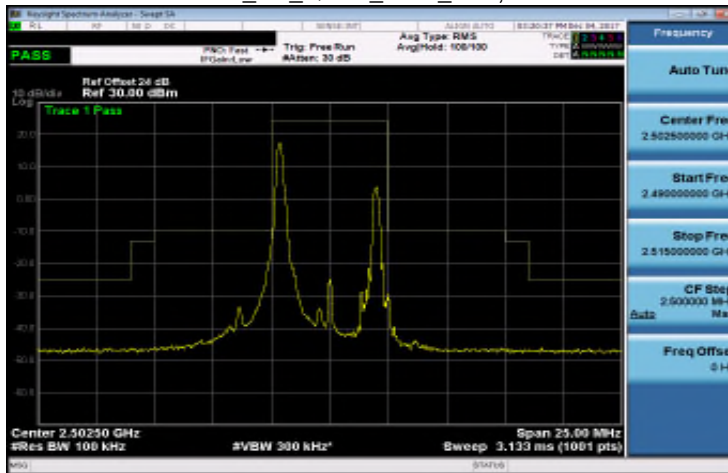
Band 7_5M_QPSK_LOW_RB1,24
