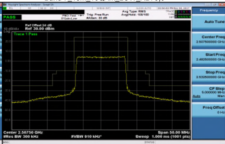
Band 7_15M_16QAM_LOW_RB75,0
