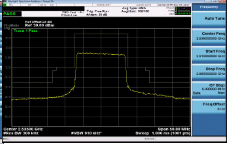
Band 7_15M_QPSK_MID_RB75,0
