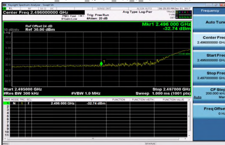
Band41_20MHz_QPSK_100_0_LowCH39750
