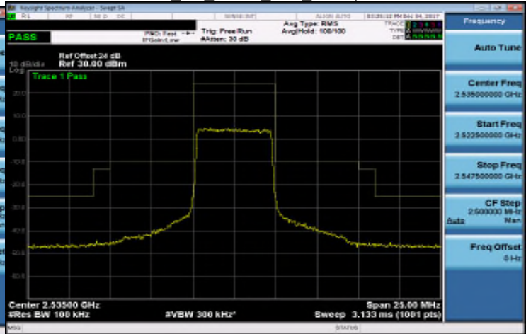
Band 7_5M_QPSK_MID_RB25,0
