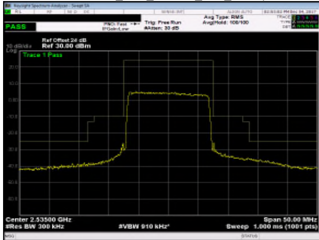
Band 7_15M_16QAM_MID_RB75,0
