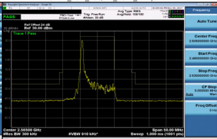
Band 7_10M_16QAM_LOW_RB1,49
