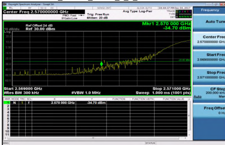
Band38_20MHz_QPSK_1_0_LowCH37850
