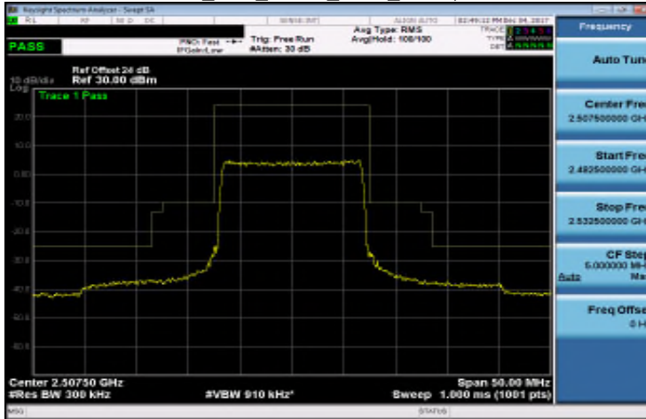
Band 7_15M_QPSK_LOW_RB75,0
