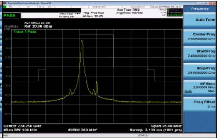
Band 7_5M_16QAM_LOW_RB1,24
