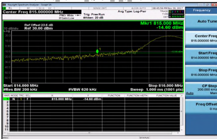
Band26_15MHz_QPSK_1_0_LowCH26775
