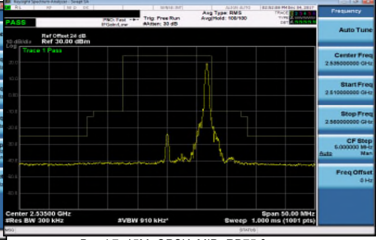
Band 7_15M_QPSK_MID_RB75,0
