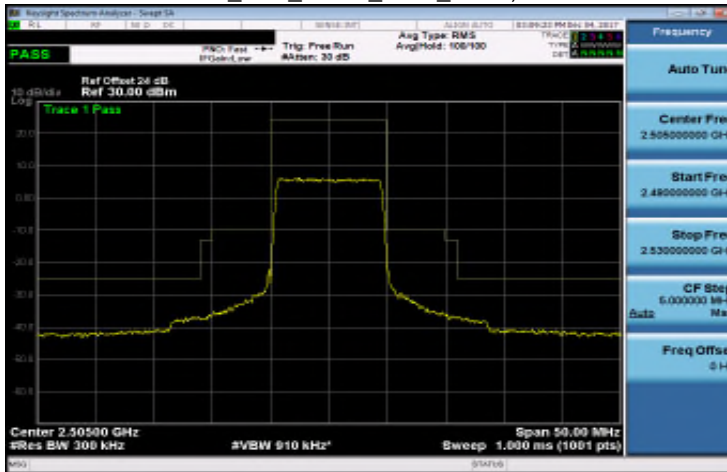
Band 7_10M_QPSK_LOW_RB50,0
