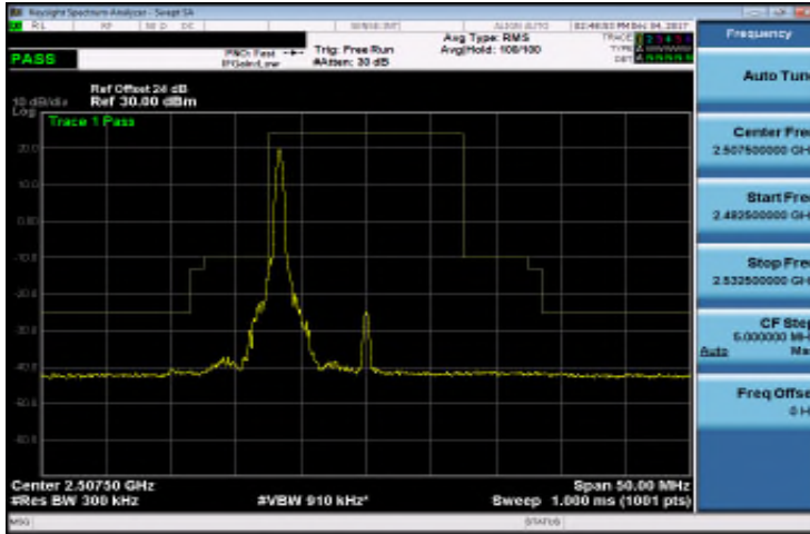
Band 7_15M_QPSK_LOW_RB1,74
