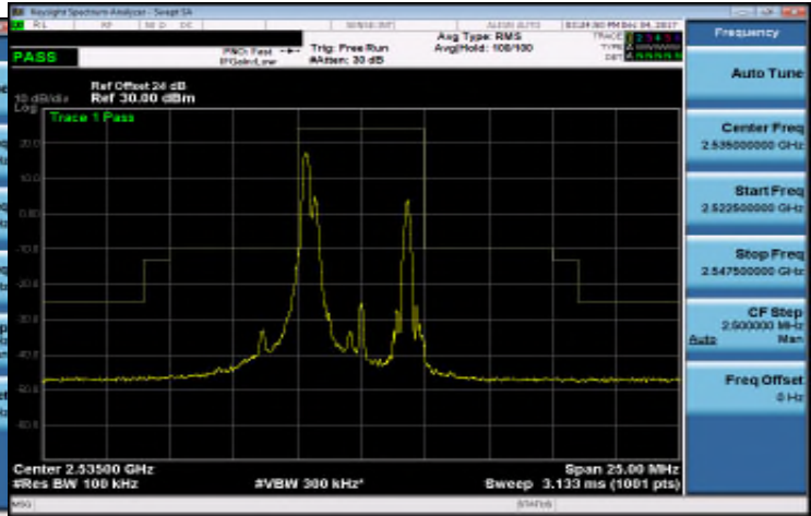
Band 7_5M_QPSK_MID_RB1,24
