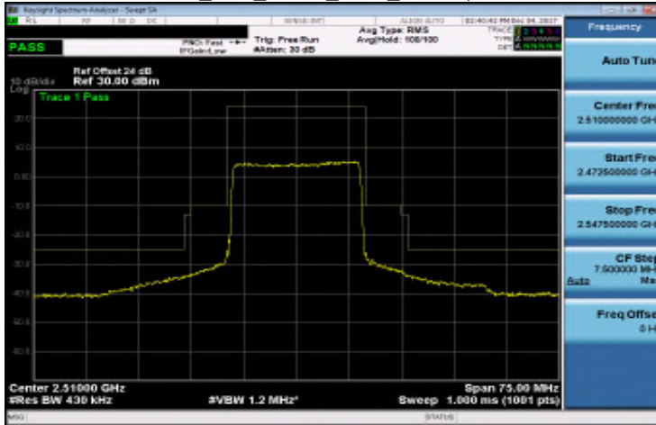
Band 7_20M_QPSK_LOW_RB100,0
