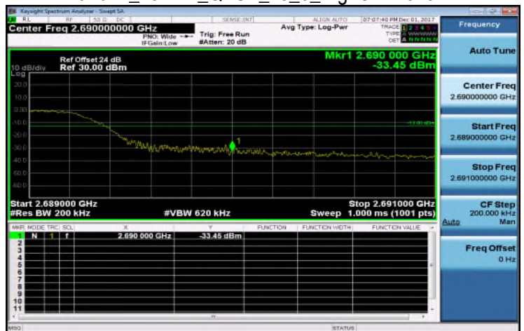
Band41_15MHz_QPSK_75_0_HighCH41515
