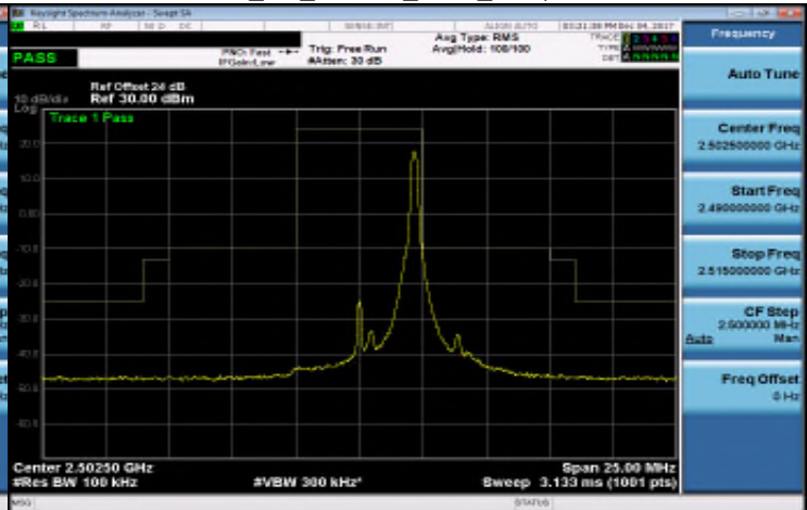
Band 7_5M_16QAM_LOW_RB25,0
