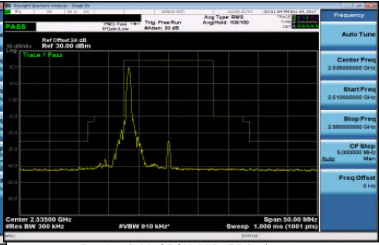
Band 7_15M_QPSK_MID_RB1,74
