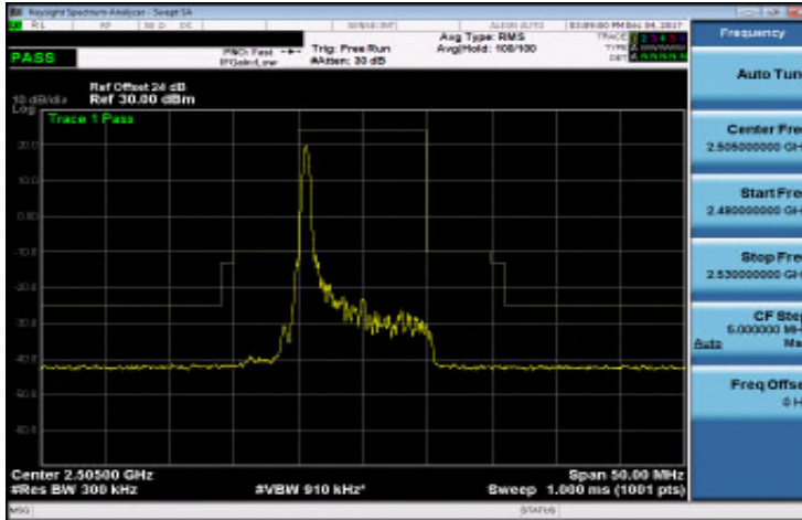
Band 7_10M_QPSK_LOW_RB1,49
