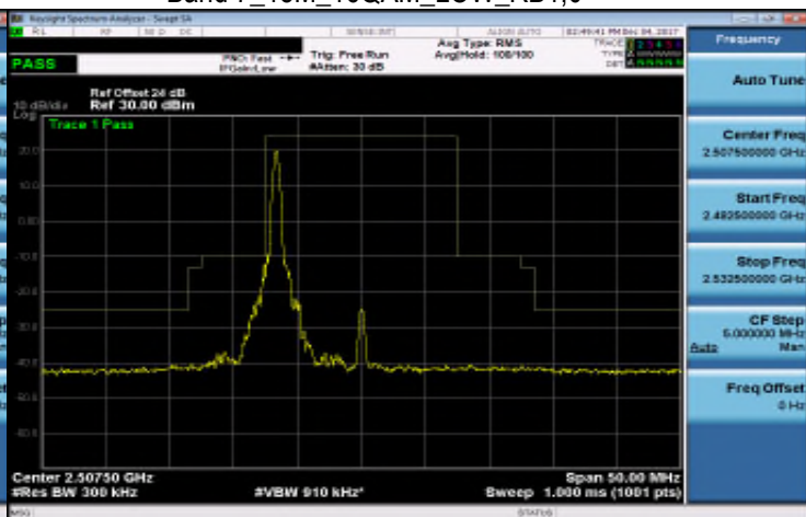
Band 7_15M_16QAM_LOW_RB1,74
