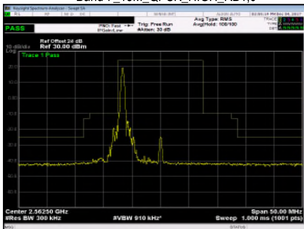
Band 7_15M_QPSK_HIGH_RB1,74
