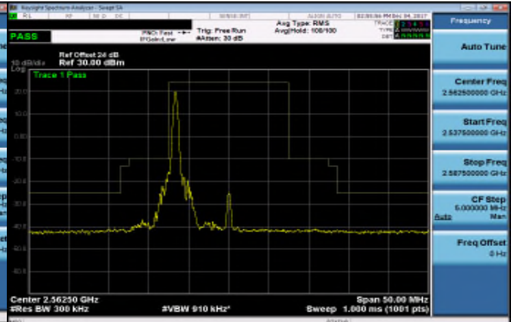
Band 7_15M_16QAM_HIGH_RB1,74
