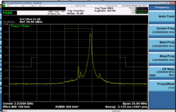
Band 7_5M_QPSK_MID_RB25,0
