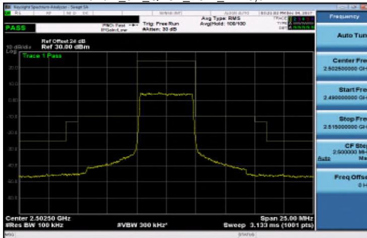
Band 7_5M_QPSK_LOW_RB25,0
