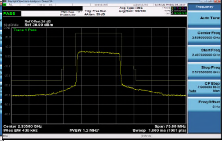
Band 7_20M_QPSK_MID_RB100,0
