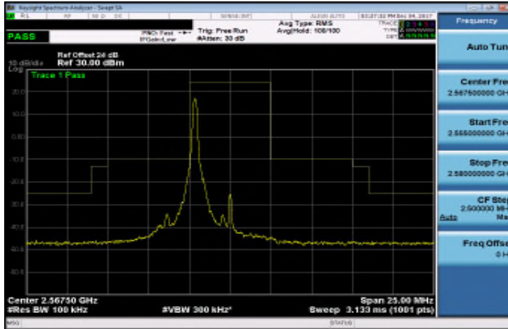
Band 7_5M_QPSK_HIGH_RB1,24
