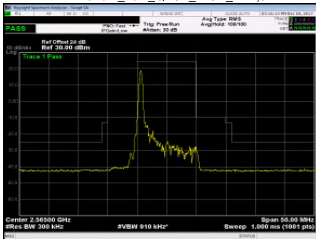
Band 7_10M_QPSK_HIGH_RB1,49
