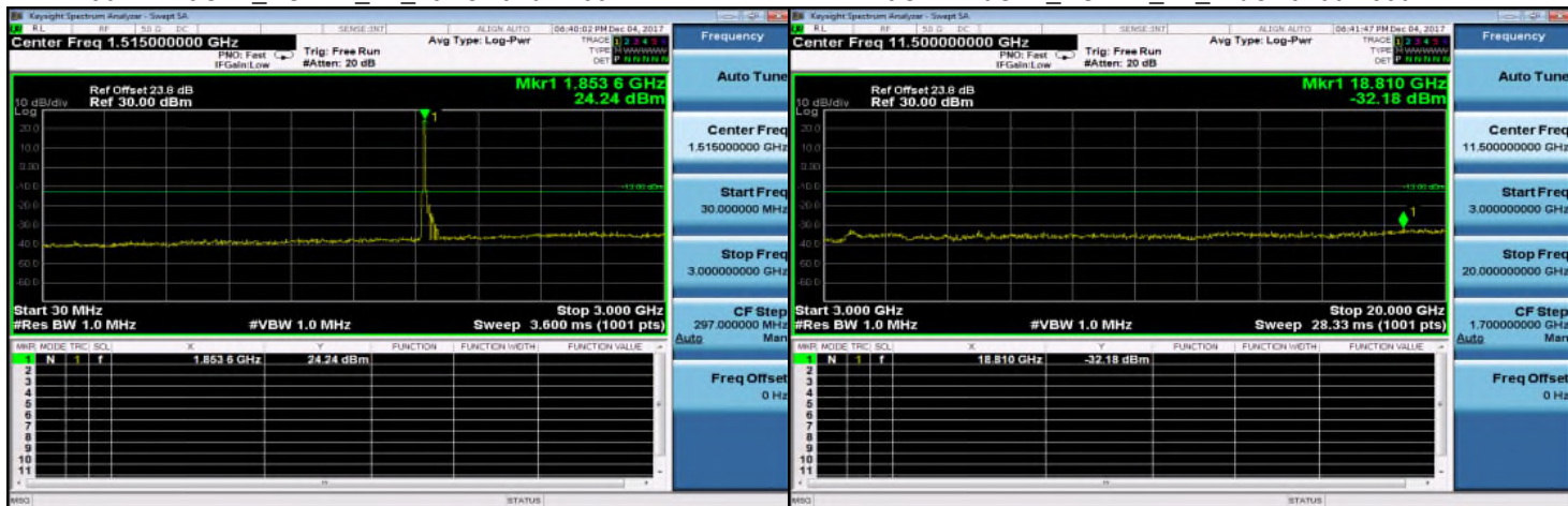
30MHz~3GHz_HSDPA_B2_LowCH9262-1852.4
