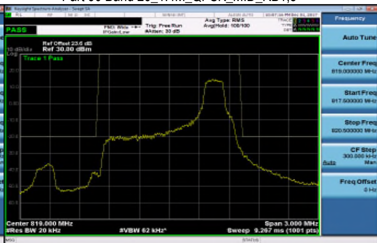
Part 90 Band 26_1.4M_QPSK_MID_RB6,0
