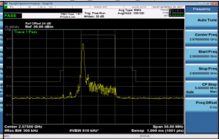
Band 38_10M_16QAM_LOW_RB1,49
