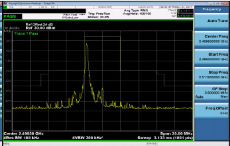
Band 41_5M_16QAM_LOW_RB1,24
