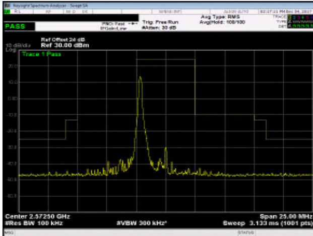
Band 38_5M_QPSK_LOW_RB1,24
