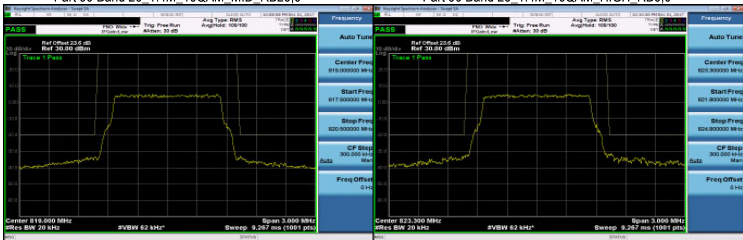
Part 90 Band 26_1.4M_16QAM_MID_RB26,0
