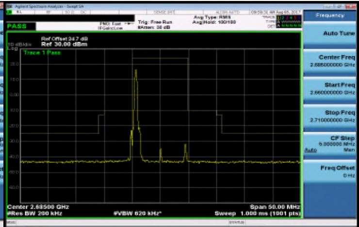
Band 41_10M_16QAM_HIGH_RB1,49
