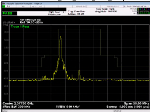
Band 38_15M_QPSK_LOW_RB1,74
