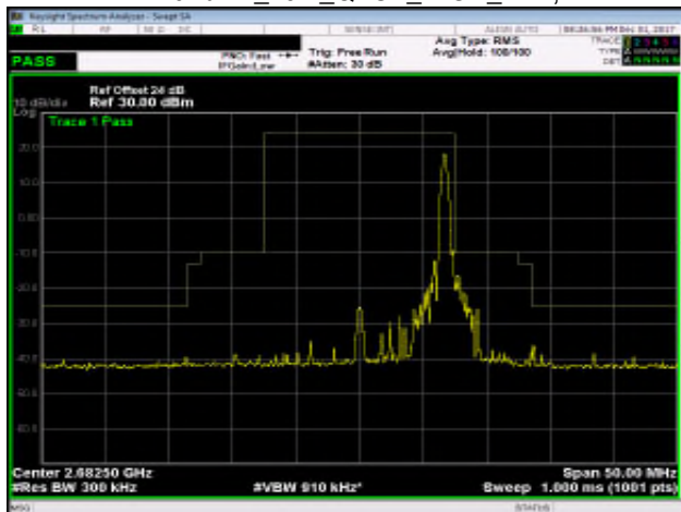
Band 41_15M_QPSK_HIGH_RB75,0
