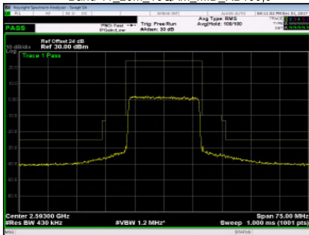
Band 41_20M_16QAM_MID_RB100,0
