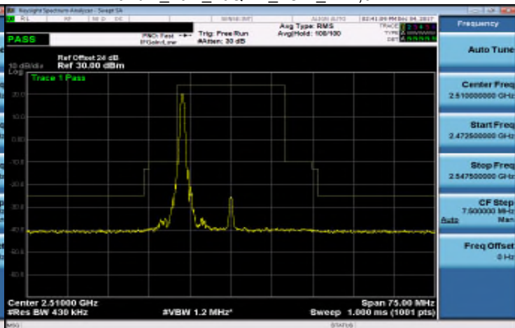
Band 7_20M_16QAM_LOW_RB1,99
