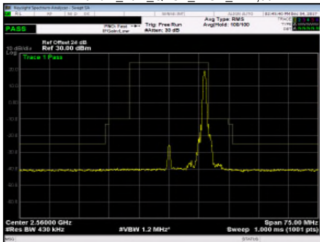
Band 7_20M_QPSK_HIGH_RB100,0
