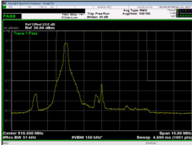
Part 90 Band 26_5M_QPSK_LOW_RB1,24
