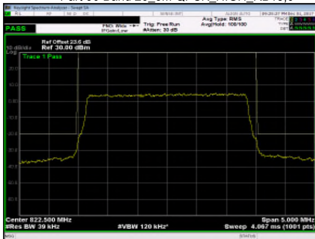
Part 90 Band 26_3M QPSK_HIGH_RB15,0
