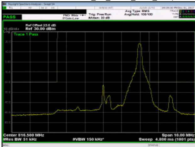
Part 90 Band 26_5M_QPSK_LOW_RB25,0
