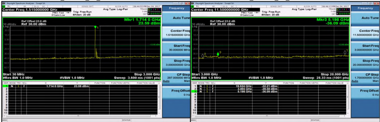
30MHz~3GHz_HSDPA_B4_LowCH1312-1712.4
