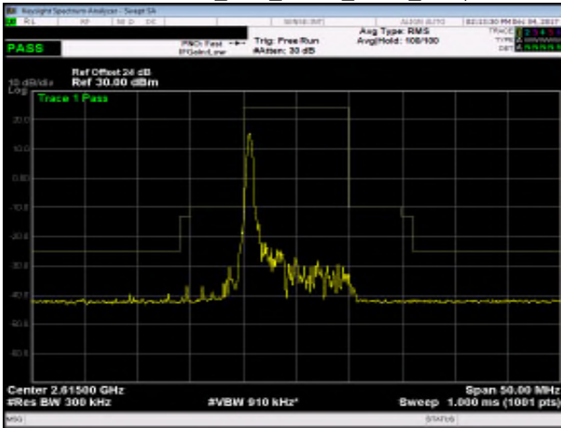
Band 38_10M_QPSK_HIGH_RB1,49
