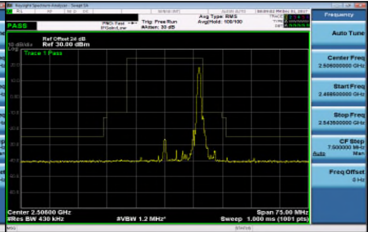
Band 41_20M_16QAM_LOW_RB100,0
