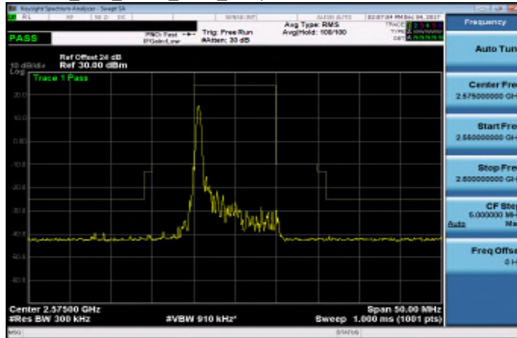
Band 38_10M_QPSK_LOW_RB1,49
