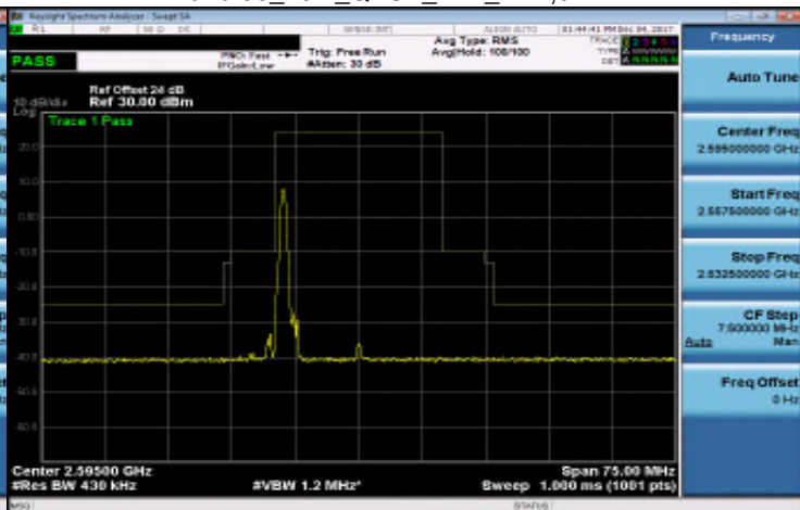
Band 38_20M_QPSK_MID_RB1,99
