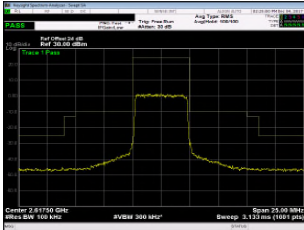
Band 38_5M_QPSK_HIGH_RB25,0
