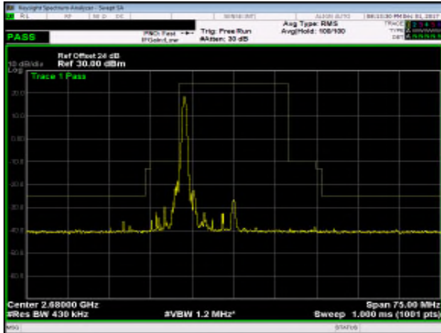
Band 41_20M_QPSK_HIGH_RB1,99
