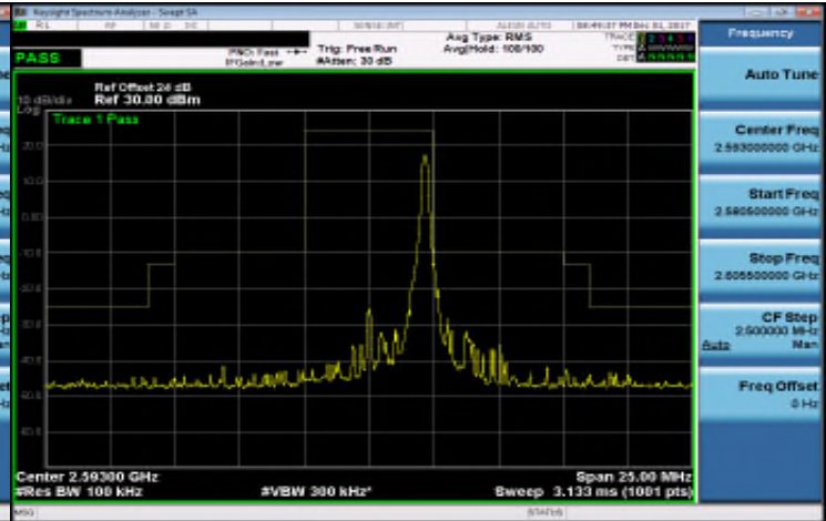
Band 41_5M_QPSK_MID_RB25,0
