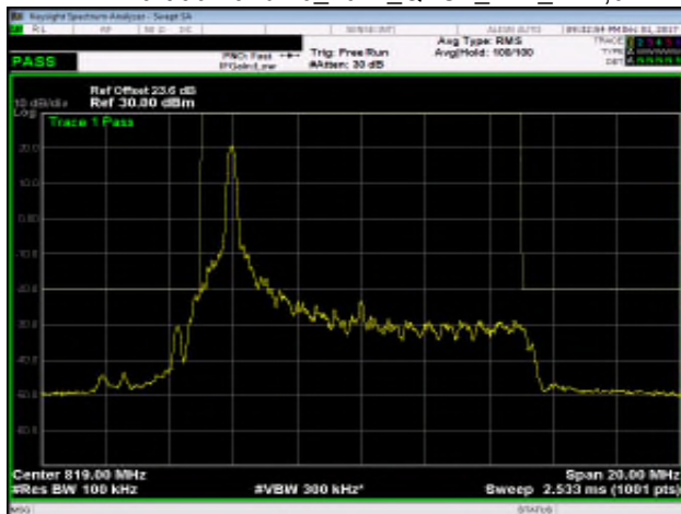
Part 90 Band 26_10M_QPSK_MID_RB1,49
