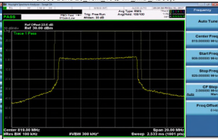
Part 90 Band 26_10M_16QAM_MID_RB50,0
