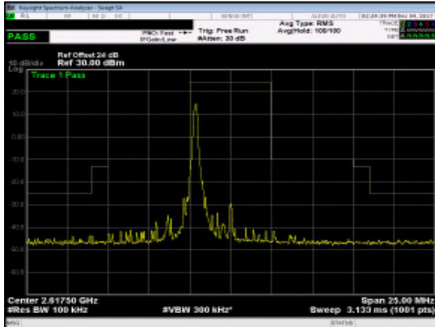
Band 38_5M_QPSK_HIGH_RB1,24
