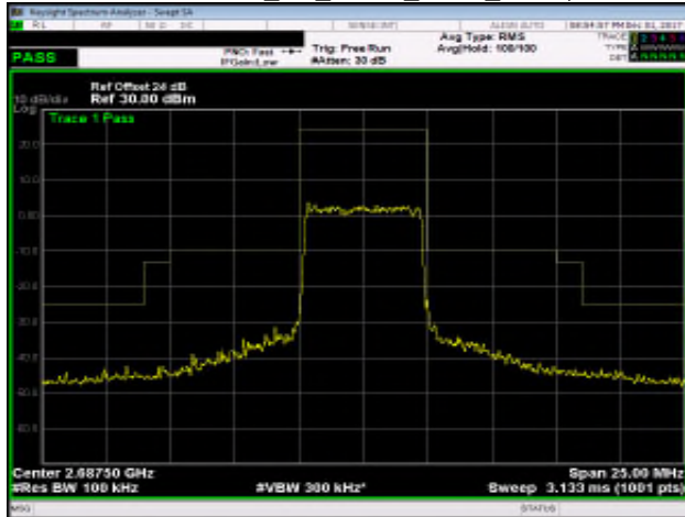
Band 41_5M_QPSK_HIGH_RB25,0
