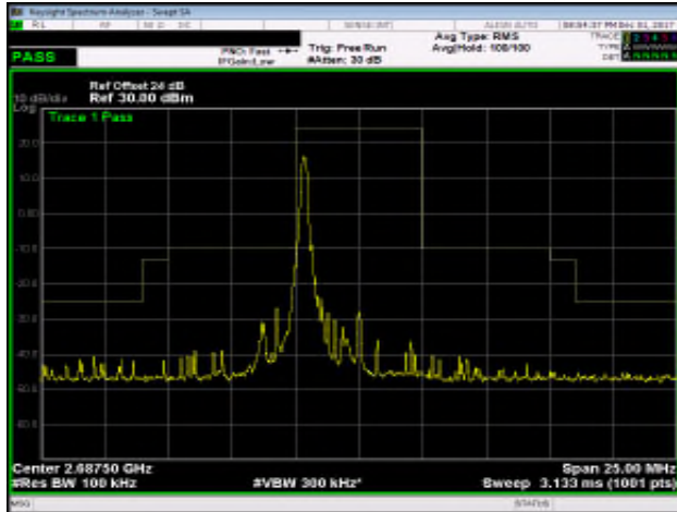
Band 41_5M_QPSK_HIGH_RB1,24
