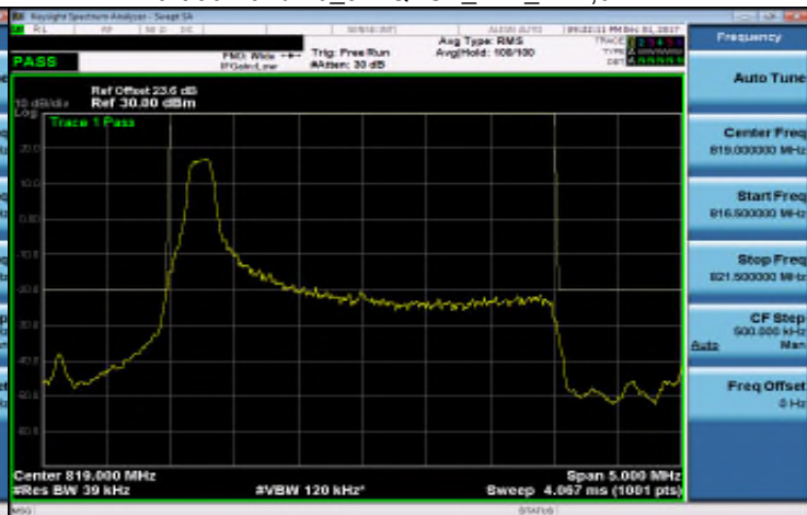
Part 90 Band 26_3M QPSK_MID_RB1,14
