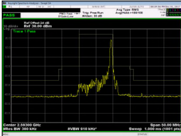
Band 41_10M_16QAM_MID_RB50,0
