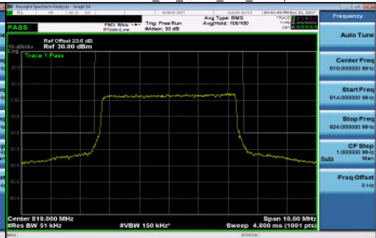
Part 90 Band 26_5M_QPSK_MID_RB25,0
