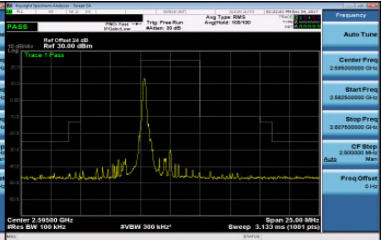
Band 38_5M_QPSK_MID_RB1,24
