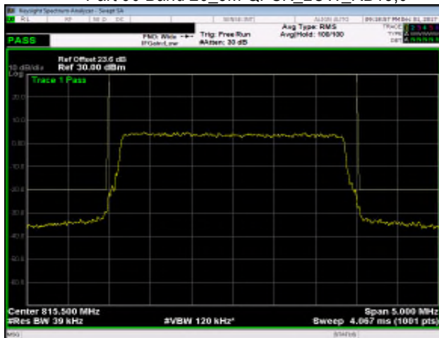
Part 90 Band 26_3M QPSK_LOW_RB15,0
