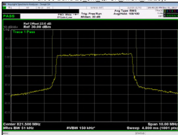
Part 90 Band 26_5M_QPSK_HIGH_RB25,0
