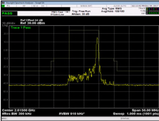
Band 38_10M_QPSK_HIGH_RB50,0
