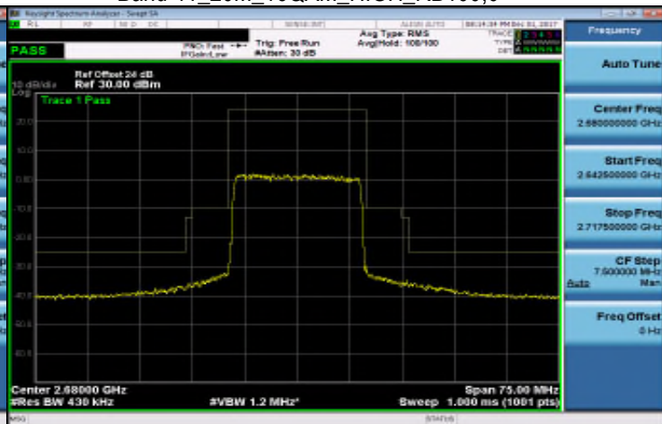
Band 41_20M_16QAM_HIGH_RB100,0
