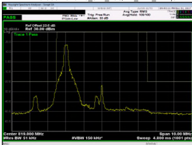
Part 90 Band 26_5M_16QAM_MID_RB1,24
