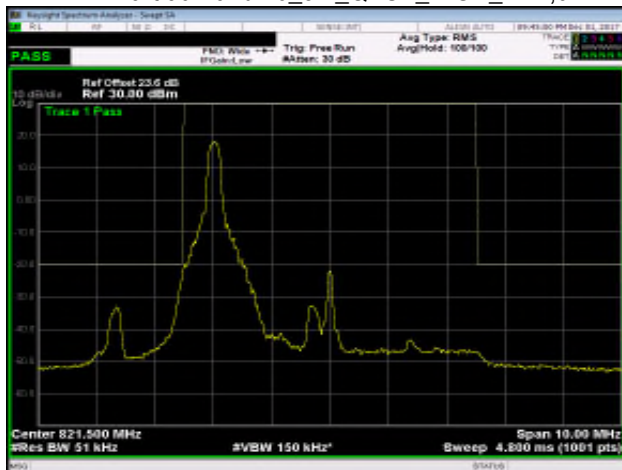
Part 90 Band 26_5M_QPSK_HIGH_RB1,24
