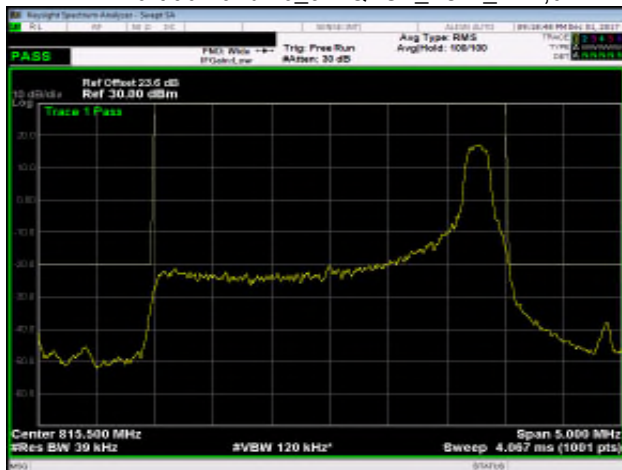
Part 90 Band 26_3M QPSK_LOW_RB1,14
