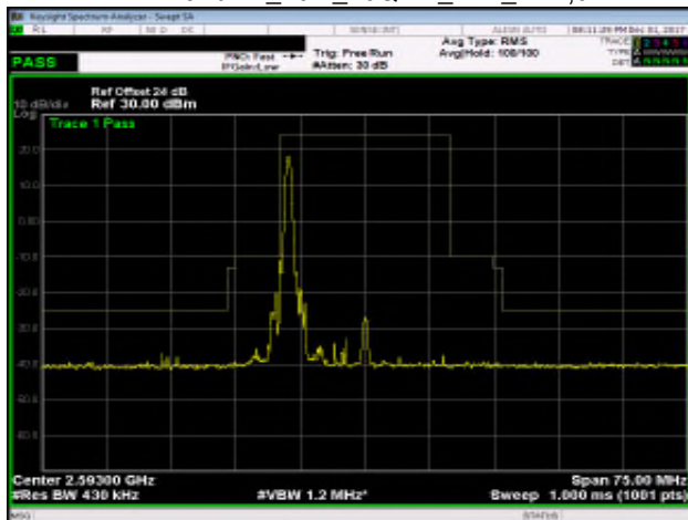
Band 41_20M_16QAM_MID_RB1,99
