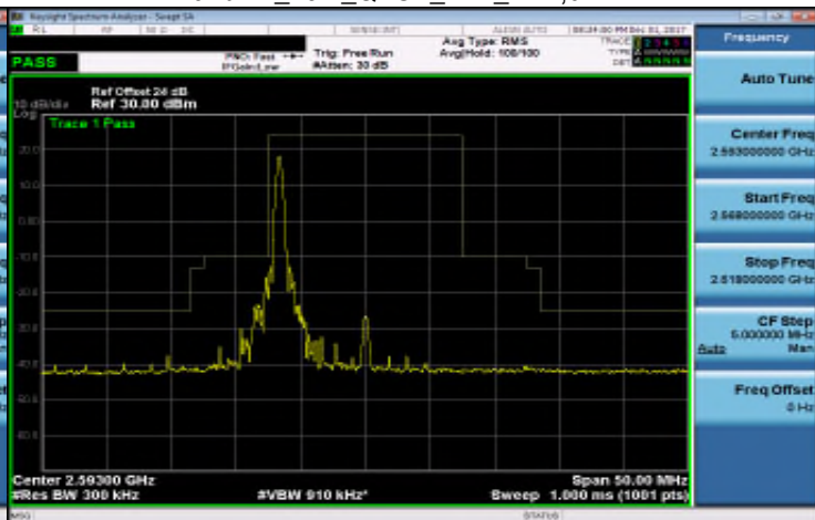
Band 41_15M_QPSK_MID_RB1,74
