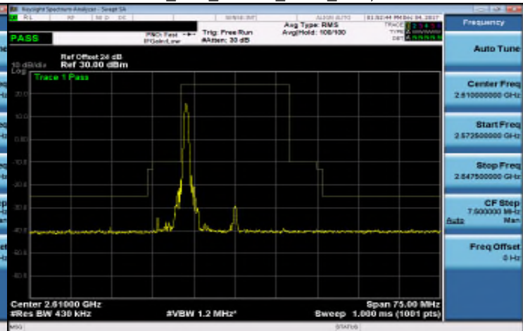
Band 38_20M_16QAM_HIGH_RB1,99
