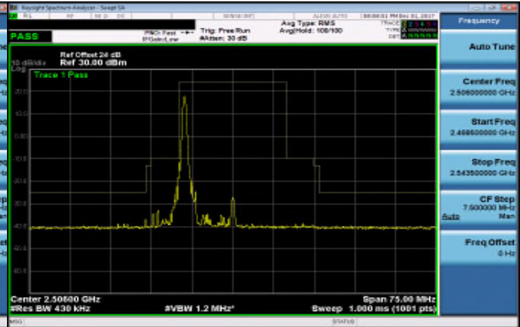
Band 41_20M_16QAM_LOW_RB1,99
