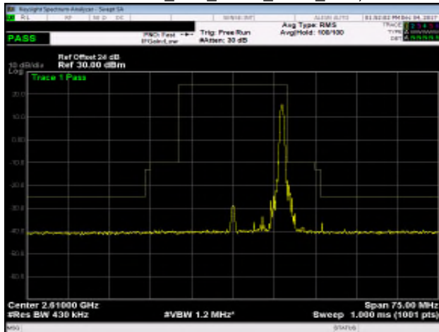
Band 38_20M_QPSK_HIGH_RB100,0
