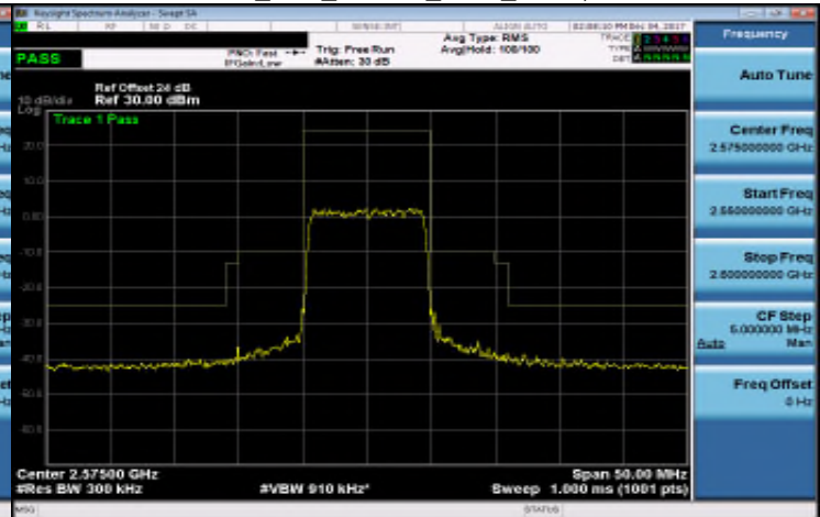
Band 38_10M_16QAM_LOW_RB50,0
