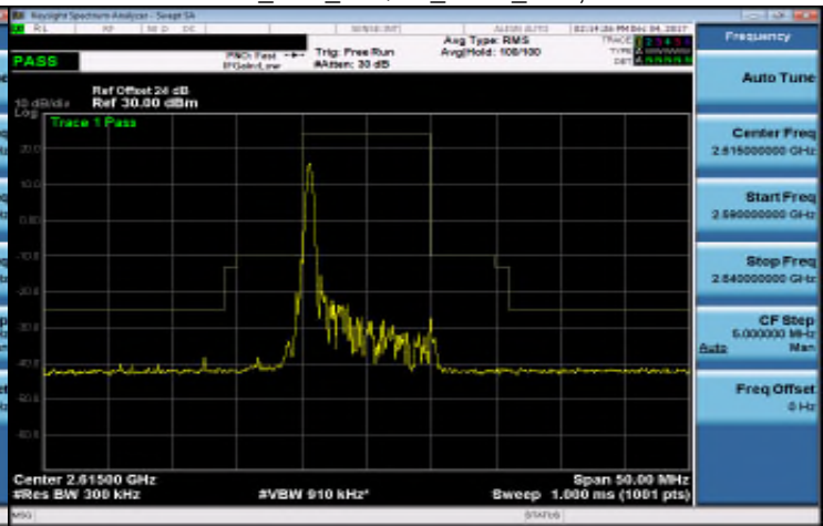
Band 38_10M_16QAM_HIGH_RB1,9
