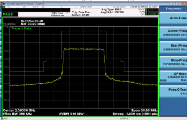
Band 41_15M_QPSK_MID_RB75,0
