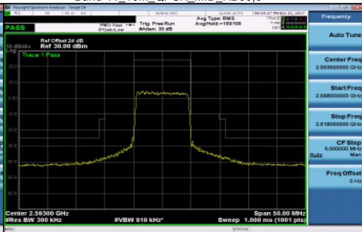
Band 41_10M_QPSK_MID_RB50,0
