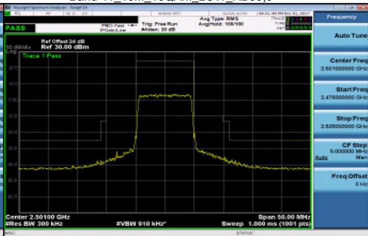
Band 41_10M_16QAM_LOW_RB50,0
