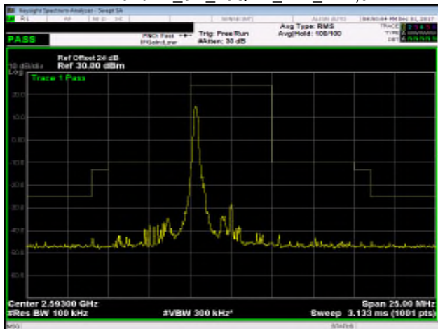
Band 41_5M_16QAM_MID_RB1,24
