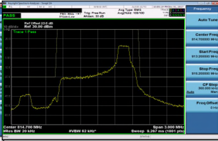
Part 90 Band 26_1.4M_16QAM_LOW_RB25,0
