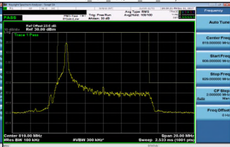
Part 90 Band 26_10M_16QAM_MID_RB1,49
