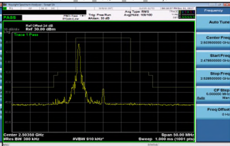
Band 41_15M_16QAM_LOW_RB1,74
