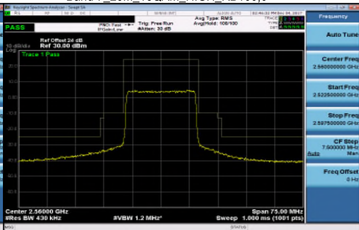
Band 7_20M_16QAM_HIGH_RB100,0
