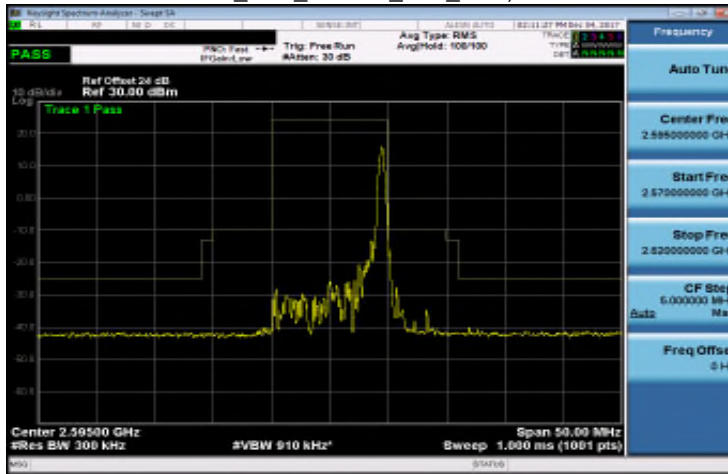
Band 38_10M_16QAM_MID_RB50,0
