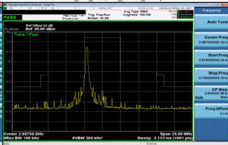
Band 41_5M_16QAM_HIGH_RB1,24
