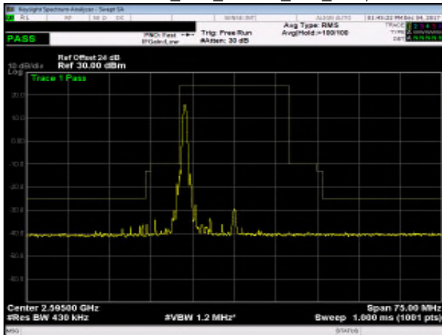
Band 38_20M_16QAM_MID_RB1,99
