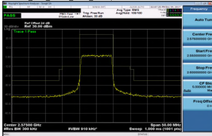
Band 38_10M_QPSK_LOW_RB50,0
