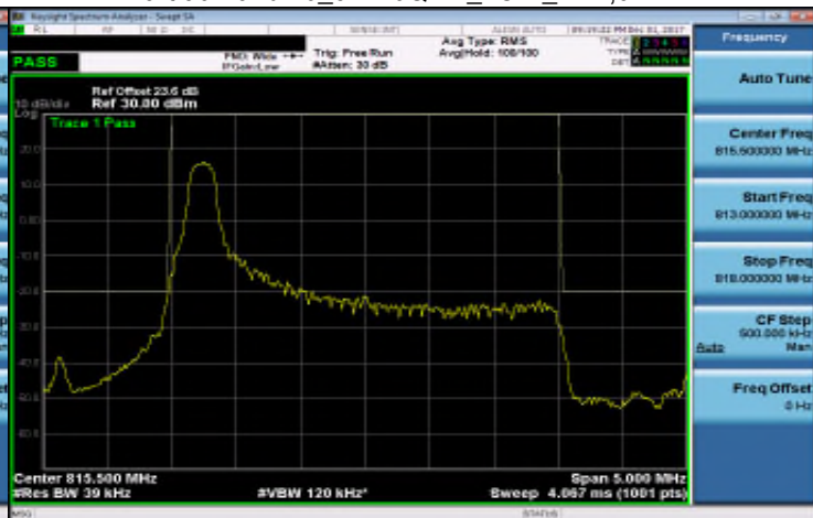
Part 90 Band 26_3M_16QAM_LOW_RB1,14
