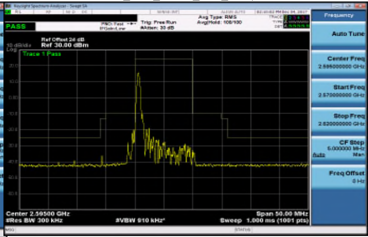
Band 38_10M_QPSK_MID_RB1,49
