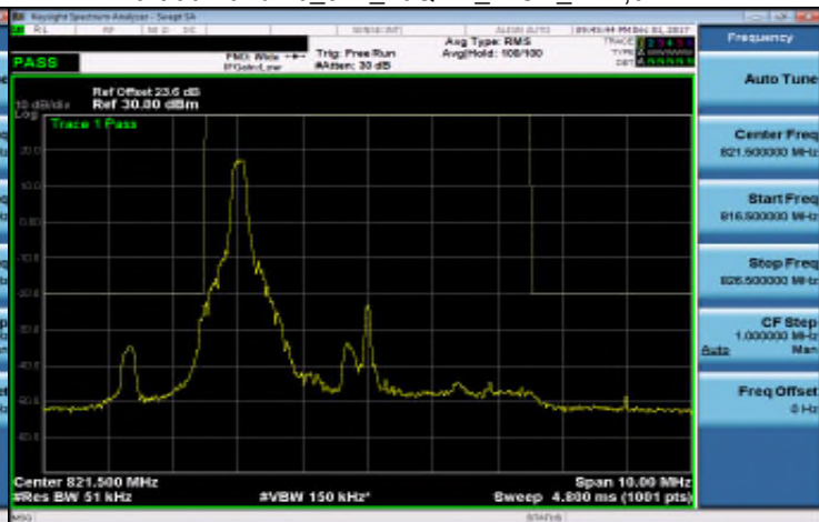
Part 90 Band 26_5M_16QAM_HIGH_RB1,24
