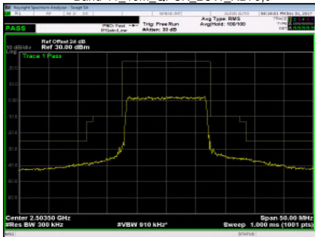
Band 41_15M_QPSK_LOW_RB75,0
