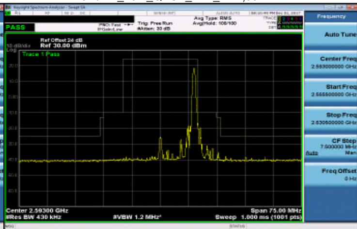
Band 41_20M_QPSK_MID_RB100,0
