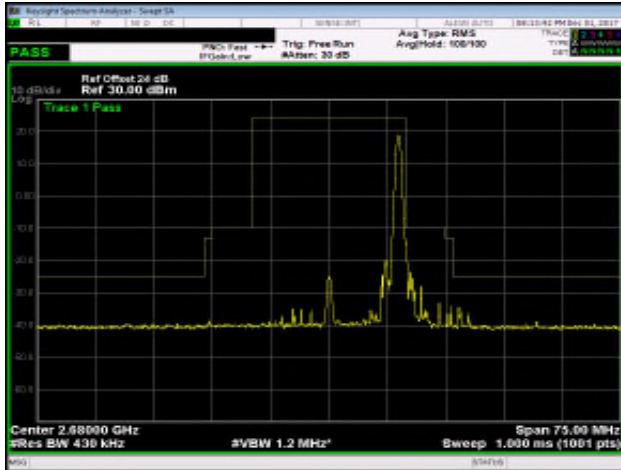
Band 41_20M_QPSK_HIGH_RB100,0
