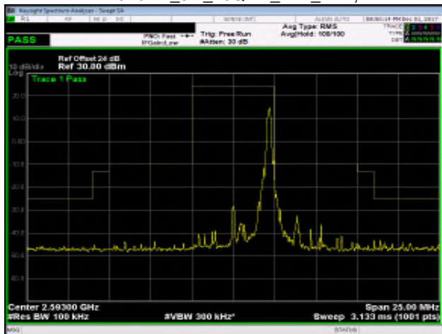
Band 41_5M_16QAM_MID_RB25,0
