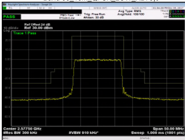
Band 38_15M_QPSK_LOW_RB75,0
