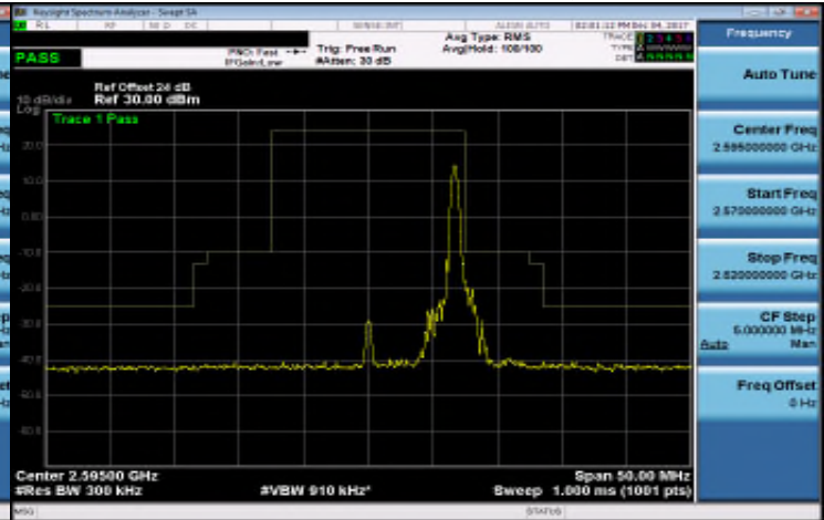
Band 38_15M_16QAM_LOW_RB75,0
