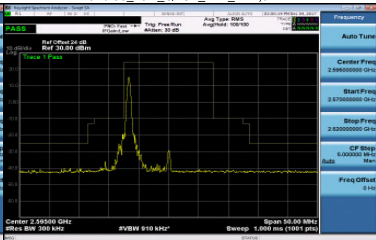
Band 38_15M_QPSK_MID_RB1,74
