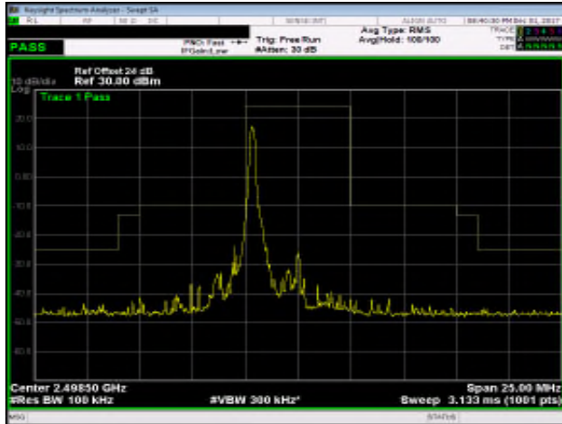
Band 41_5M_QPSK_LOW_RB1,24
