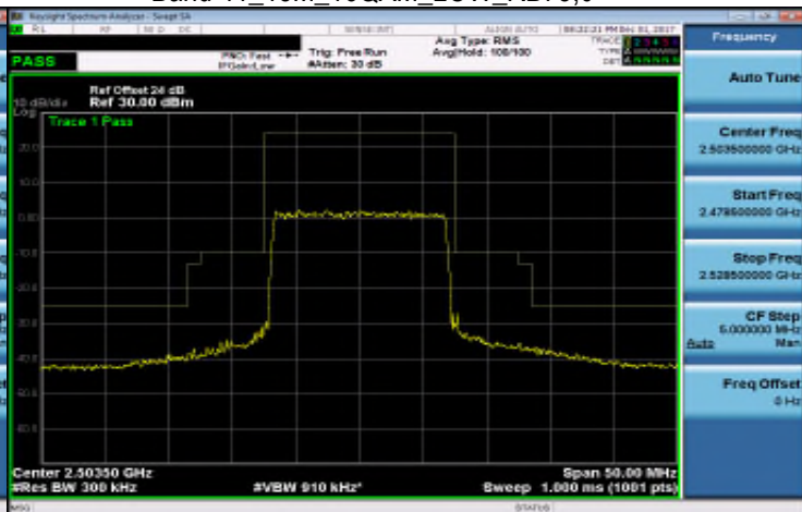
Band 41_15M_16QAM_LOW_RB75,0
