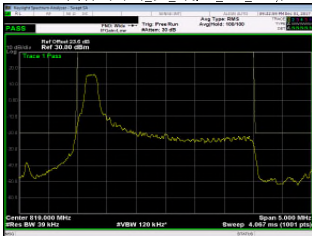
Part 90 Band 26_3M_16QAM_MID_RB1,14
