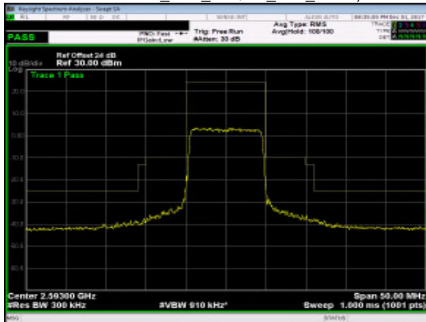
Band 41_10M_16QAM_MID_RB50,0
