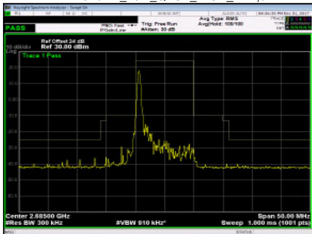
Band 41_10M_QPSK_HIGH_RB1,49
