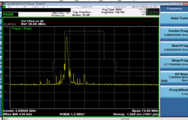
Band 41_20M_16QAM_HIGH_RB1,99
