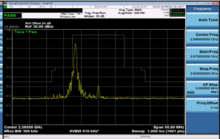
Band 38_15M_16QAM_LOW_RB1,74
