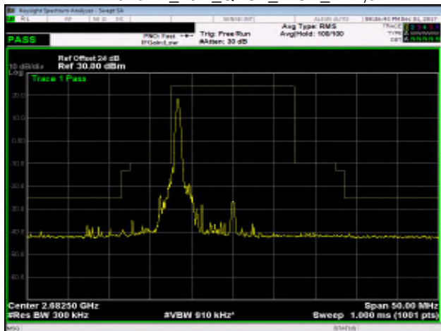
Band 41_15M_QPSK_HIGH_RB1,74
