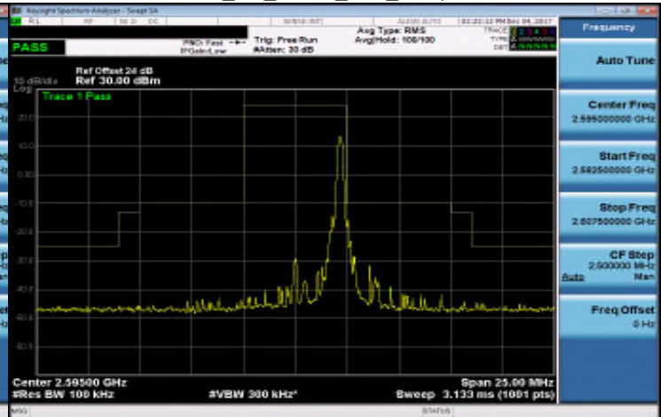
Band 38_5M_QPSK_MID_RB25,0
