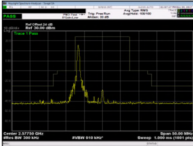
Band 38_15M_QPSK_HIGH_RB1,74
