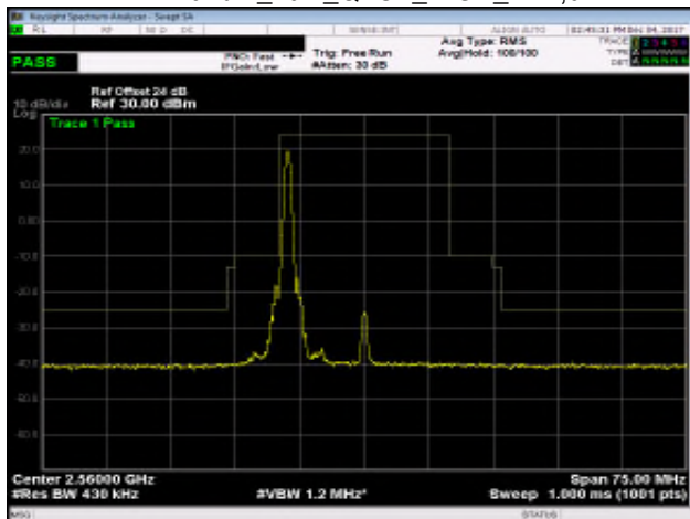
Band 7_20M_QPSK_HIGH_RB1,99
