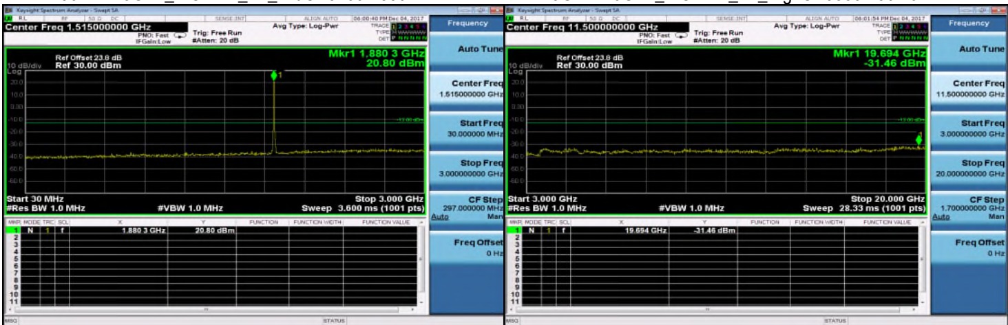
30MHz~3GHz_WCDMA_B2_MidCH9400-1880
