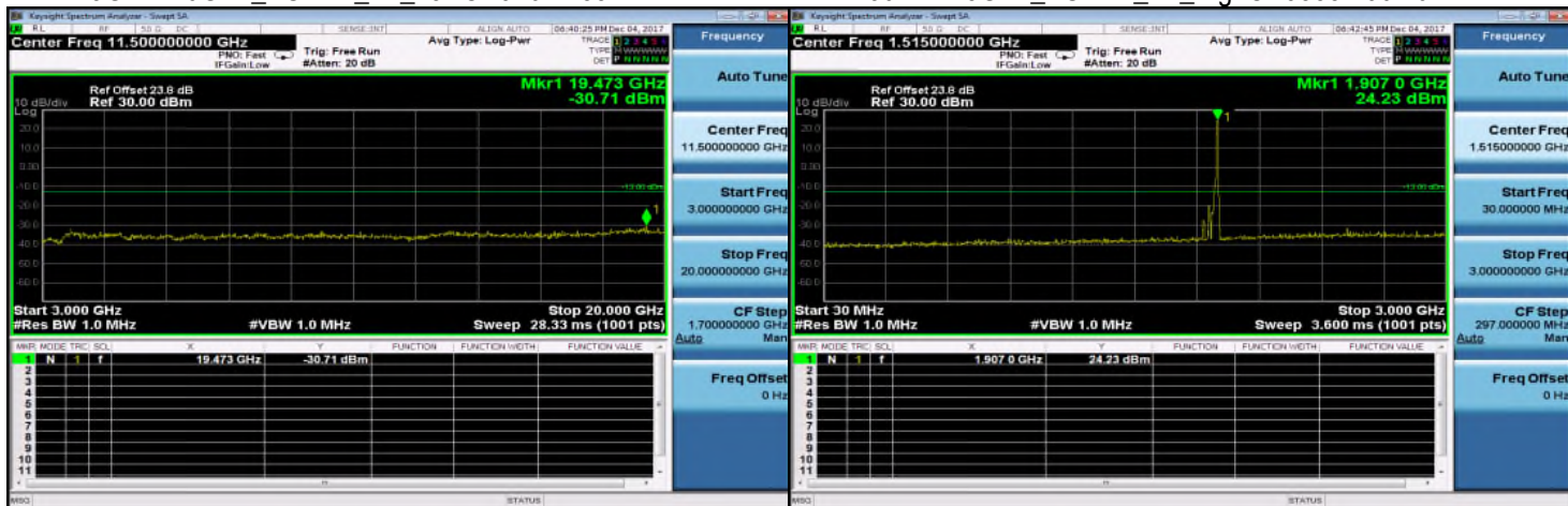
3GHz~20GHz_HSDPA_B2_LowCH9262-1852.4
