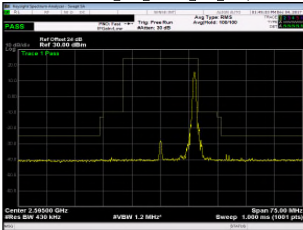
Band 38_20M_16QAM_MID_RB100,0
