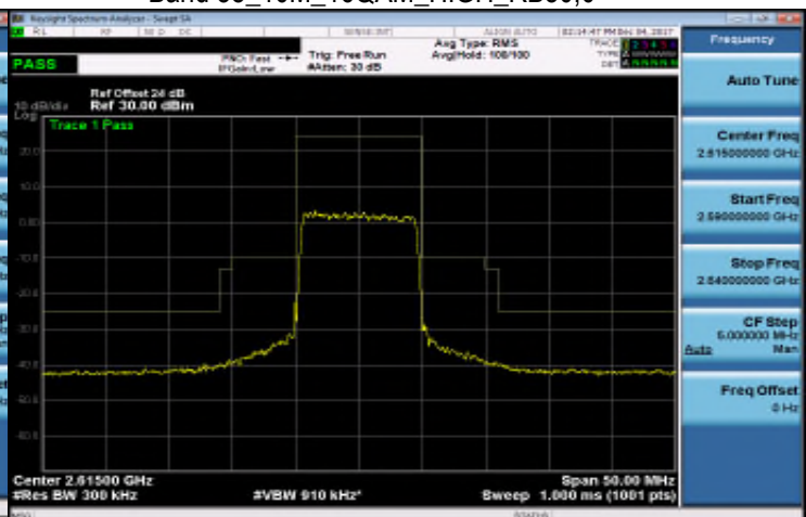
Band 38_10M_16QAM_HIGH_RB50,0
