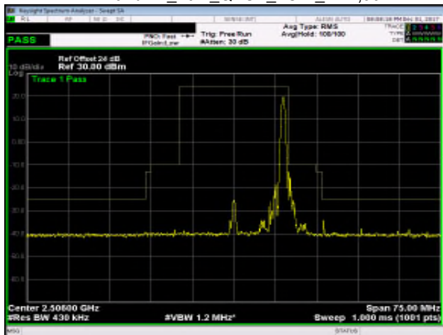
Band 41_20M_QPSK_LOW_RB100,0
