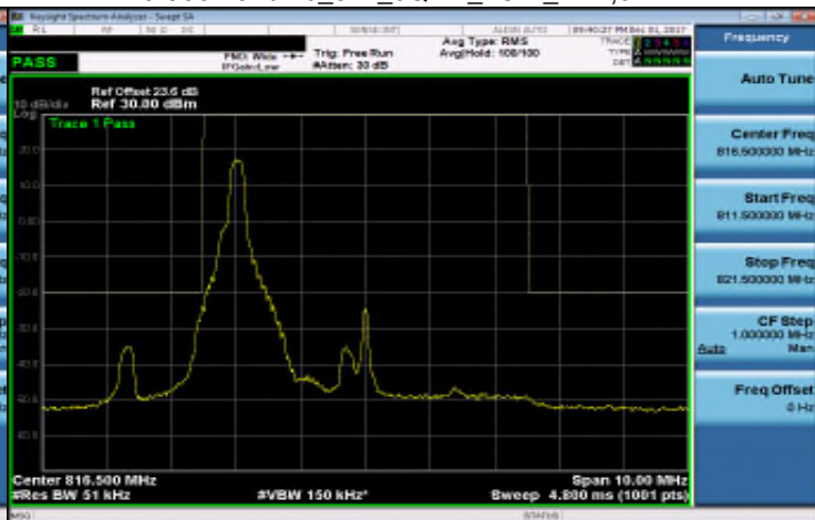
Part 90 Band 26_5M_16QAM_LOW_RB1,24
