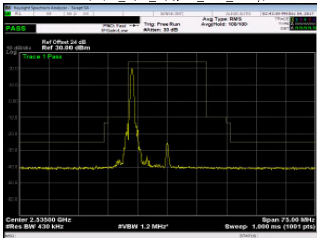
Band 7_20M_16QAM_MID_RB1,99
