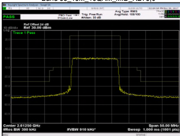
Band 38_15M_16QAM_MID_RB75,0
