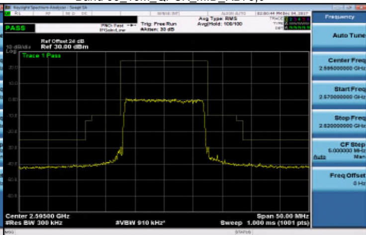
Band 38_15M_QPSK_MID_RB75,0
