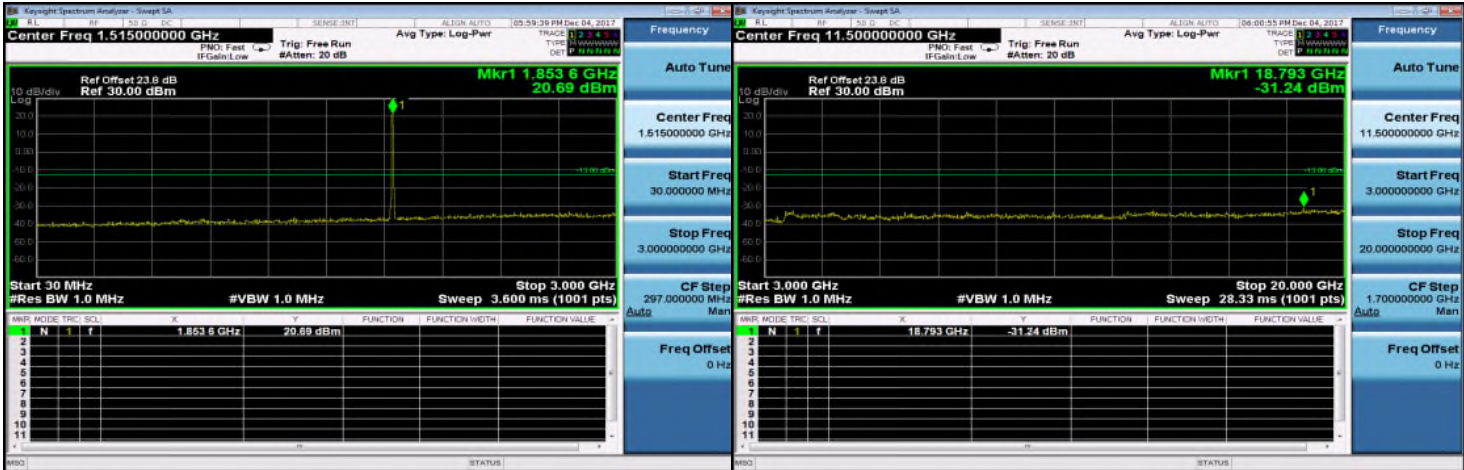
30MHz~3GHz_WCDMA_B2_LowCH9262-1852.4
