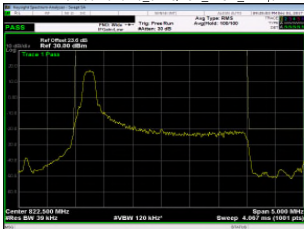
Part 90 Band 26_3M QPSK_HIGH_RB1,14
