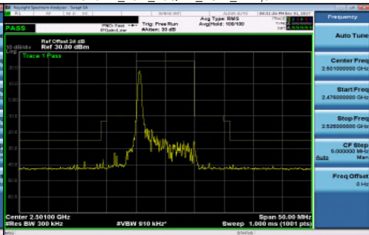
Band 41_10M_16QAM_LOW_RB1,49
