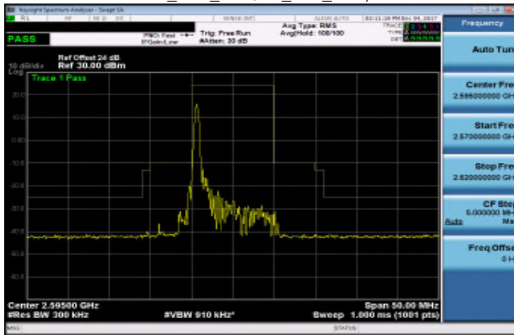
Band 38_10M_16QAM_MID_RB1,9
