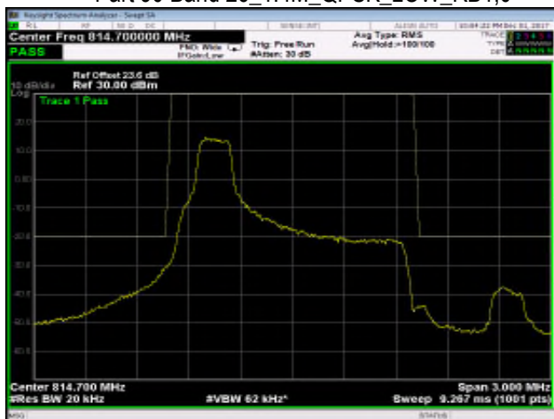
Part 90 Band 26_1.4M_QPSK_LOW_RB1,5
