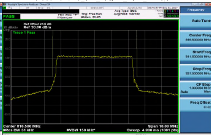
Part 90 Band 26_5M_16QAM_LOW_RB25,0
