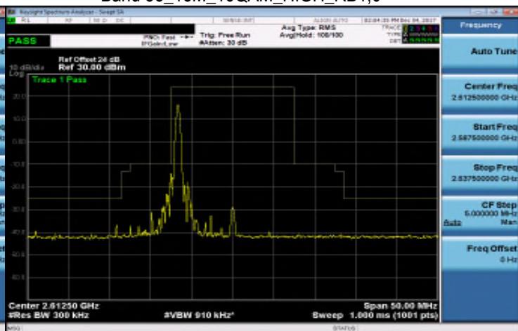
Band 38_15M_16QAM_HIGH_RB1,74
