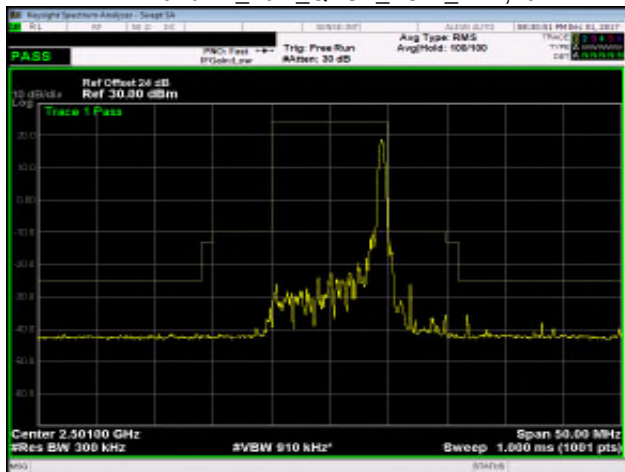
Band 41_10M_QPSK_LOW_RB50,0
