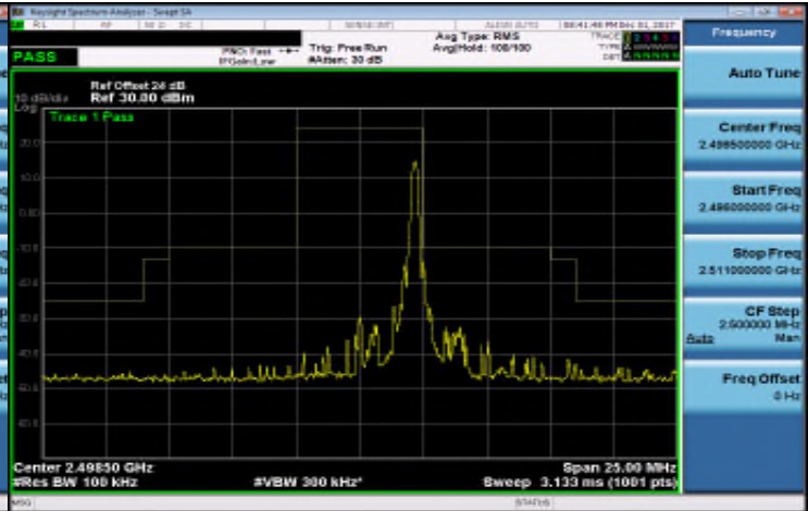
Band 41_5M_16QAM_LOW_RB25,0
