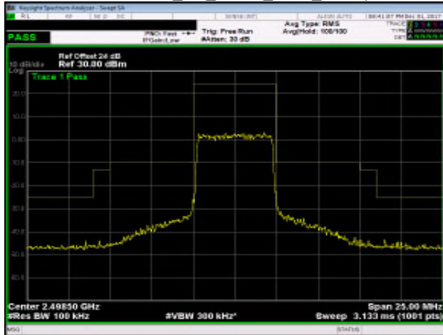
Band 41_5M_QPSK_LOW_RB25,0
