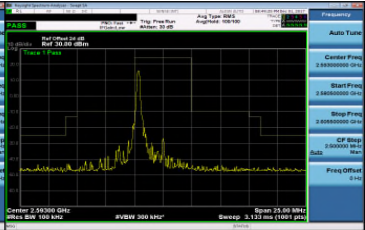
Band 41_5M_QPSK_MID_RB1,24
