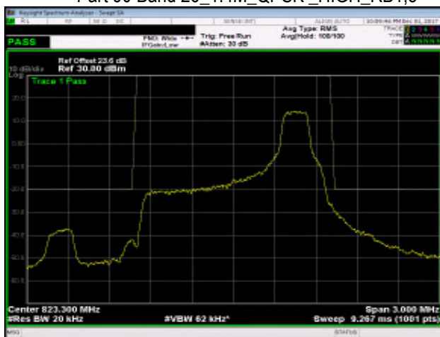
Part 90 Band 26_1.4M_QPSK_HIGH_RB6,0
