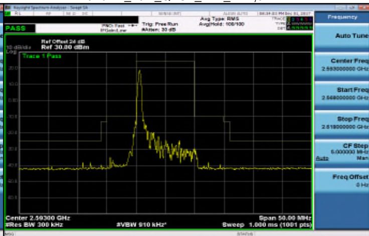
Band 41_10M_QPSK_MID_RB1,49
