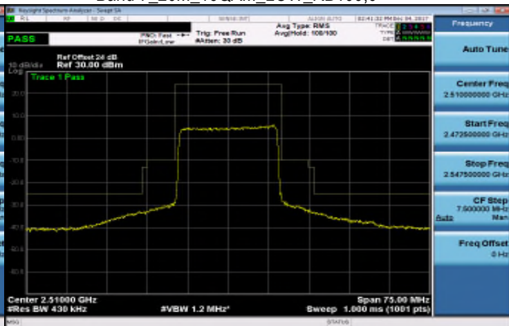
Band 7_20M_16QAM_LOW_RB100,0
