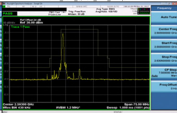
Band 41_20M_QPSK_MID_RB1,99
