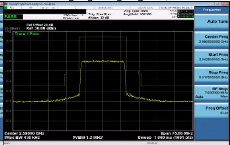
Band 38_20M_16QAM_LOW_RB100,0
