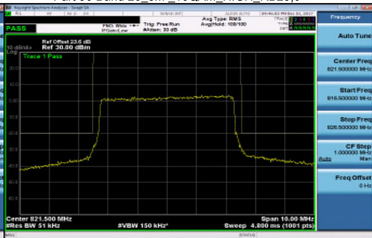
Part 90 Band 26_5M_16QAM_HIGH_RB25,0
