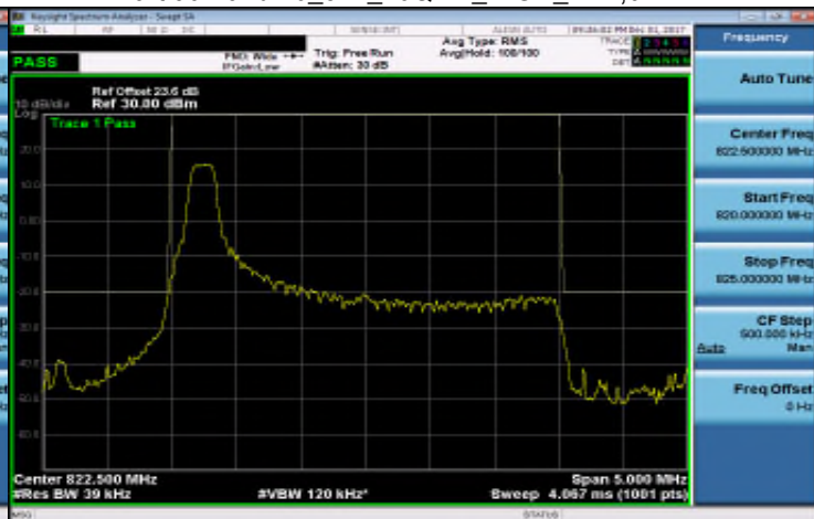
Part 90 Band 26_3M_16QAM_HIGH_RB1,14
