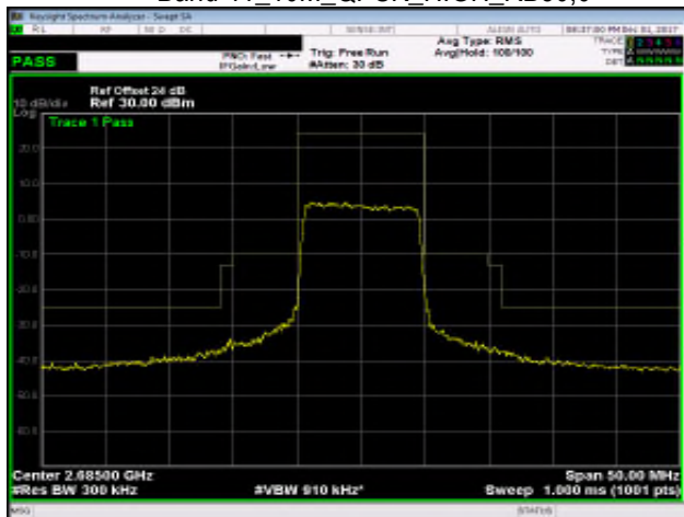
Band 41_10M_QPSK_HIGH_RB50,0
