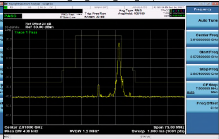
Band 38_20M_16QAM_HIGH_RB100,0
