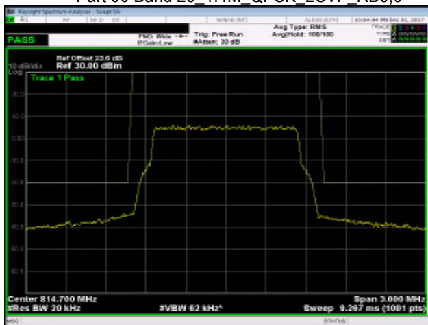
Part 90 Band 26_1.4M_QPSK_LOW_RB6,0
