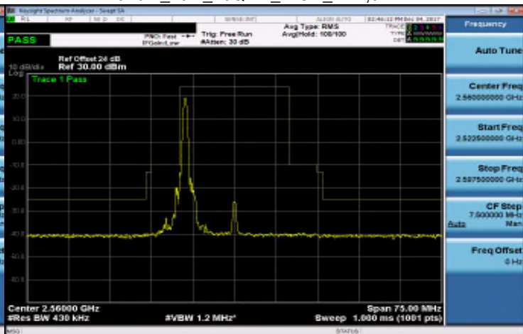
Band 7_20M_16QAM_HIGH_RB1,99
