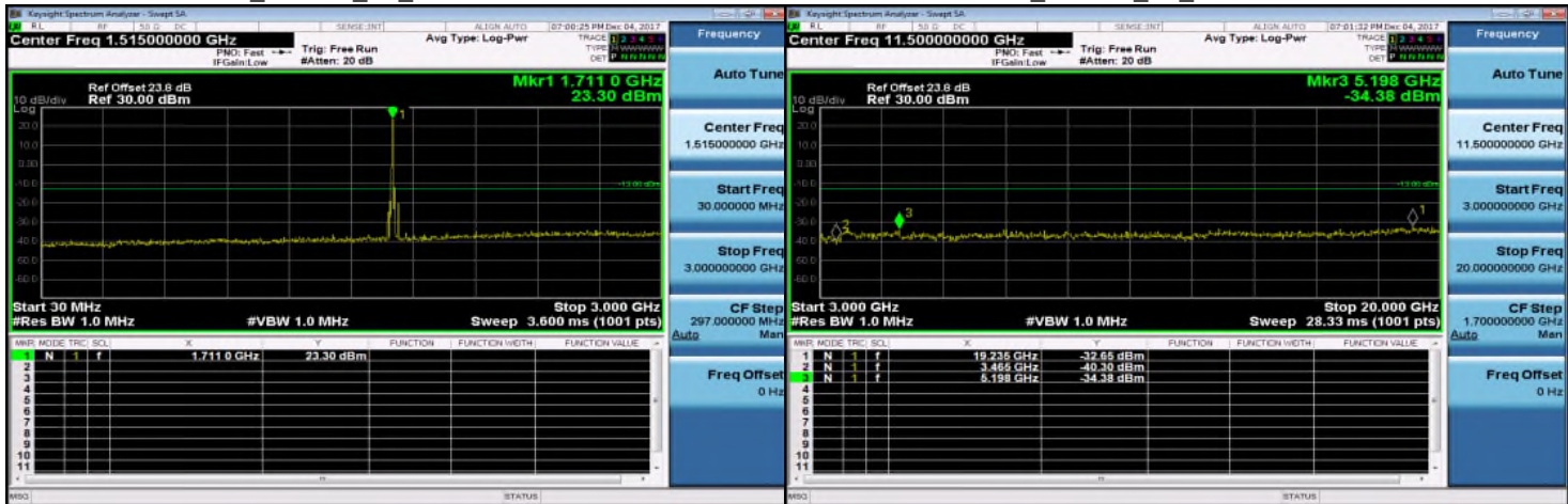
30MHz~3GHz_HSUPA_B4_LowCH1312-1712.4
