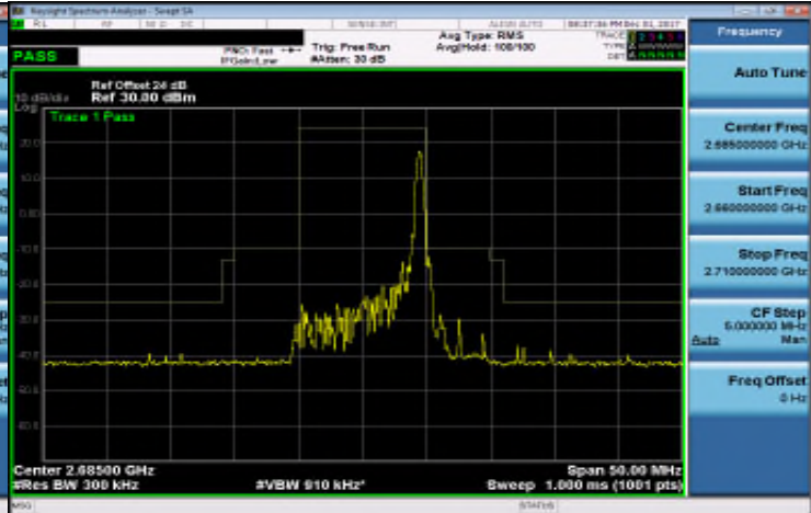
Band 41_10M_16QAM_HIGH_RB50,0
