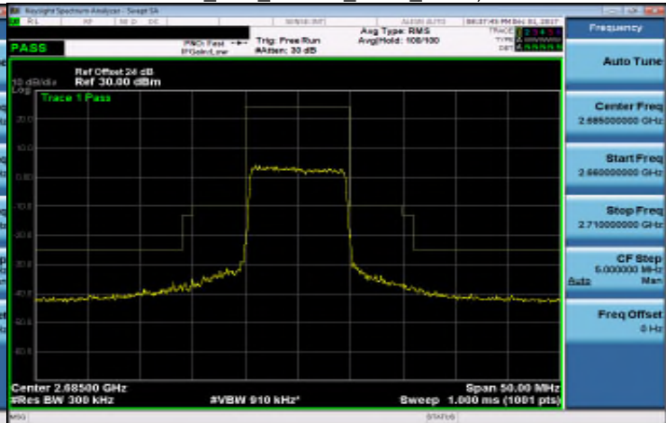
Band 41_10M_16QAM_HIGH_RB50,0
