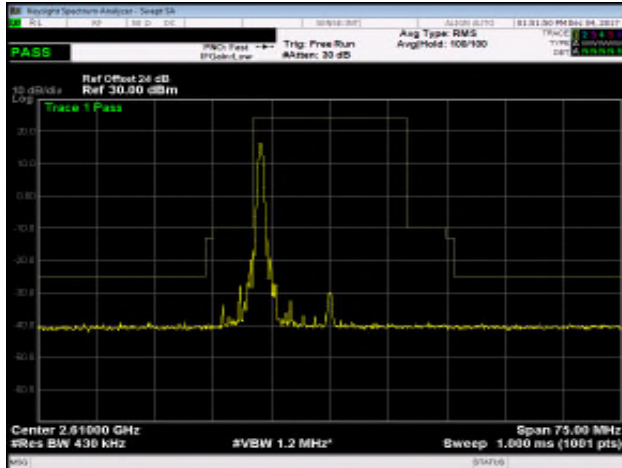
Band 38_20M_QPSK_HIGH_RB1,99
