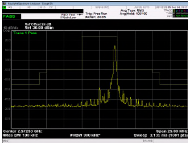
Band 38_5M_QPSK_LOW_RB25,0
