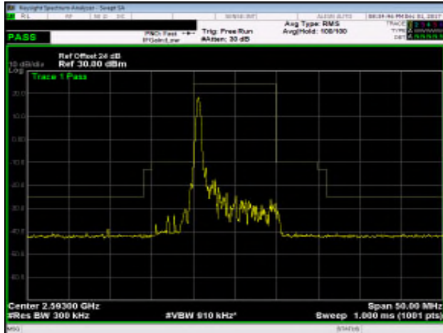
Band 41_10M_16QAM_MID_RB1,49
