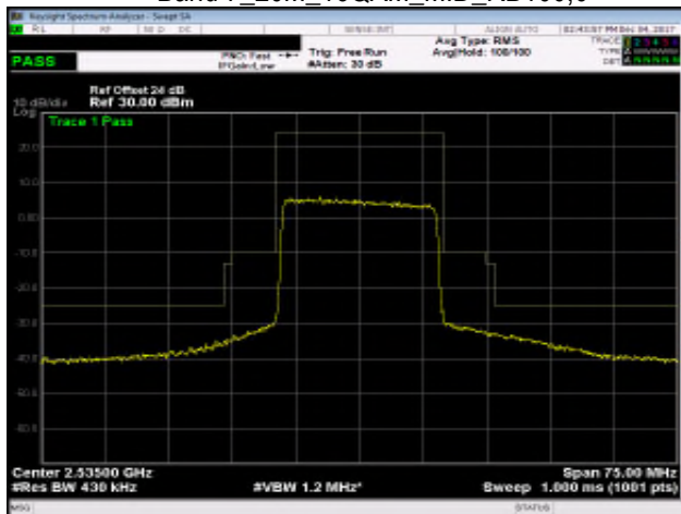
Band 7_20M_16QAM_MID_RB100,0
