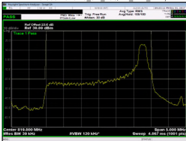
Part 90 Band 26_3M_16QAM_MID_RB15,0
