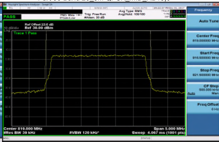
Part 90 Band 26_3M QPSK_MID_RB15,0
