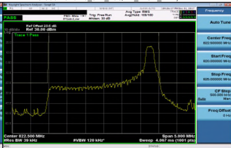
Part 90 Band 26_3M_16QAM_HIGH_RB15,0
