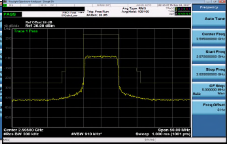
Band 38_10M_QPSK_MID_RB50,0
