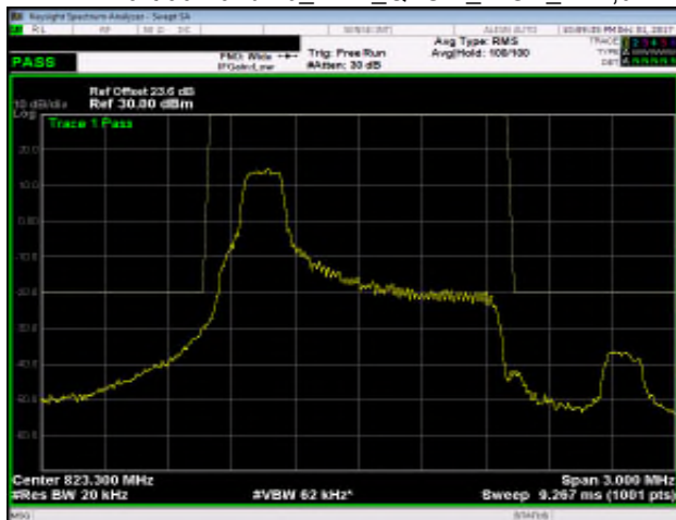
Part 90 Band 26_1.4M_QPSK_HIGH_RB1,5
