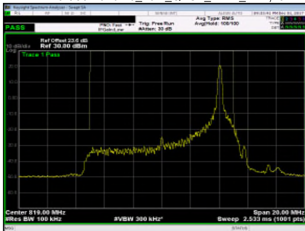
Part 90 Band 26_10M_QPSK_MID_RB50,0
