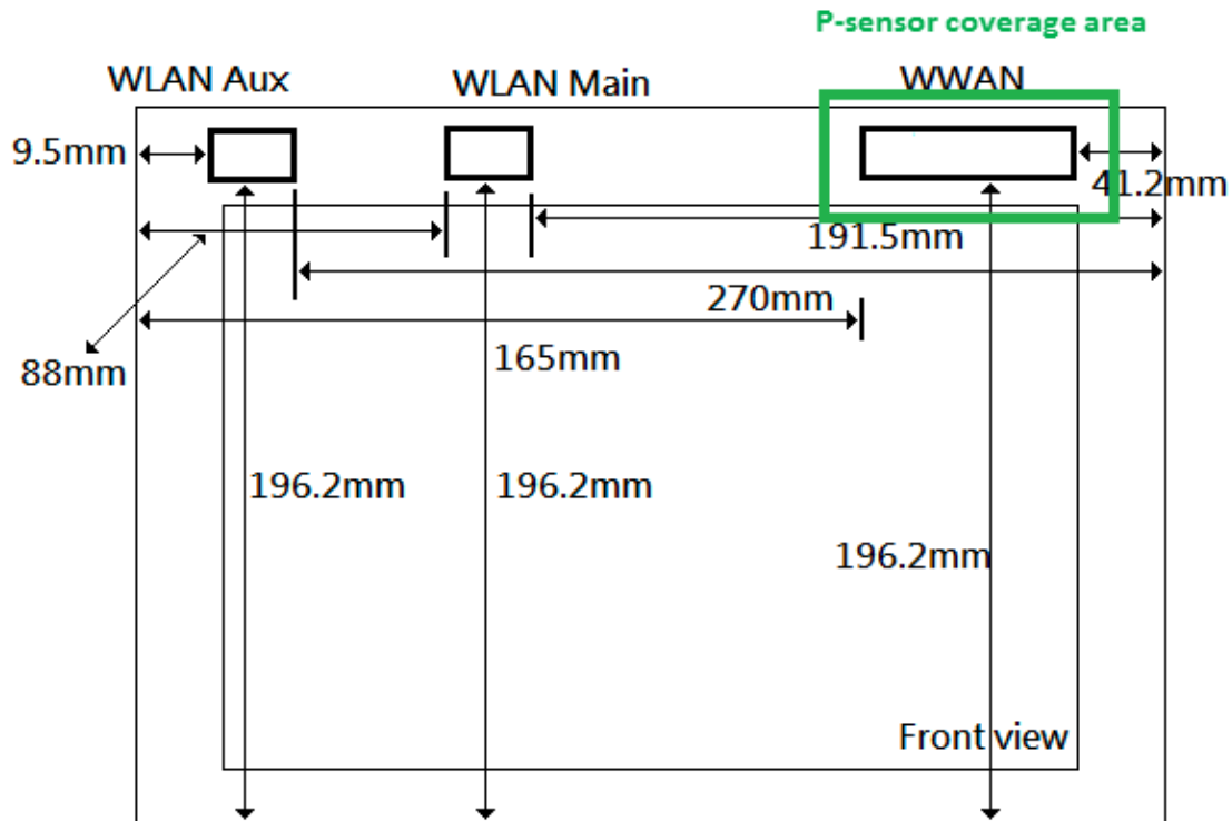
Fig.12 Antenna position of EUT
