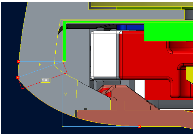
The WWAN Antenna surface edge along the curved
