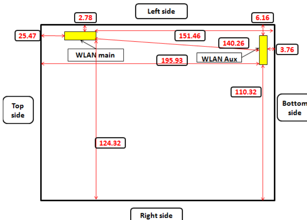
Fig.9 Antenna position of EUT (Back view)
