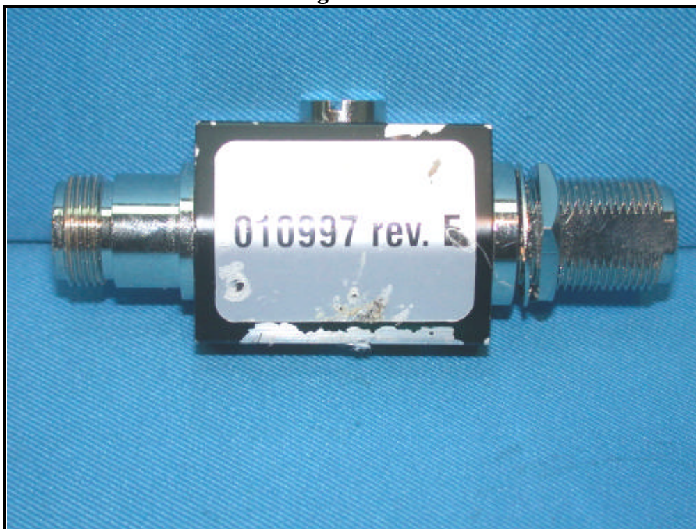
Surge arrestor
