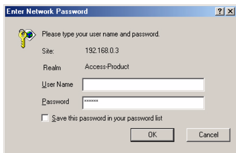
Figure 6. Network Password
