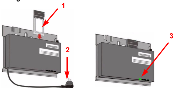
Figure 5. Installing an AP Card
