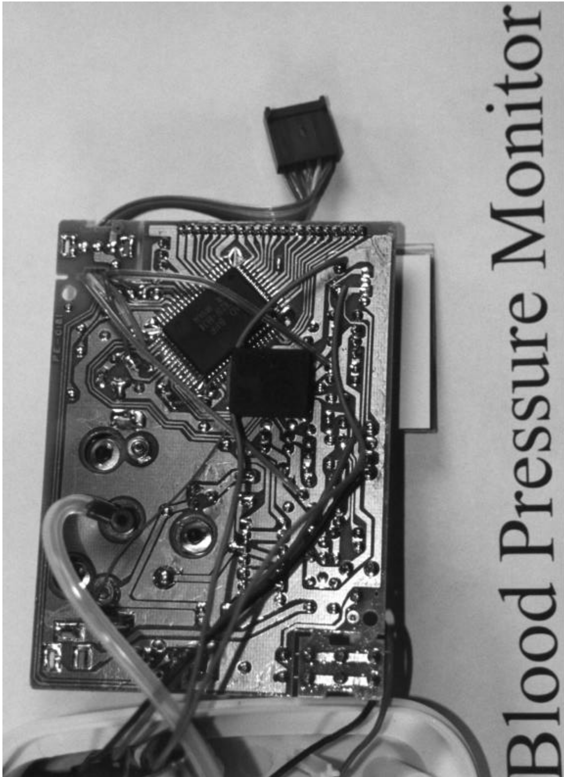
Rear of Board One
