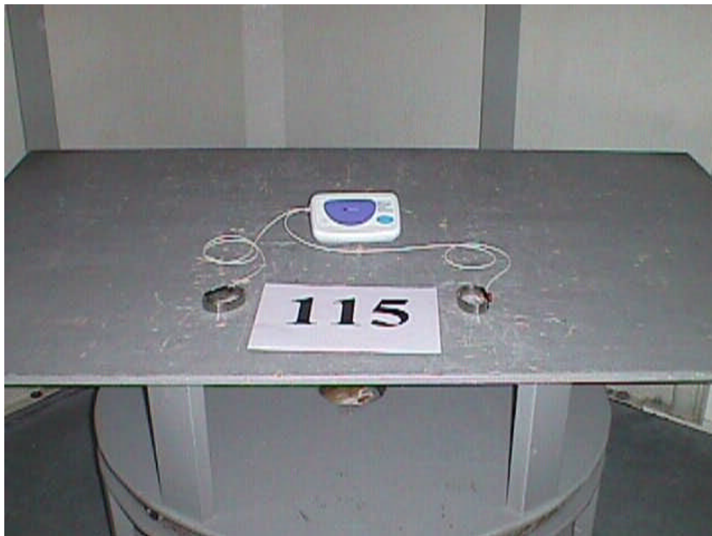
Radiated Emissions
