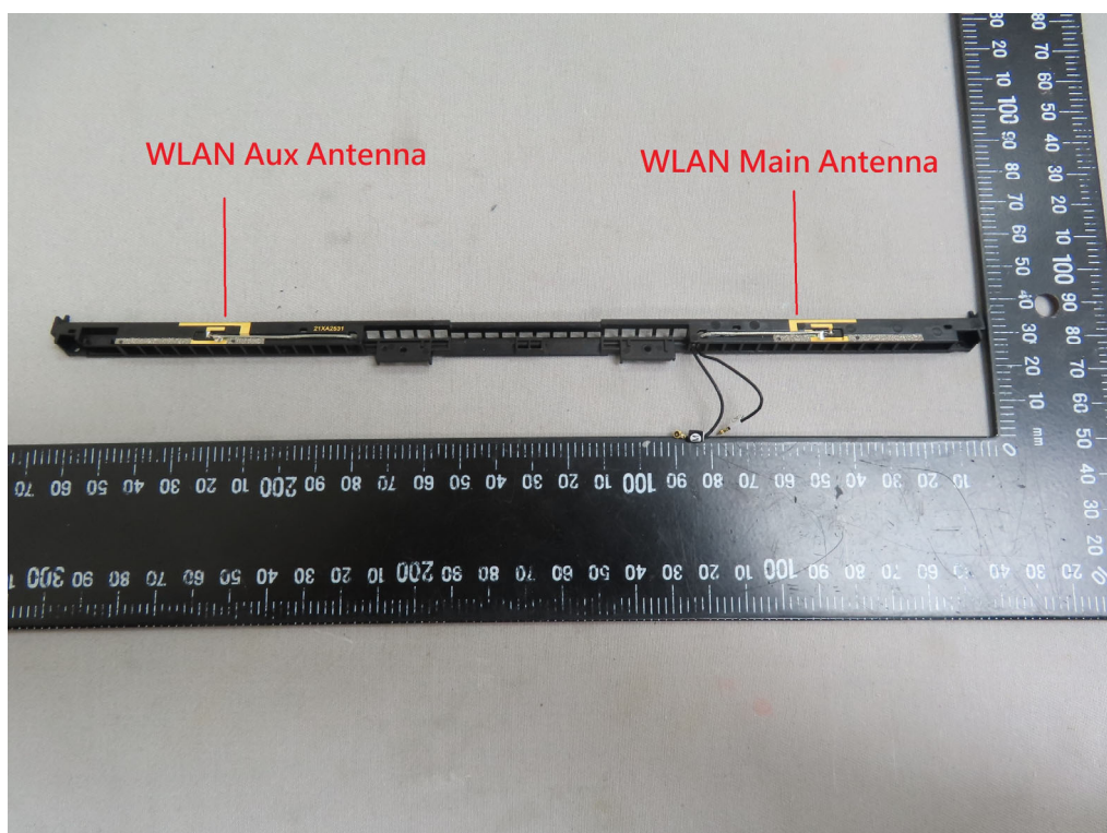
WLAN Antenna
