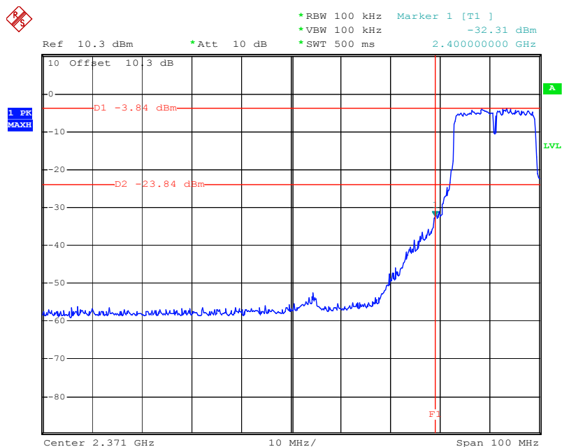
802.11g CH01
