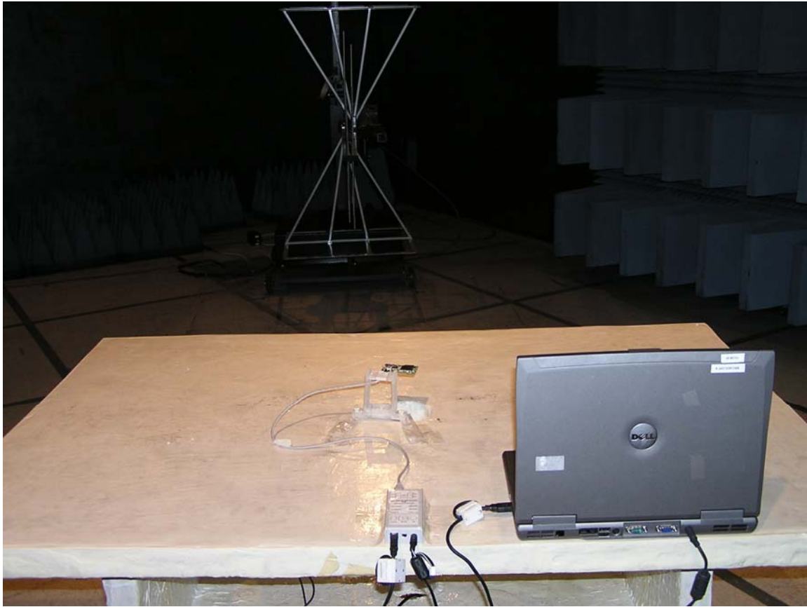
Test setup – Radiated measurements with USB 1.1
