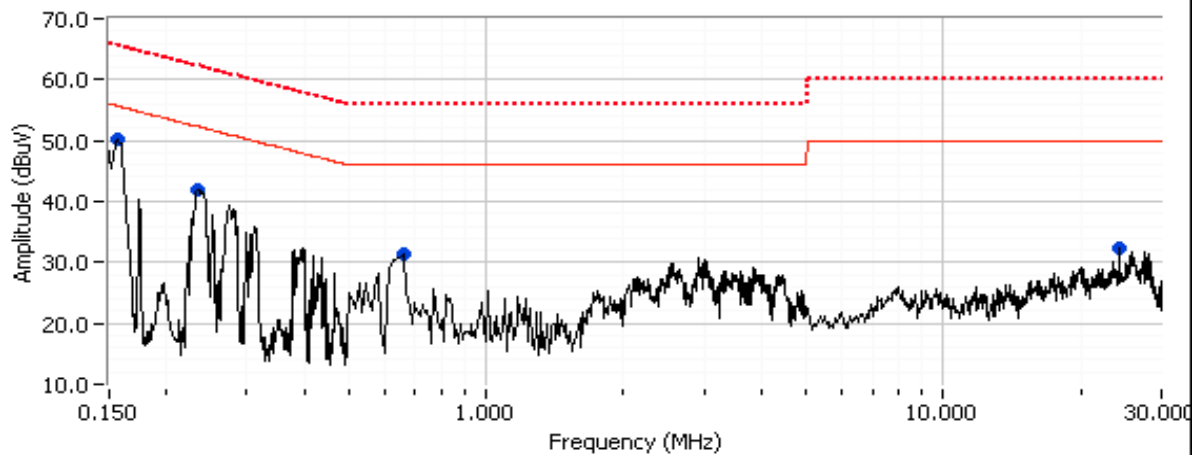
.15 - 30 MHz, 120V/60Hz, BLE CH0, WiFi b mode CH11, Neutral
