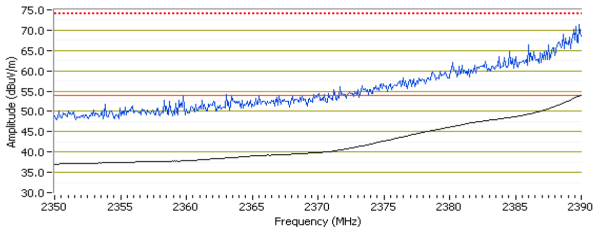
RB 1 MHz; VB 10 Hz Avg (Black trace); RB 1MHz VB 3MHz PK (Blue trace) H
