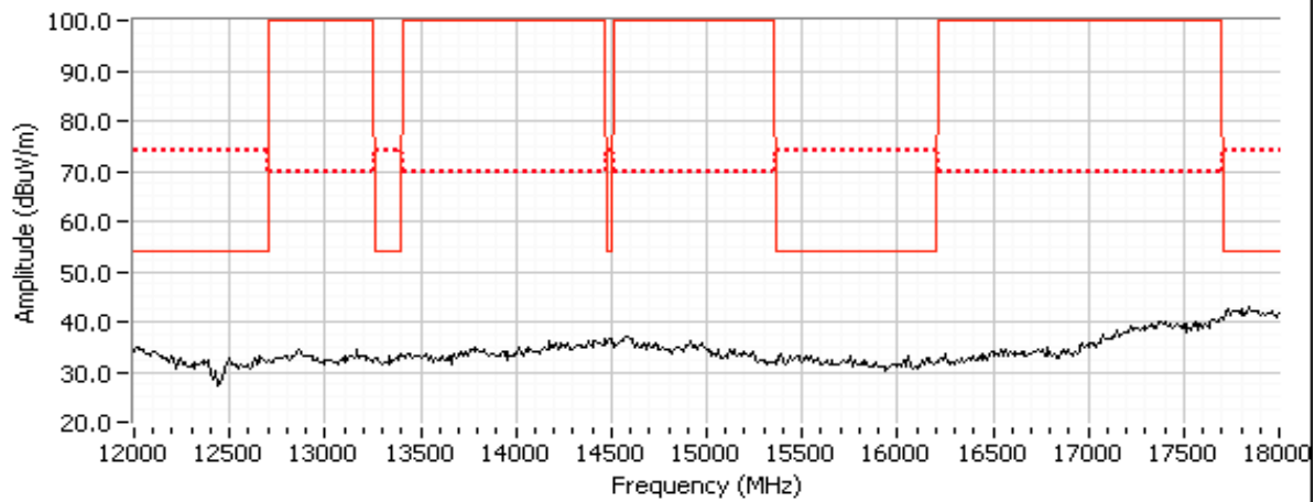
802.11g, Main Antenna, 2437 MHz
