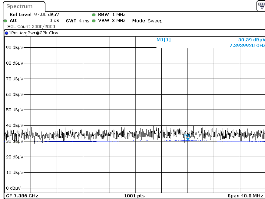
Radiated Spurious Emissions plot – Average Result (802.11b_1 Mbps, Ch.11 3rd Harmonic, Y-H)
