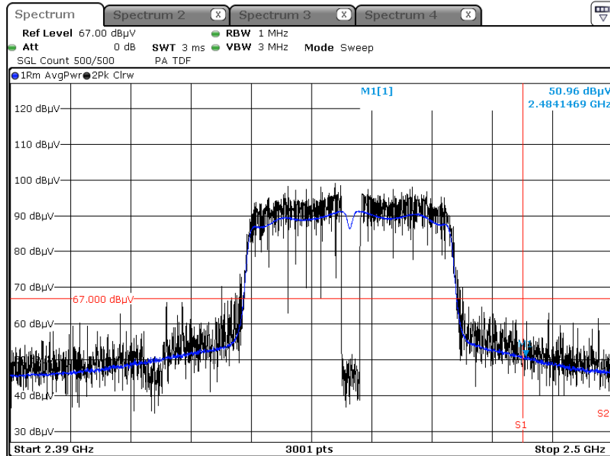
Radiated Restricted Band Edges plot – Average Result (802.11n(HT40)_ MCS0, Ch.9, Z-H)
