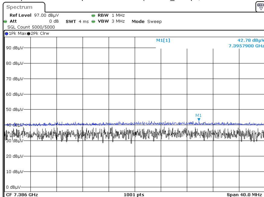
Radiated Spurious Emissions plot – Peak Result (802.11b_1 Mbps, Ch.11 3rd Harmonic, Y-H)
