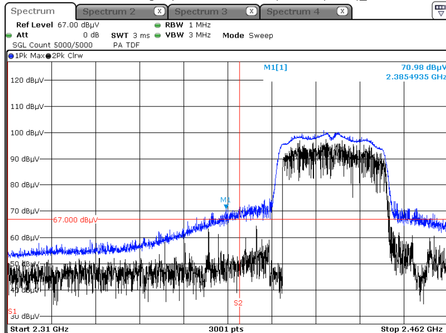
Radiated Restricted Band Edges plot – Peak Result (802.11n(HT40)_MCS0, Ch.3, Z-H)
