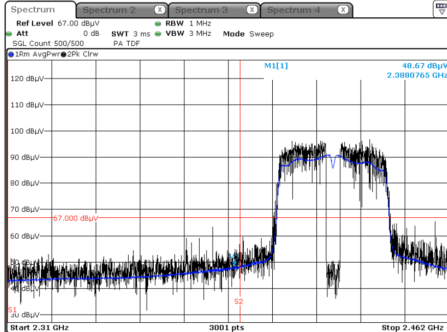
Radiated Restricted Band Edges plot – Average Result (802.11n(HT40)_MCS0, Ch.3, Z-H)
