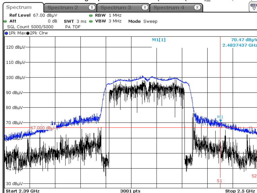
Radiated Restricted Band Edges plot – Peak Result (802.11n(HT40)_ MCS0, Ch.9, Z-H)
