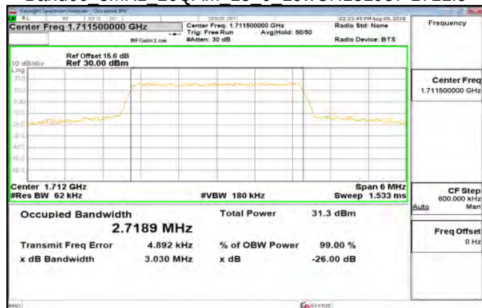
Band66 3MHz 16QAM 15 0 LowCH131987-1711.5
