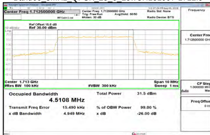
Band66 5MHz QPSK 25 0 LowCH131997-1712.5
