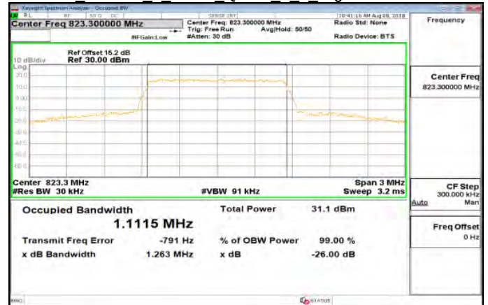
Part 90 Band26 1 4MHz QPSK 6 0 HighCH26783-823.3
