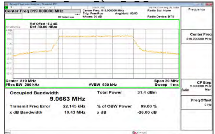
Part 90 Band26 10MHz QPSK 50 0 HighCH26740-819
