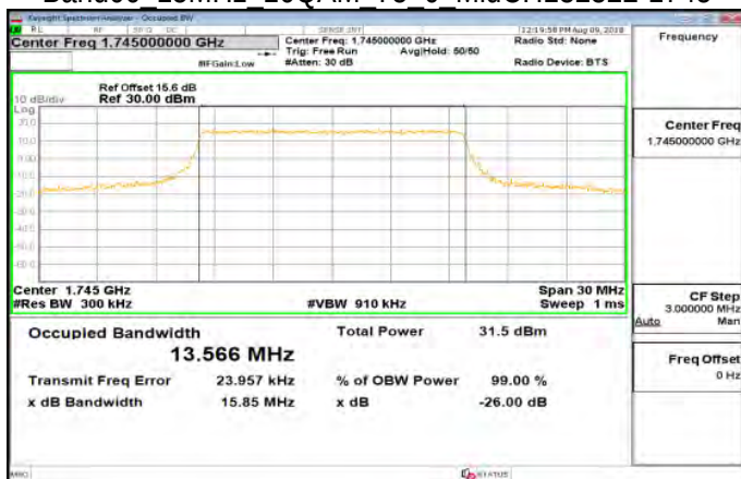
Band66 15MHz 16QAM 75 0 MidCH132322-1745
