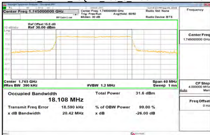
Band66 20MHz 16QAM 100 0 MidCH132322-1745
