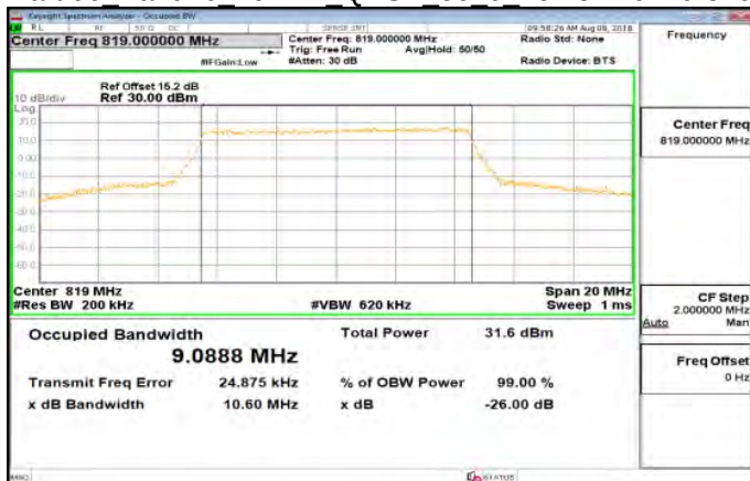
Part 90 Band26 10MHz QPSK 50 0 LowCH26740-819
