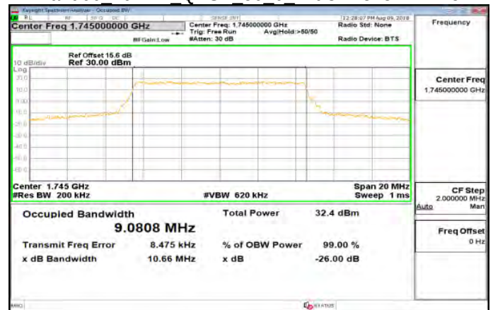
Band66 10MHz QPSK 50 0 MidCH132322-1745
