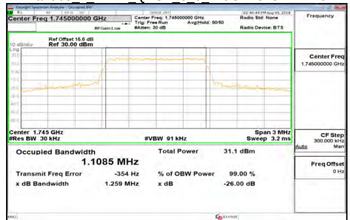
Band66 1 4MHz QPSK 6 0 MidCH132322-1745
