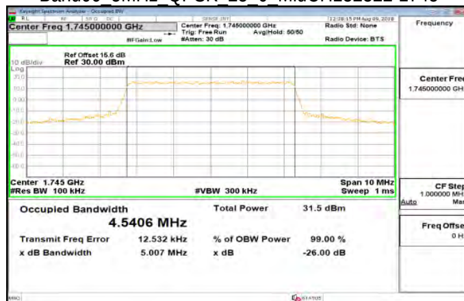
Band66 5MHz QPSK 25 0 MidCH132322-1745
