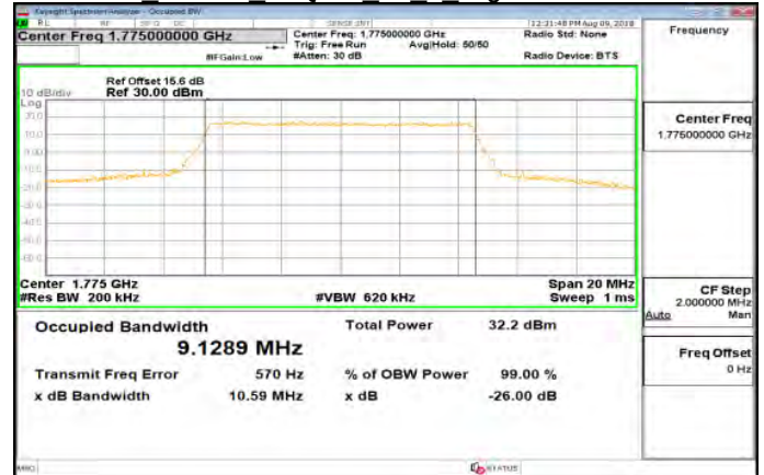
Band66 10MHz 16QAM 50 0 HighCH132622-1775
