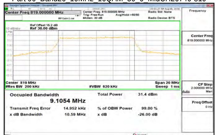
Part 90 Band26 10MHz 16QAM 50 0 MidCH26740-819
