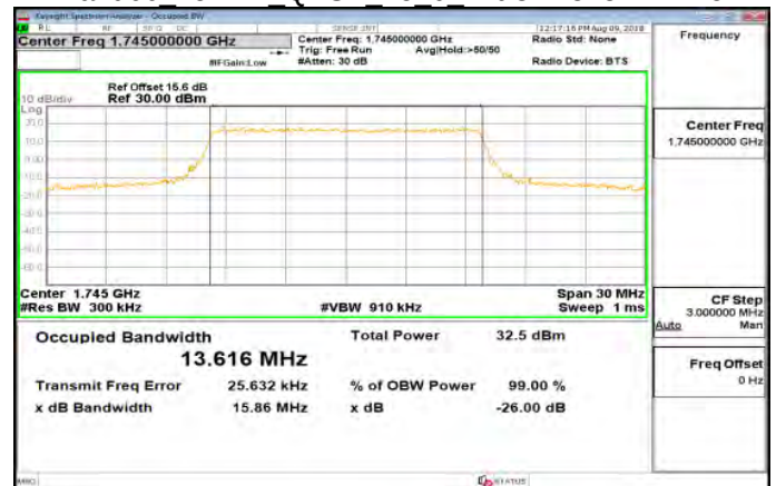
Band66 15MHz QPSK 75 0 MidCH132322-1745
