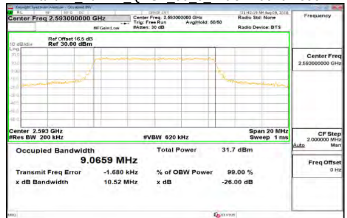
Band41 10MHz QPSK 50 0 MidCH40620-2593
