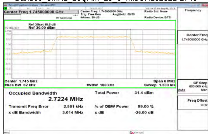
Band66 3MHz 16QAM 15 0 MidCH132322-1745
