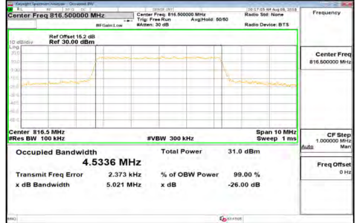
Part 90 Band26 5MHz 16QAM 25 0 LowCH26715-816.5
