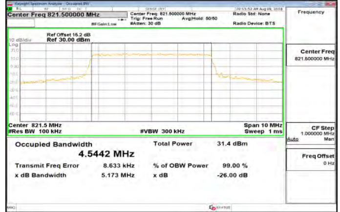
Part 90 Band26 5MHz QPSK 25 0 HighCH26765-821.5
