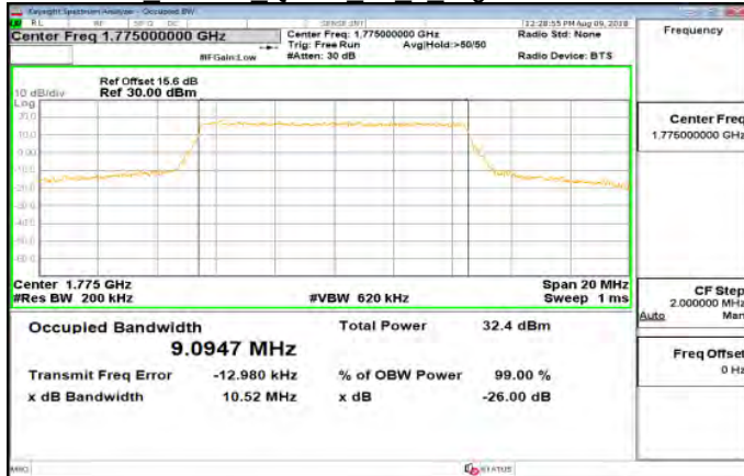
Band66 10MHz QPSK 50 0 HighCH132622-1775
