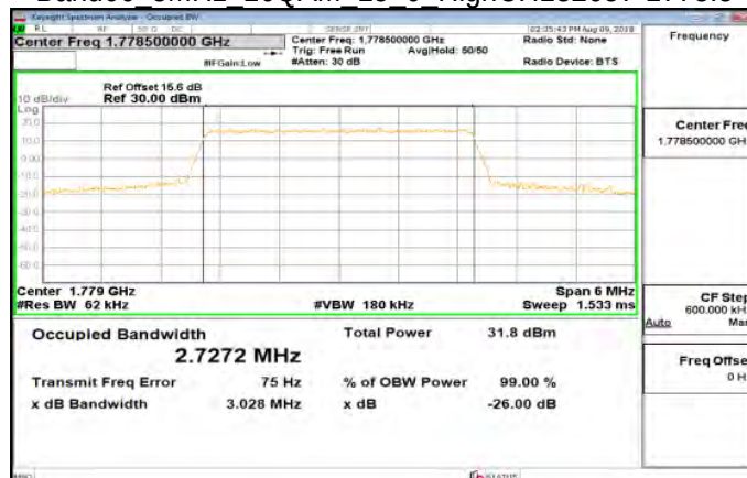
Band66 3MHz 16QAM 15 0 HighCH132657-1778.5
