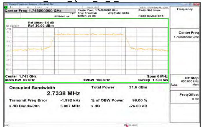
Band66 3MHz QPSK 15 0 MidCH132322-1745
