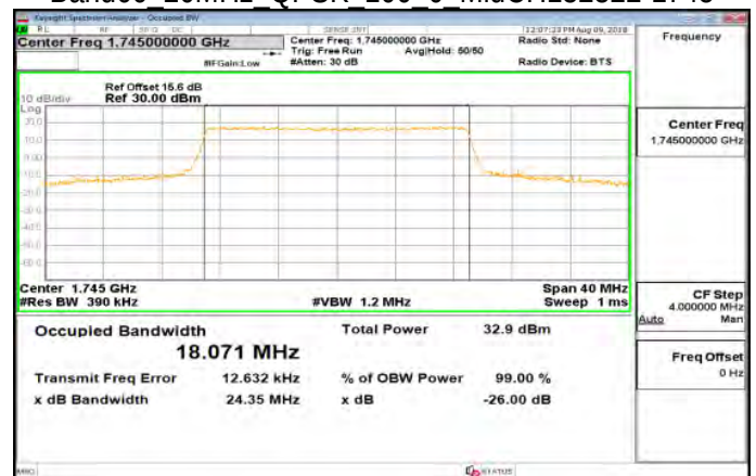
Band66 20MHz QPSK 100 0 MidCH132322-1745
