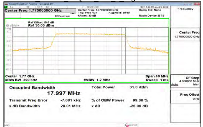
Band66 20MHz 16QAM 100 0 HighCH132572-1770
