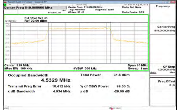
Part 90 Band26 5MHz QPSK 25 0 MidCH26740-819
