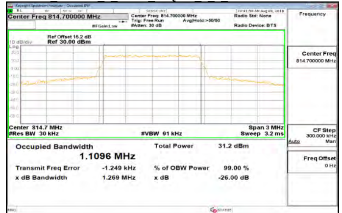
Part 90 Band26 1 4MHz 16QAM 6 0 LowCH26697-814.7
