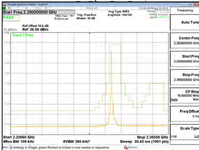
Band 30 5M QPSK LOW RB1,24
