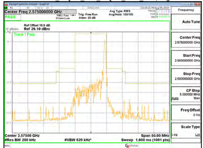
Band 38 16QAM 10M 16QAM LOW RB50,0.gif
