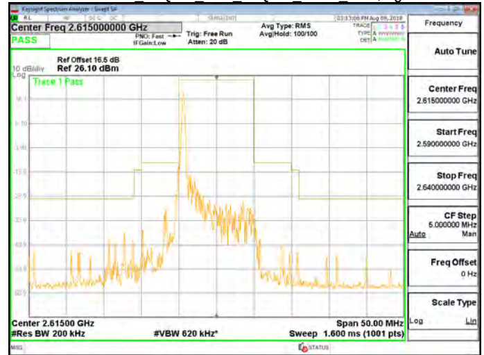
Band 38 16QAM 10M 16QAM HIGH RB1,49.gif
