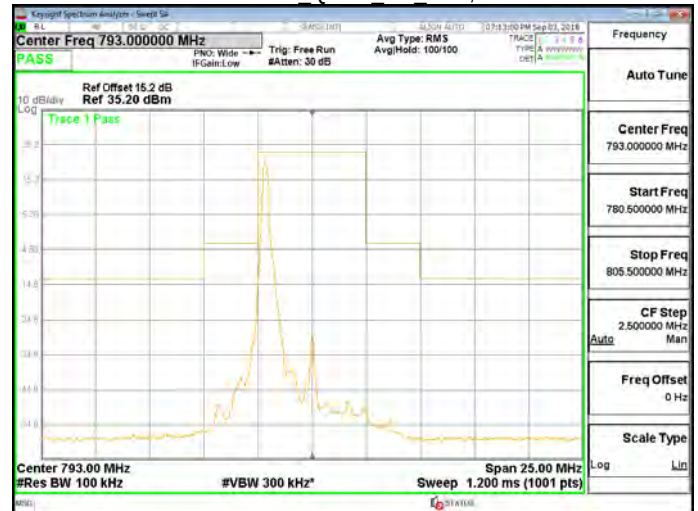
Band 14 QPSK 5M RB1,24
