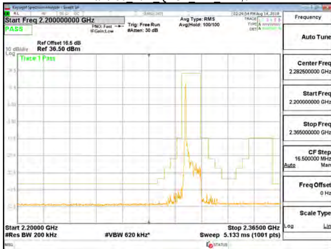
Band 30 10M QPSK MID RB1,49
