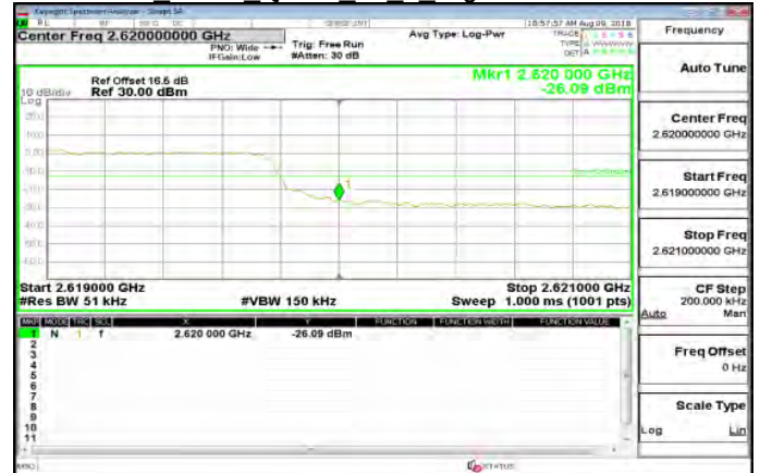
Band38 5MHz QPSK 25 0 HighCH38225-2617.5
