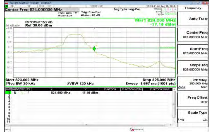
Part 90 Band26 3MHz QPSK 1 14 HighCH26775-822.5
