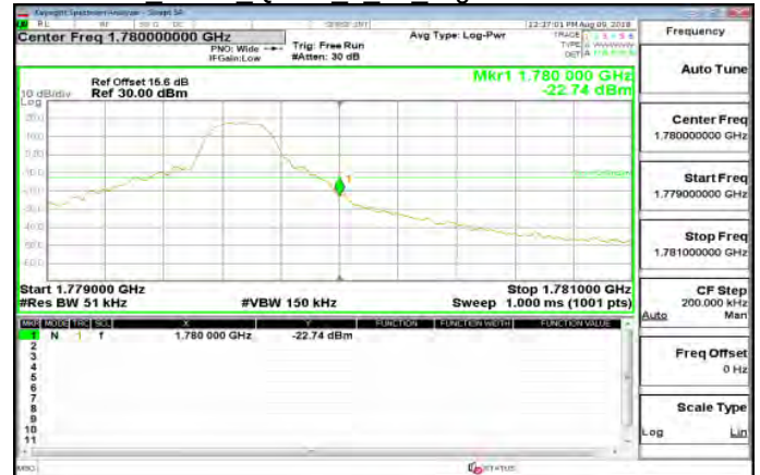
Band66 5MHz QPSK 1 24 HighCH132647-1777.5
