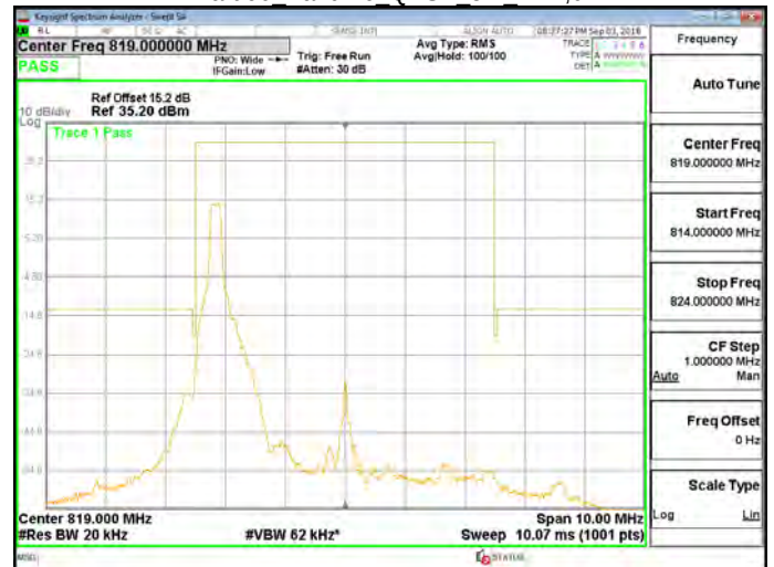
Part 90 Band 26 QPSK 5M RB1,24
