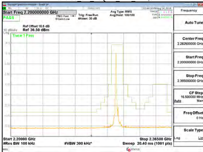
Band 30 5M 16QAM MID RB1,24
