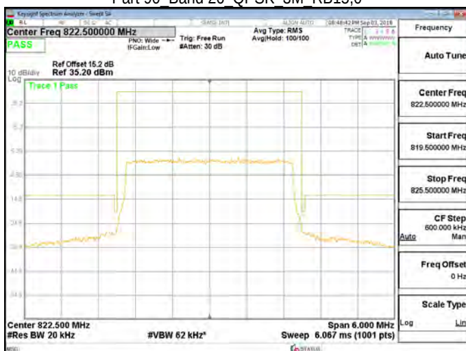
Part 90 Band 26 QPSK 3M RB15,0
