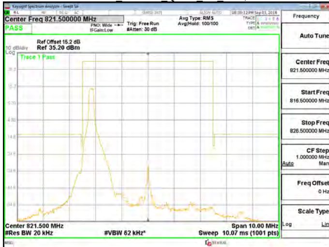
Part 90 Band 26 QPSK 5M RB1,24
