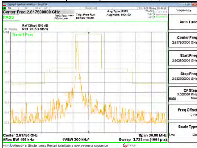
Band 38 QPSK 5M QPSK HIGH RB1,24.gif
