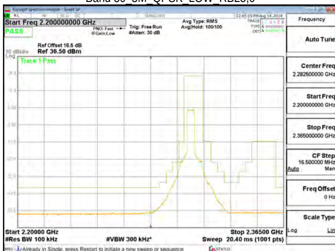
Band 30 5M QPSK LOW RB25,0
