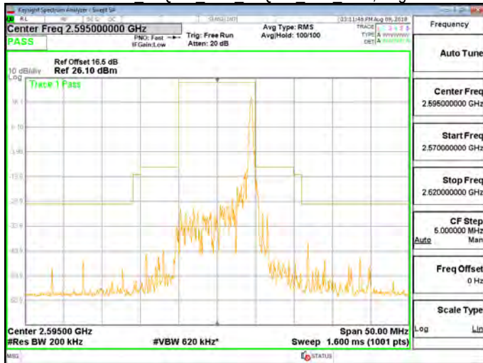
Band 38 16QAM 10M 16QAM MID RB50,0.gif
