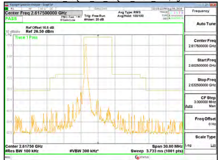
Band 38 16QAM 5M 16QAM HIGH RB1,24.gif
