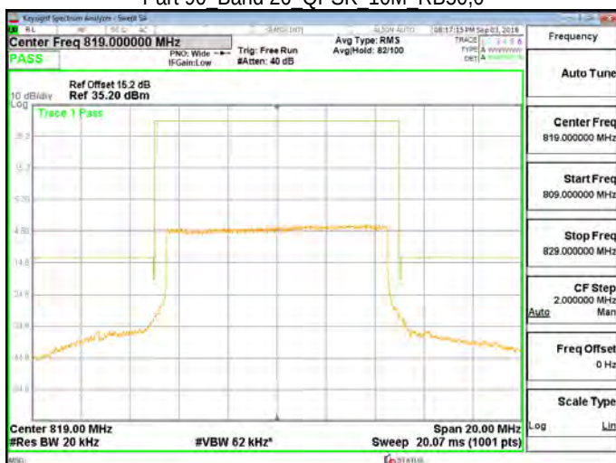
Part 90 Band 26 QPSK 10M RB50,0
