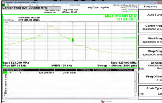
Band26 5MHz QPSK 1 24 HighCH26765-821.5
