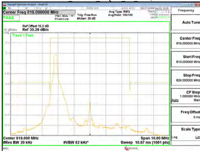
Part 90 Band 26 16QAM 5M RB1,24
