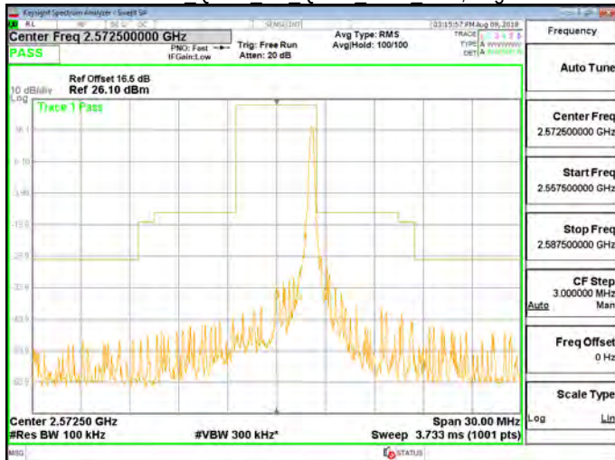
Band 38 QPSK 5M QPSK LOW RB25,0.gif
