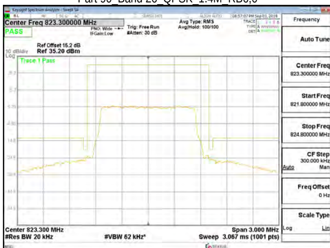
Part 90 Band 26 QPSK 1.4M RB6,0
