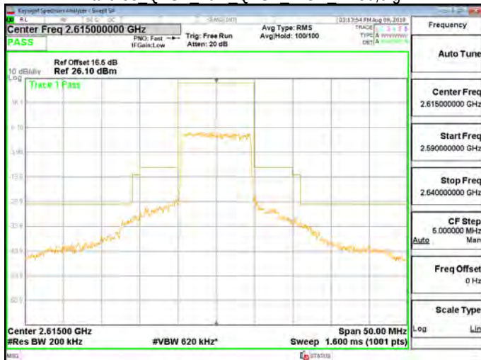
Band 38 QPSK 10M QPSK HIGH RB50,0.gif
