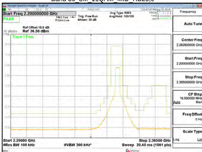
Band 30 5M 16QAM MID RB25,0
