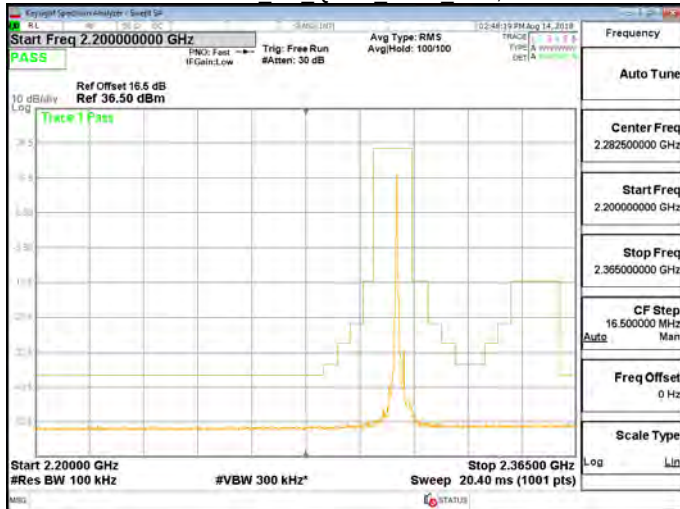
Band 30 5M QPSK HIGH RB1,24
