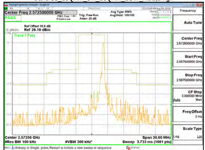
Band 38 16QAM 5M 16QAM LOW RB25,0.gif
