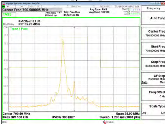
Band 14 QPSK 5M RB1,24
