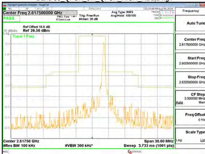
Band 38 QPSK 5M QPSK HIGH RB25,0.gif
