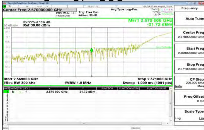
Band38 20MHz QPSK 1 0 LowCH37850-2580
