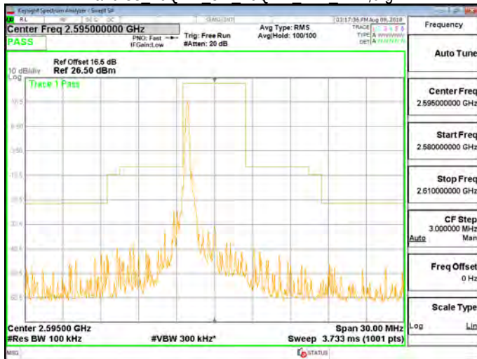
Band 38 16QAM 5M 16QAM MID RB1,24.gif
