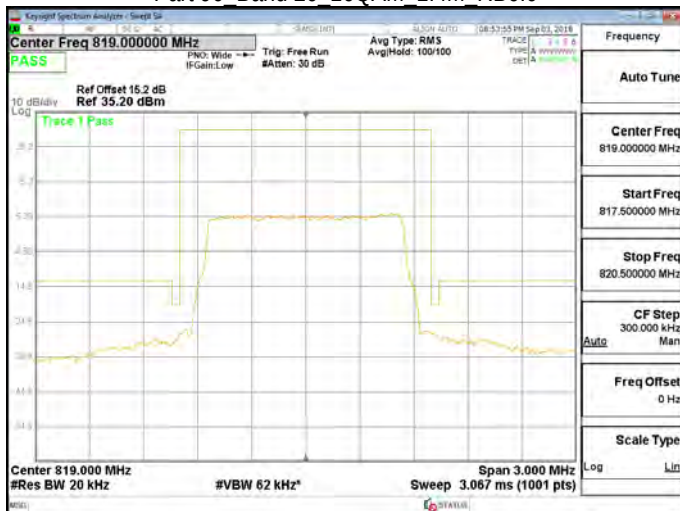
Part 90 Band 26 16QAM 1.4M RB6,0
