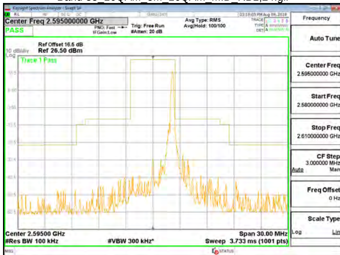
Band 38 16QAM 5M 16QAM MID RB25,0.gif
