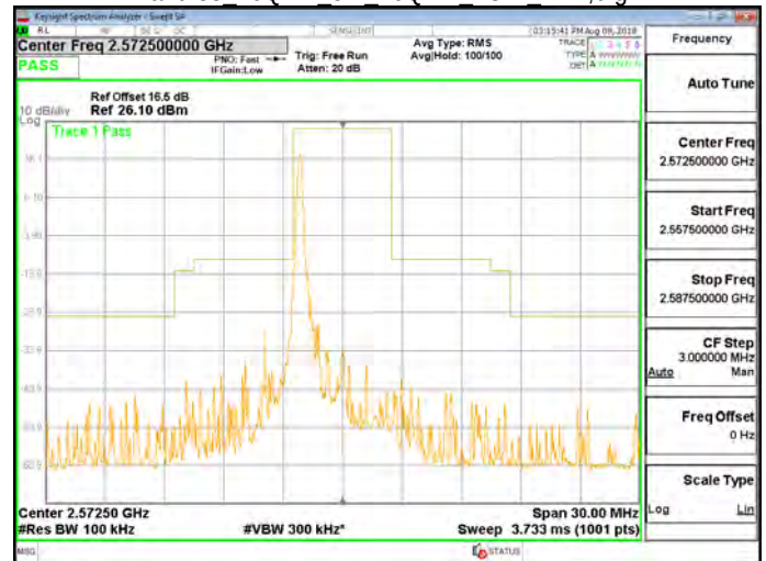
Band 38 16QAM 5M 16QAM LOW RB1,24.gif
