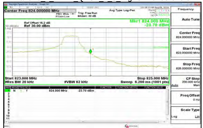
Band26 1 4MHz QPSK 1 5 HighCH26783-823.3
