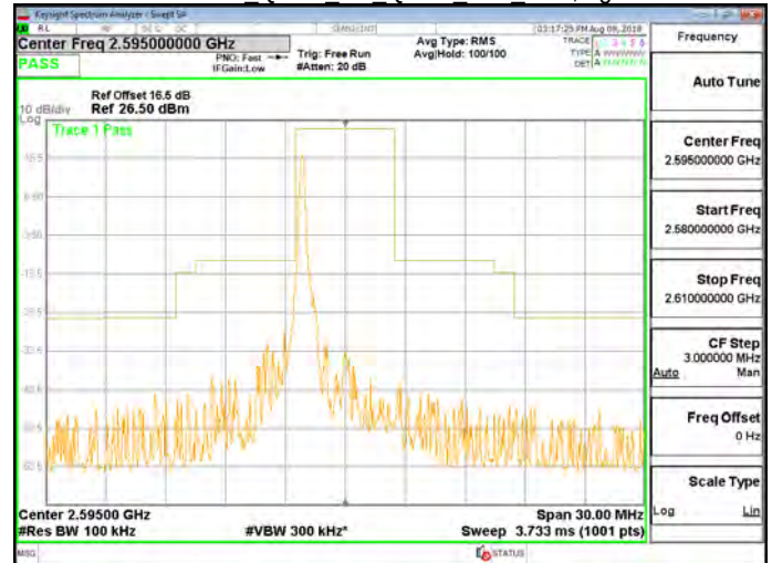
Band 38 QPSK 5M QPSK MID RB1,24.gif
