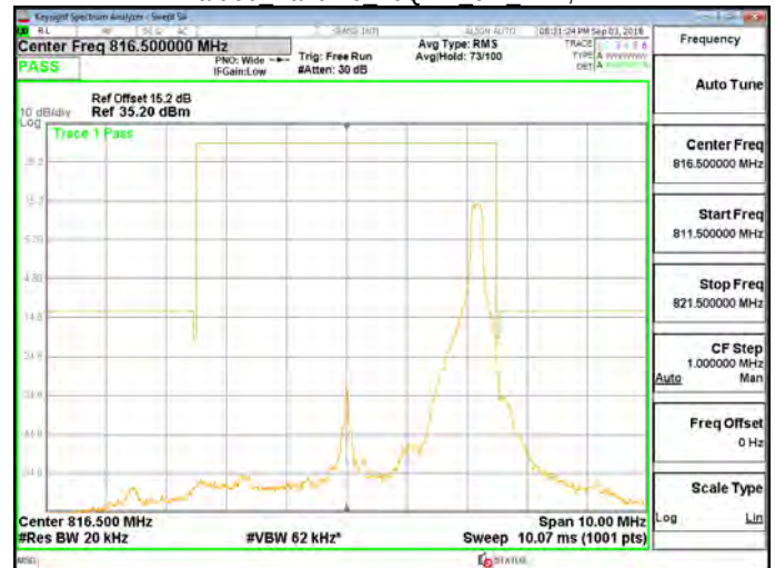
Part 90 Band 26 16QAM 5M RB25,0
