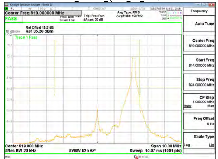
Part 90 Band 26 QPSK 5M RB25,0
