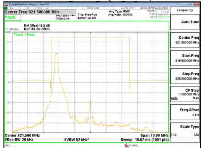
Part 90 Band 26 16QAM 5M RB1,24
