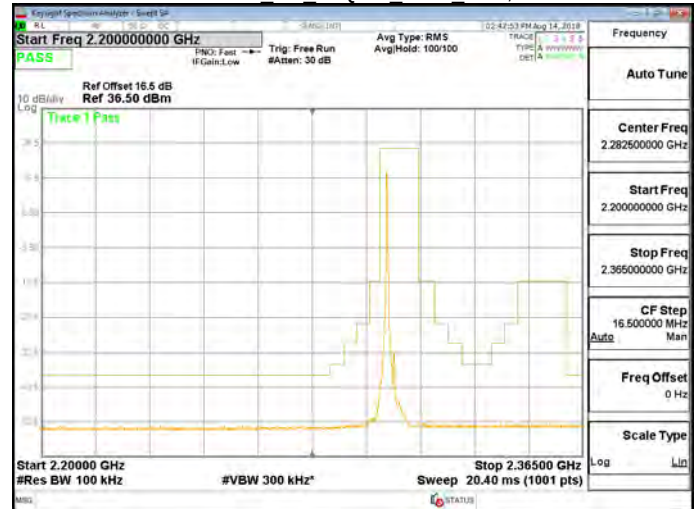
Band 30 5M 16QAM LOW RB1,24
