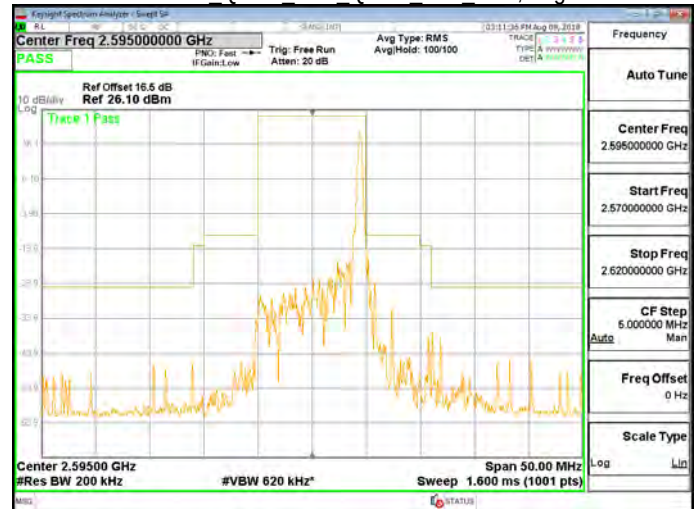
Band 38 QPSK 10M QPSK MID RB50,0.gif
