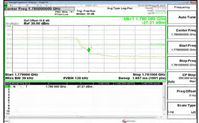
Band66 3MHz QPSK 15 0 HighCH132657-1778.5
