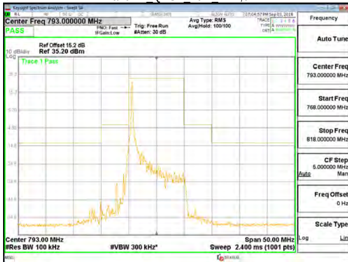
Band 14 QPSK 10M RB1,49
