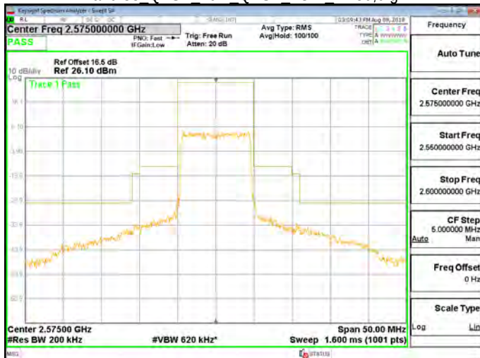
Band 38 QPSK 10M QPSK LOW RB50,0.gif
