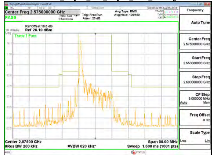
Band 38 16QAM 10M 16QAM LOW RB1,49.gif
