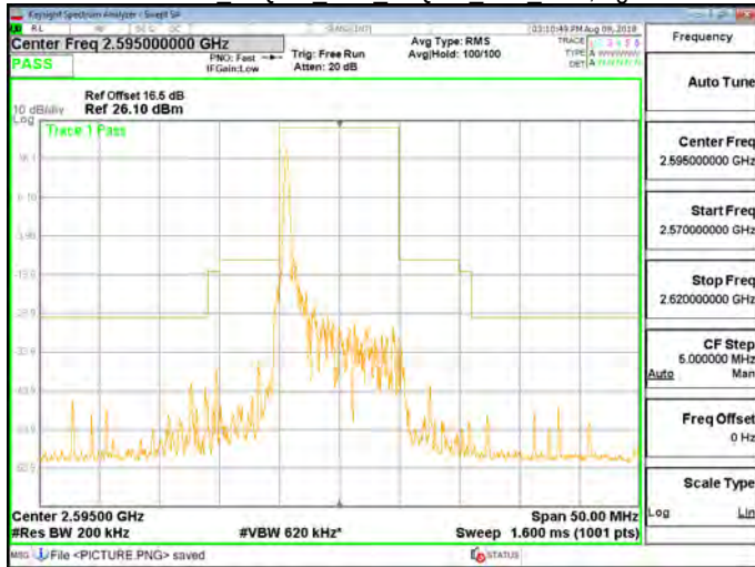
Band 38 16QAM 10M 16QAM MID RB1,49.gif
