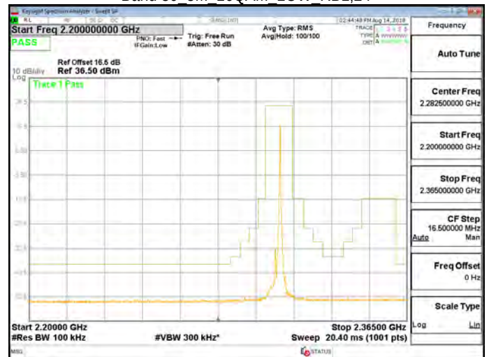
Band 30 5M 16QAM LOW RB25,0
