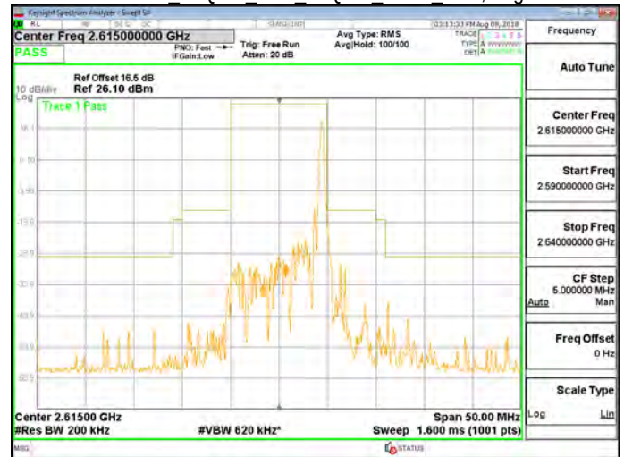
Band 38 16QAM 10M 16QAM HIGH RB50,0.gif
