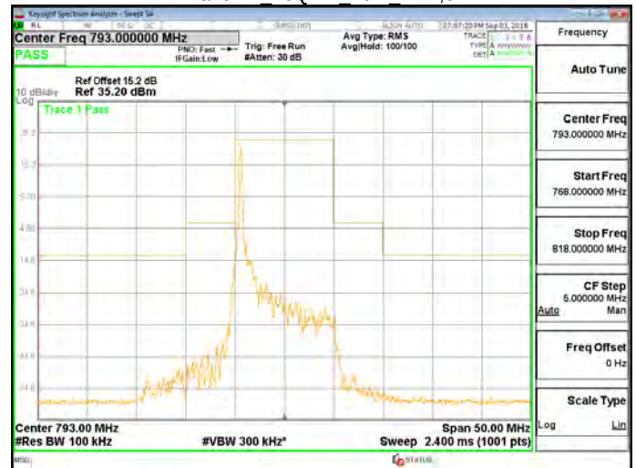
Band 14 16QAM 10M RB1,49
