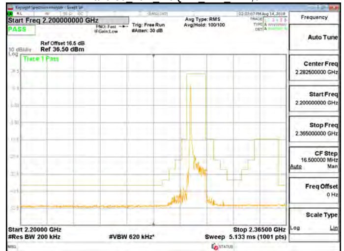
Band 30 10M 16QAM MID RB1,49
