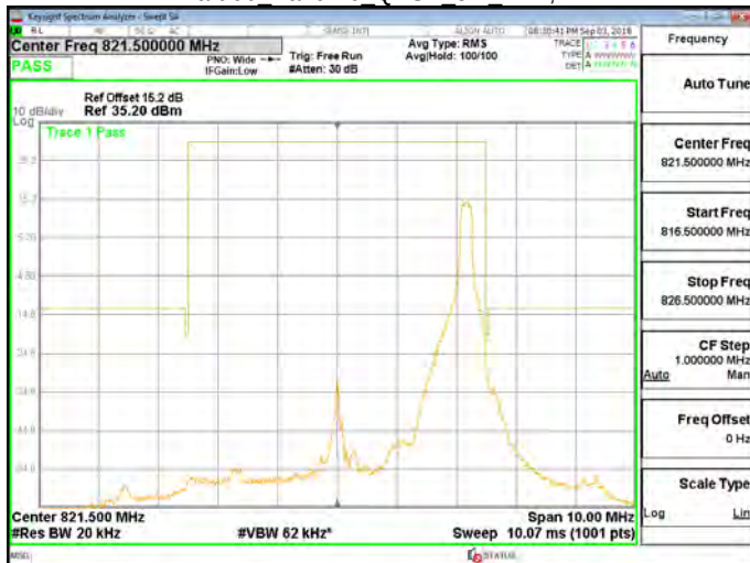
Part 90 Band 26 QPSK 5M RB25,0
