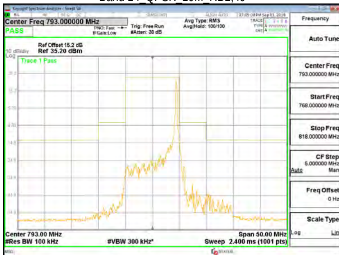
Band 14 QPSK 10M RB50,0
