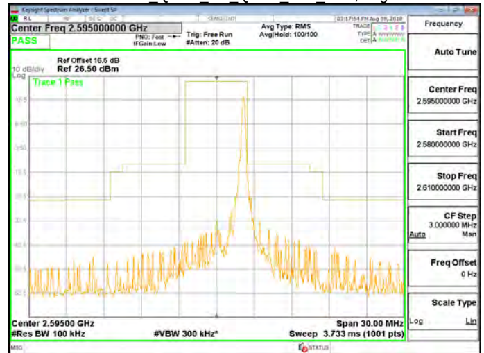
Band 38 QPSK 5M QPSK MID RB25,0.gif
