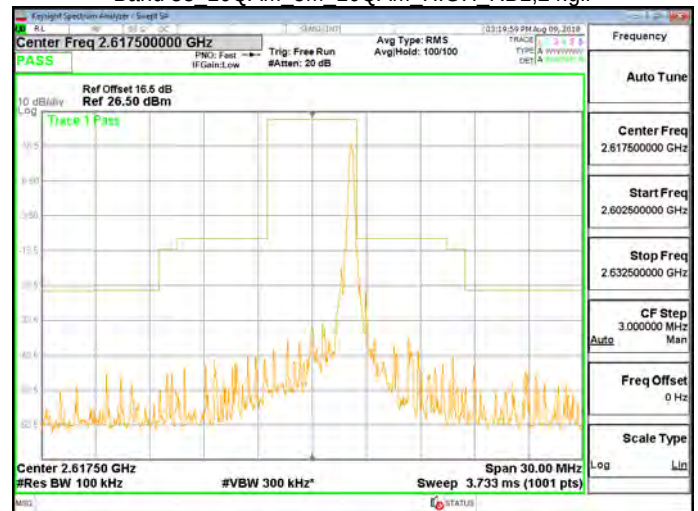
Band 38 16QAM 5M 16QAM HIGH RB25,0.gif
