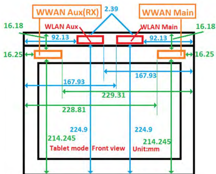
Fig.12 Antenna location (front view of tablet mode)
