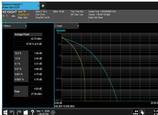
N25(10M)_DFT-s-OFDM_PI_2- BPSK_Outer_Full_Low_CH
