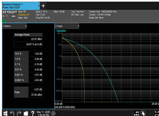
N25(5M)_DFT-s-OFDM_PI_2- BPSK_Outer_Full_Mid_CH
