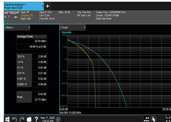
N25(10M)_DFT-s- OFDM_QPSK_Outer_Full_Low_CH
