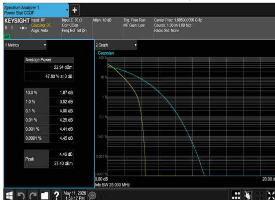
N25(20M)_DFT-s-OFDM_PI_2- BPSK_Outer_Full_High_CH
