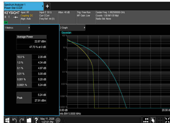
N25(5M)_DFT-s- OFDM_QPSK_Outer_Full_Mid_CH
