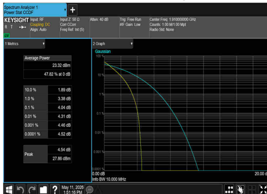
N25(10M)_DFT-s-OFDM_PI_2- BPSK_Outer_Full_High_CH
