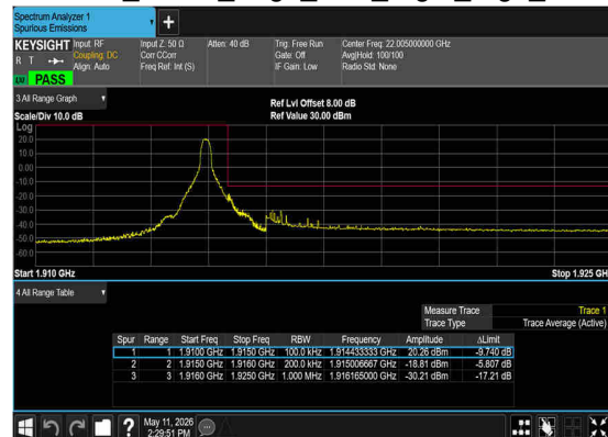
N25(20M)_DFT-s-OFDM_QPSK_Edge_1RB_Right_High_CH
