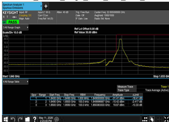
N25(10M)_DFT-s-OFDM_QPSK_Edge_1RB_Left_Low_CH
