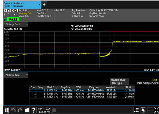
N25(10M)_DFT-s-OFDM_QPSK_Outer_Full_Low_CH
