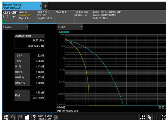
N26(10M)_DFT-s-OFDM_PI_2- BPSK_Outer_Full_High_CH
