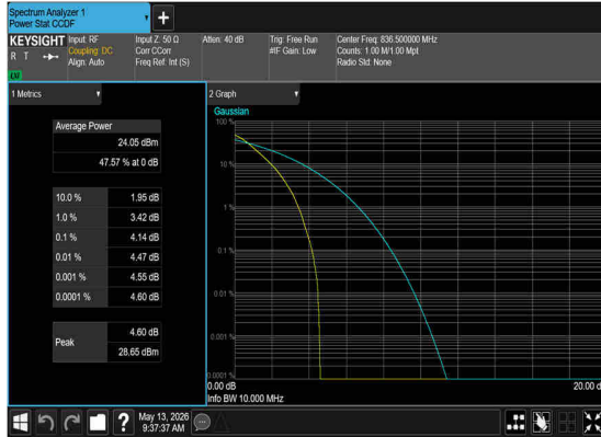
N26(10M)_DFT-s-OFDM_PI_2- BPSK_Outer_Full_Mid_CH
