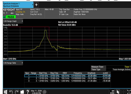
N25(10M)_DFT-s-OFDM_QPSK_Edge_1RB_Right_High_CH
