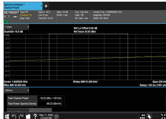
N25(10M)_DFT-s-OFDM_QPSK_Edge_1RB_Left_Low_CH_CHP_PA SS
