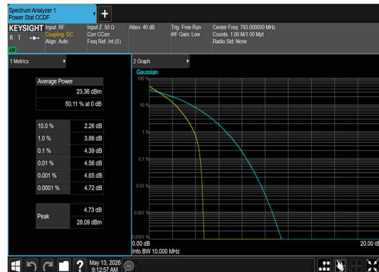
N14(10M)_DFT-s- OFDM_QPSK_Outer_Full_Mid_CH
