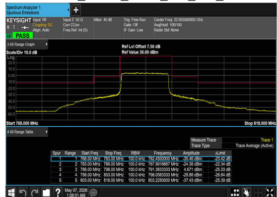
N14(10M)_DFT-s- OFDM_QPSK_Outer_Full_Mid_CH
