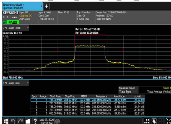
N14(10M)_DFT-s- OFDM_BPSK_Outer_Full_Mid_CH
