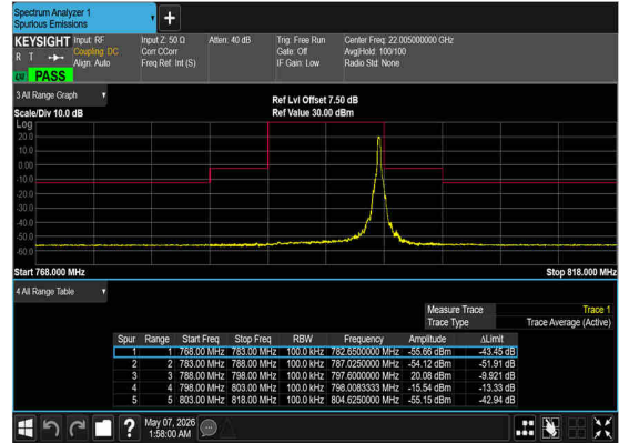
N14(10M)_DFT-s- OFDM_QPSK_Edge_1RB_Right_Mid_CH
