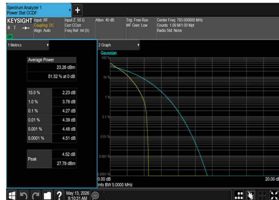
N14(5M)_DFT-s- OFDM_QPSK_Outer_Full_Mid_CH
