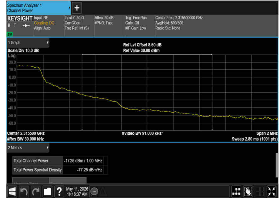
N30(10M)_DFT-s- OFDM_BPSK_Edge_1RB_Right_Low_CH_CHP_PASS
