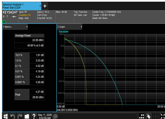
N30(5M)_DFT-s-OFDM_PI_2- BPSK_Outer_Full_Mid_CH
