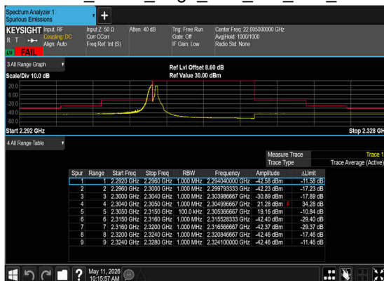
N30(10M)_DFT-s- OFDM_QPSK_Edge_1RB_Left_Low_CH
