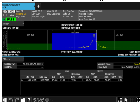
N48(15M)_DFT-s-OFDM_QPSK_Edge_1RB_Right_Mid_CH
