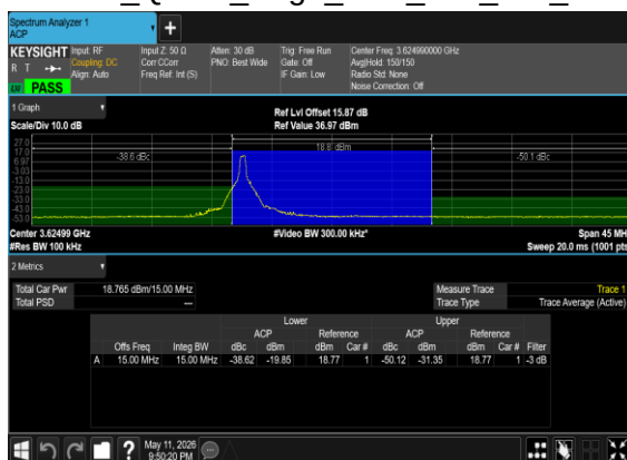
N48(15M)_DFT-s-OFDM_QPSK_Edge_1RB_Left_Mid_CH
