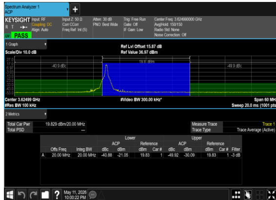
N48(20M)_DFT-s-OFDM_PI_2-BPSK_Edge_1RB_Left_Mid_CH
