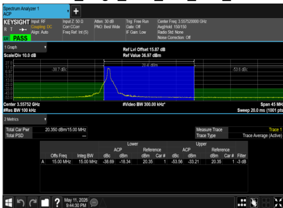
N48(15M)_DFT-s-OFDM_PI_2-BPSK_Edge_1RB_Left_Low_CH
