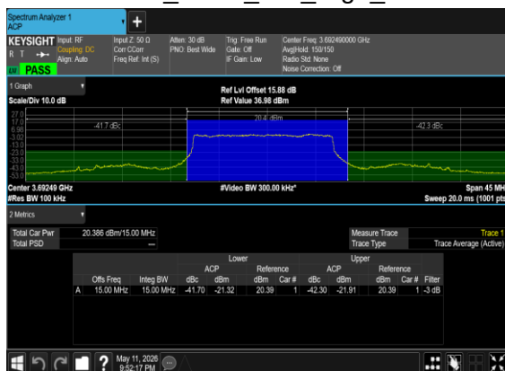
N48(15M)_DFT-s-OFDM_PI_2-BPSK_Outer_Full_High_CH
