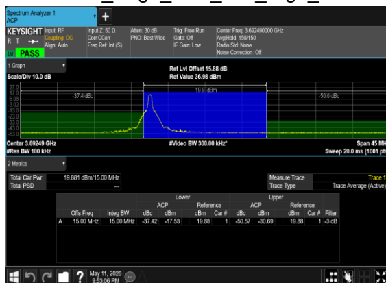
N48(15M)_DFT-s-OFDM_PI_2-BPSK_Edge_1RB_Left_High_CH
