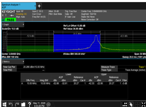
N48(10M)_DFT-s-OFDM_QPSK_Edge_1RB_Right_High_CH
