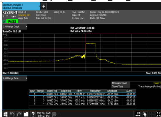
N77(15M)_DFT-s- OFDM_QPSK_Outer_Full_Low_CH
