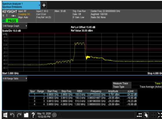
N77(15M)_DFT-s- OFDM_QPSK_Outer_Full_High_CH
