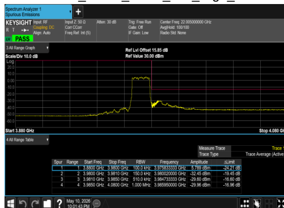
N77(15M)_DFT-s- OFDM_BPSK_Outer_Full_High_CH
