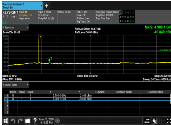
N77(15M)_DFT-s- OFDM_BPSK_Edge_1RB_Left_Low_CH
