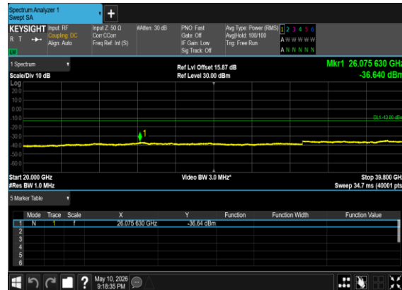
N77(15M)_DFT-s- OFDM_QPSK_Edge_1RB_Left_Low_CH
