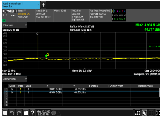
N77(15M)_DFT-s-OFDM_QPSK_Edge_1RB_Left_Mid_CH
