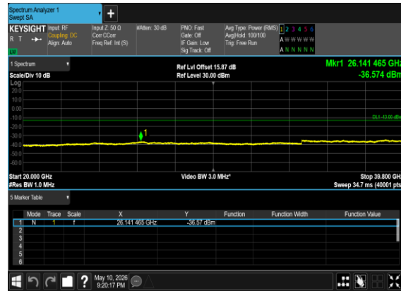
N77(15M)_DFT-s-OFDM_BPSK_Edge_1RB_Left_Mid_CH
