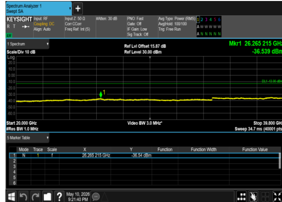
N77(15M)_DFT-s-OFDM_QPSK_Edge_1RB_Left_Mid_CH
