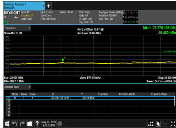
N77(15M)_DFT-s- OFDM_BPSK_Edge_1RB_Left_Low_CH
