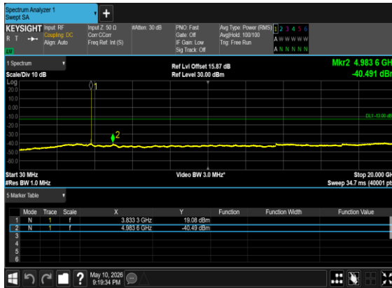
N77(15M)_DFT-s-OFDM_BPSK_Edge_1RB_Left_Mid_CH
