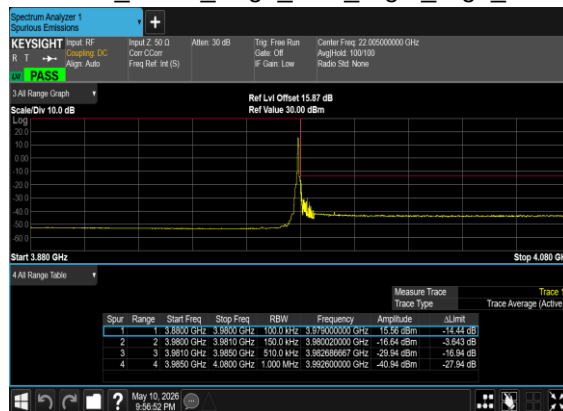
N77(15M)_DFT-s- OFDM_BPSK_Edge_1RB_Right_High_CH
