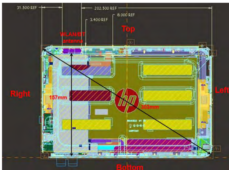
Fig.7 Antenna position (Back view)
